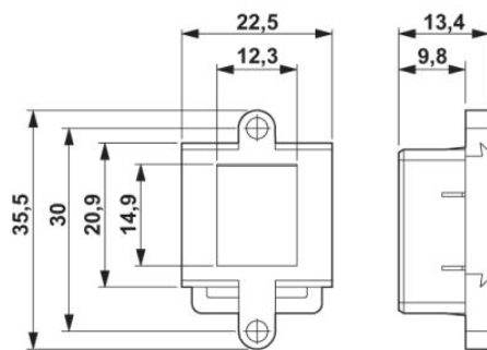
RJ45 panel mounting frame, IP20
