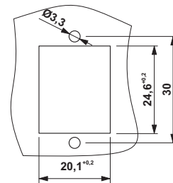
Dimensioned drawing
