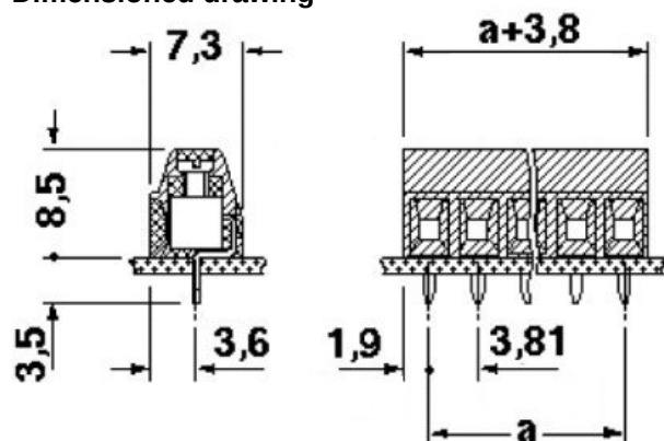
Dimensioned drawing
