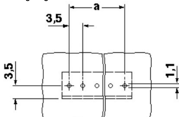
Drilling diagram
