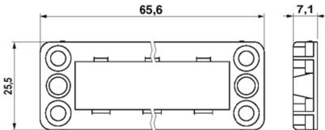
Dimensioned drawing
