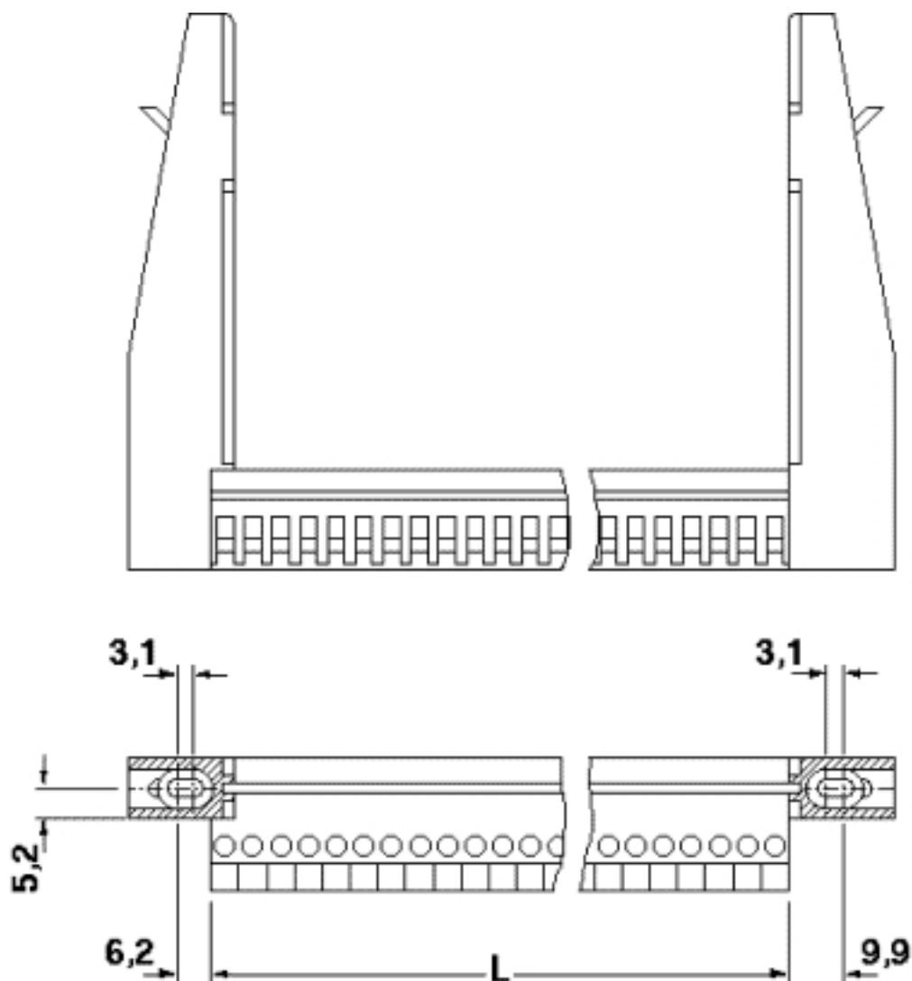
Dimensioned drawing
