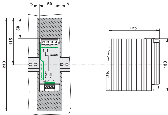
Figure 3 Installation dimensions
