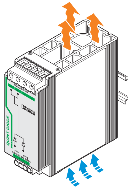
Figure 2 Convection
