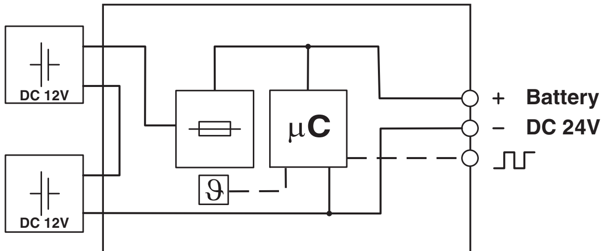
Block diagram
