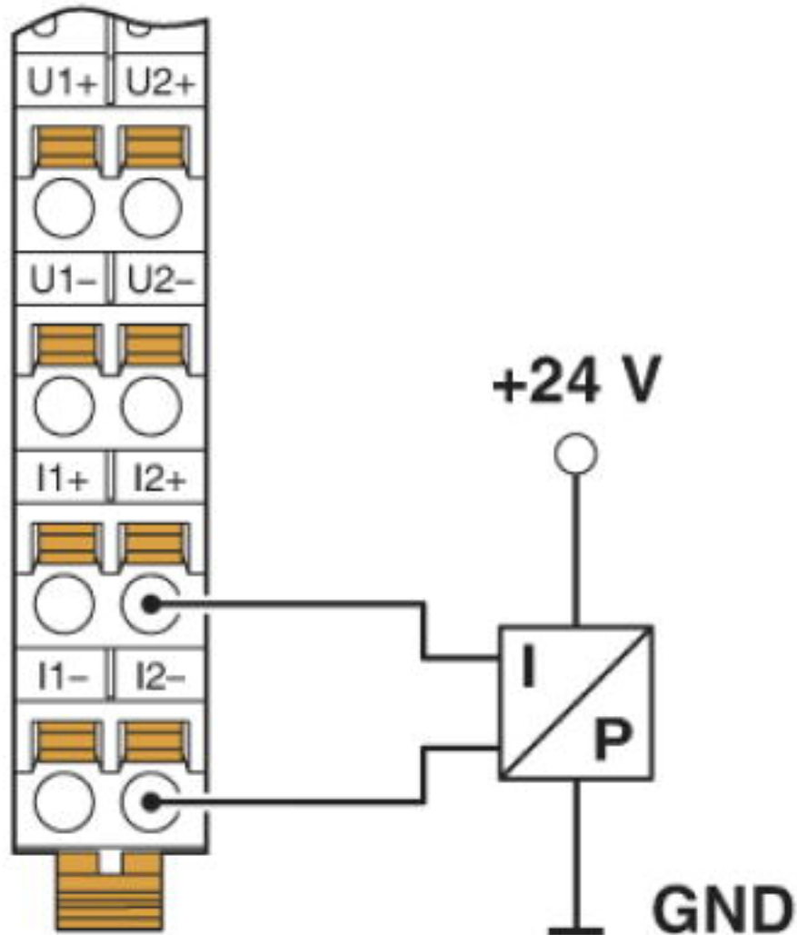
Connection diagram
