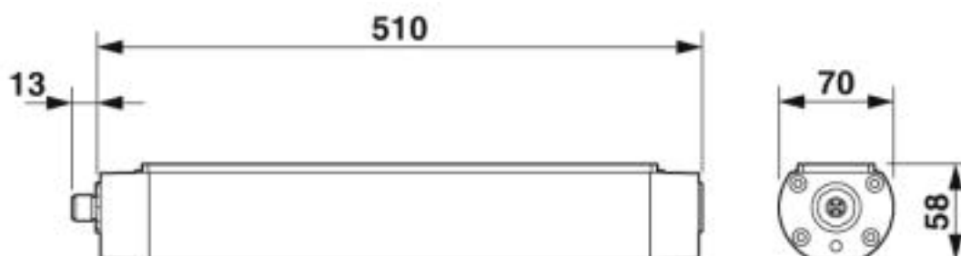
Dimensional drawing
