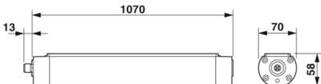
Dimensional drawing
