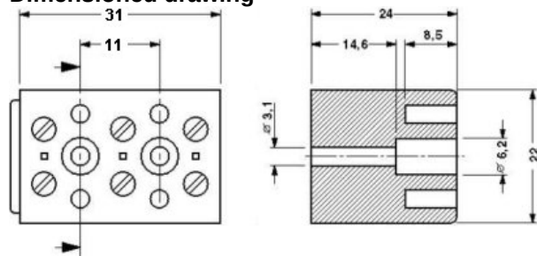
Dimensioned drawing
