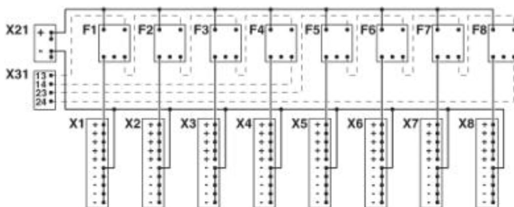
Circuit diagram
