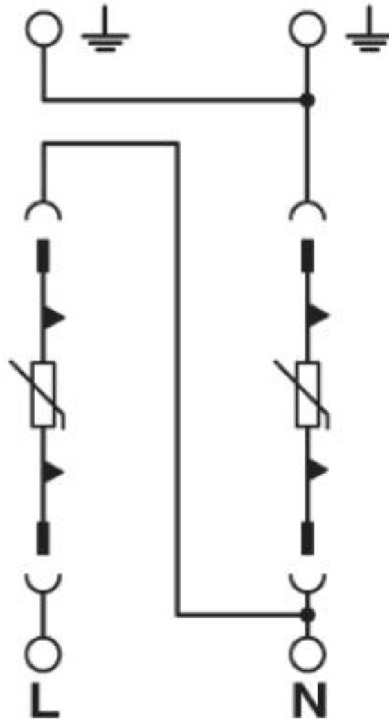
Circuit diagram
