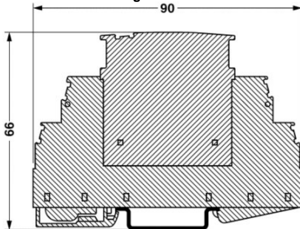
Dimensioned drawing
