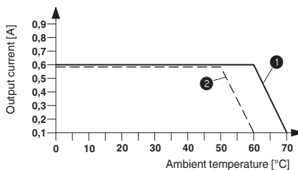
Derating curve ELR H5-IES-SC-230AC/500AC-0,6 100% operating time
