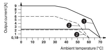
Derating curve ELR H5-ES-SC-230AC/500AC-2 and ELR H5-ES-SC-230AC/500AC-9 100% operating time
