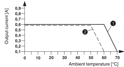
Derating curve ELR H5-ES-SC-230AC/500AC-0,6 100% operating time
