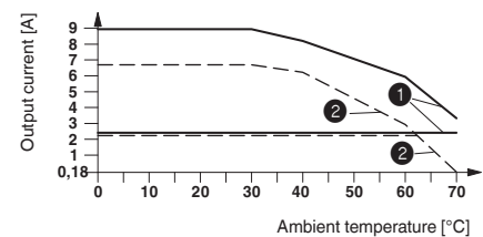
Derating curve ELR H3-ES-SC-24DC/500AC-2 and ELR H3-ES-SC-230AC/500AC-9 100% operating time
