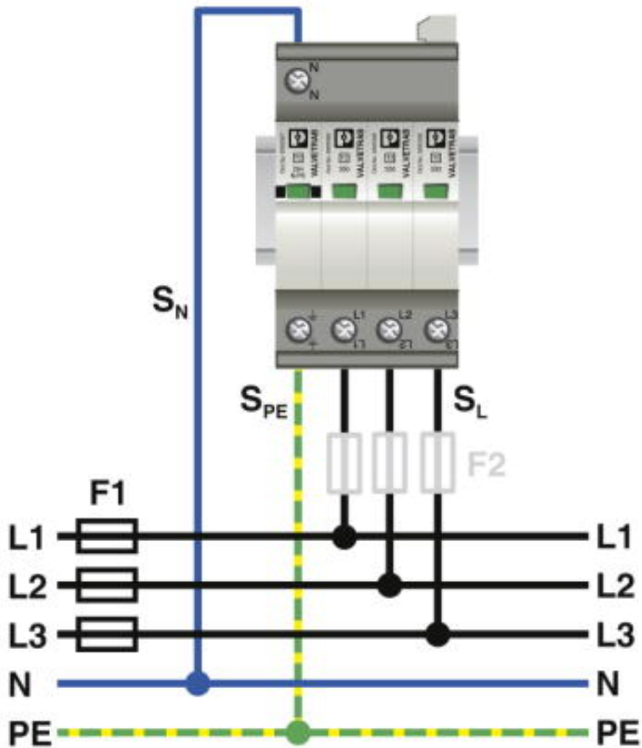
Figure shows version with remote indication contact
