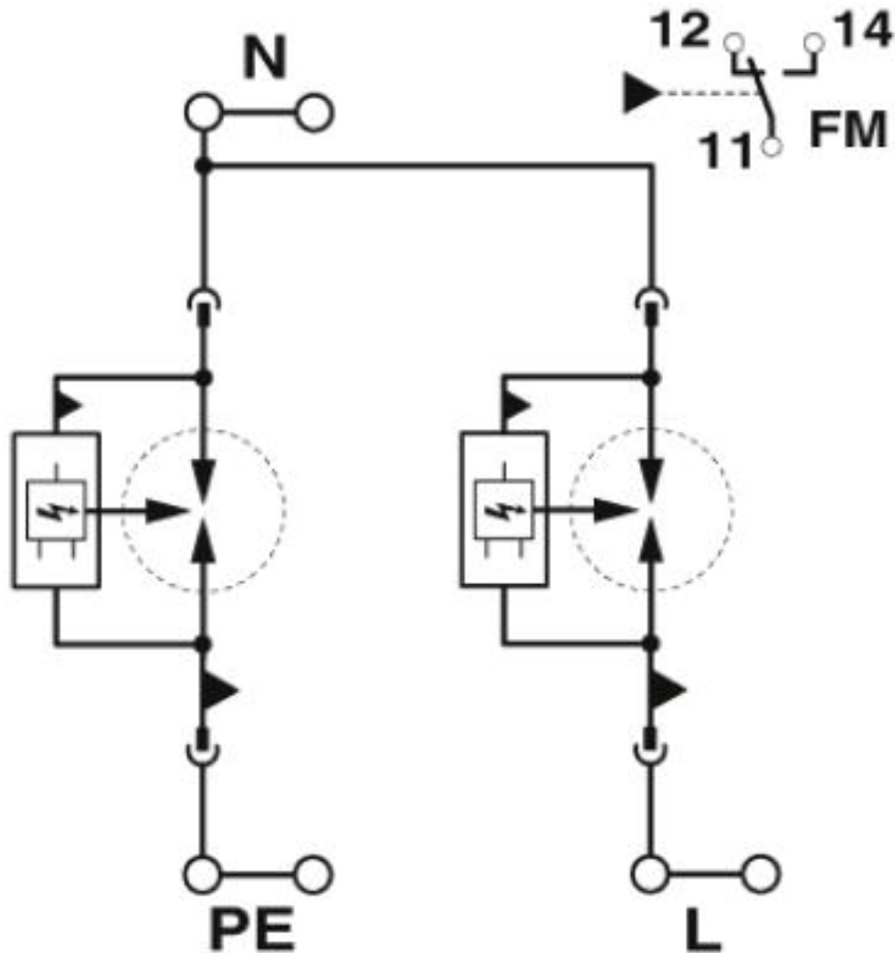
Circuit diagram
