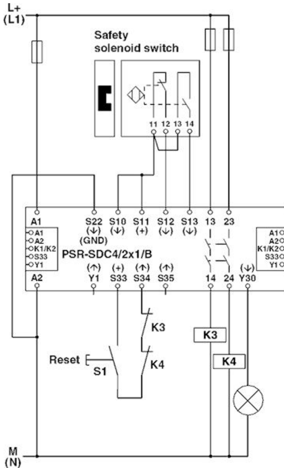
Circuit diagram
