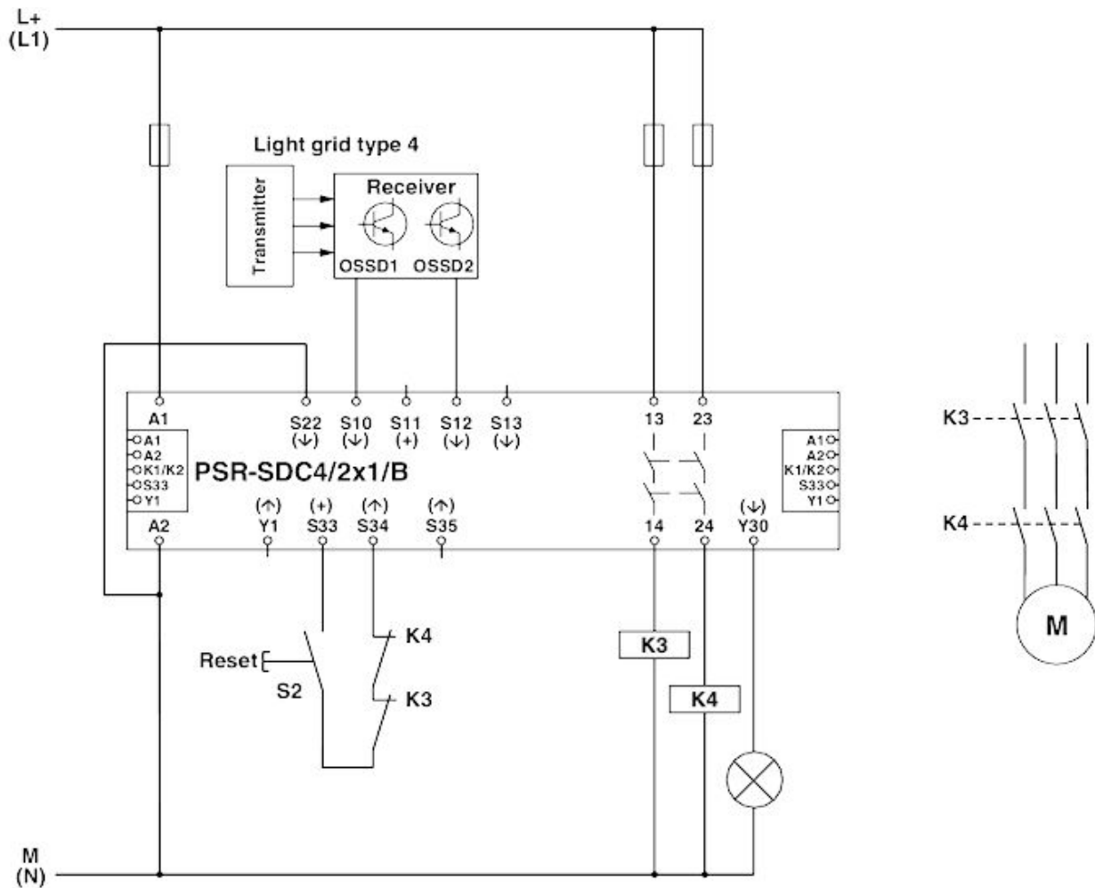
Circuit diagram
