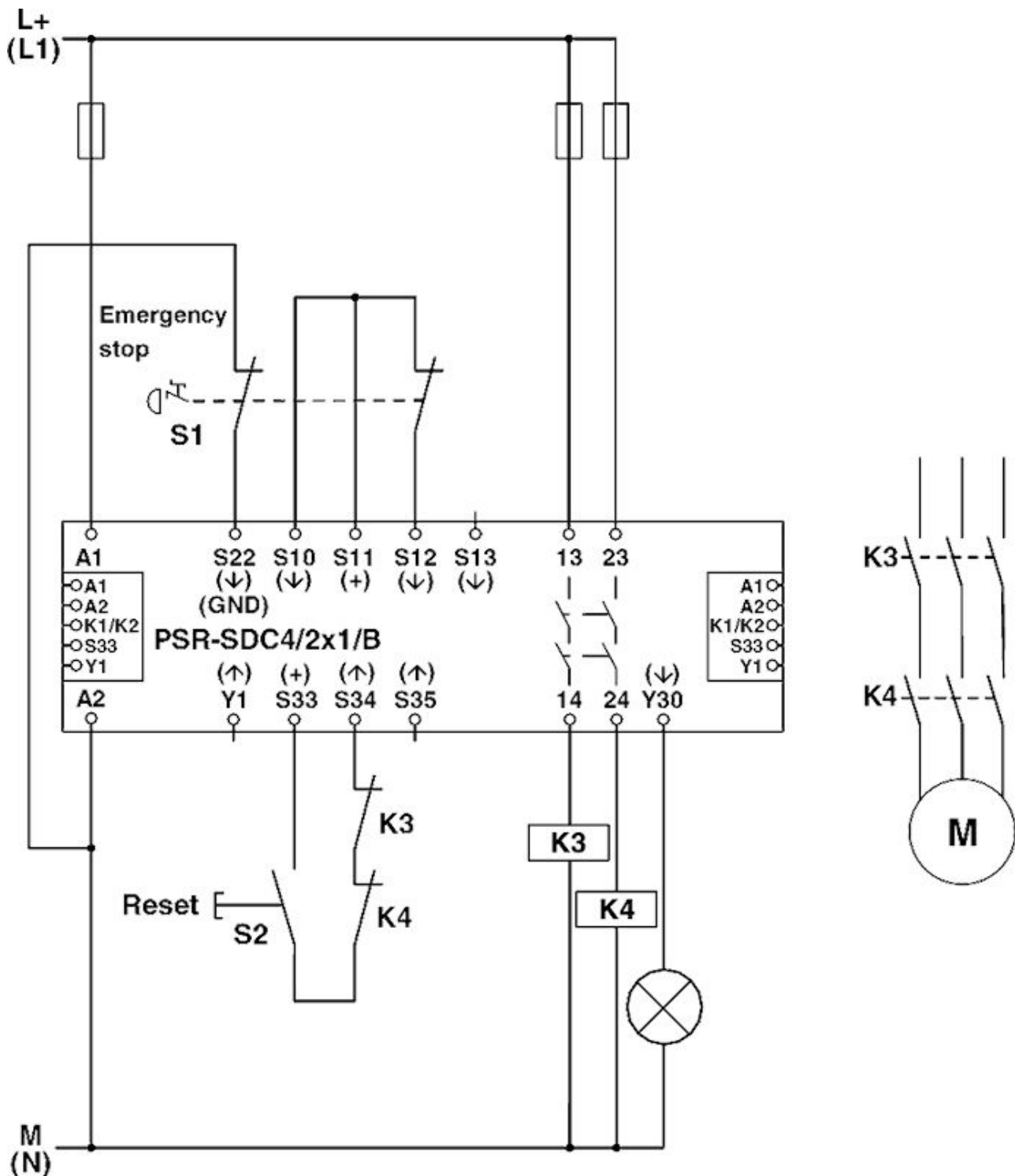
Circuit diagram
