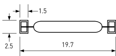
Pad sizes
