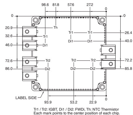
Tr1 / Tr2: IGBT, Di1 / Di2: FWDi, Th: NTC Thermistor Each mark points to the center position of each chip.
