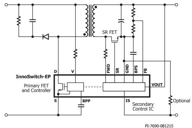
Figure 1. Typical Application/Performance.
