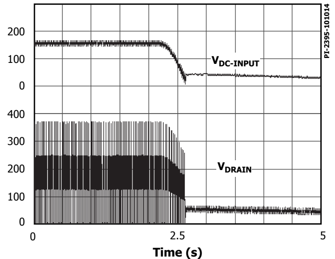
Figure 12. Normal Power-Down Timing.
