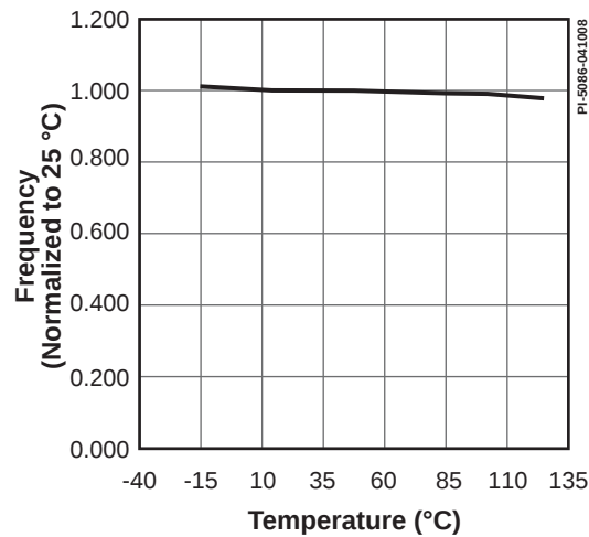
Figure 13. Output Frequency vs. Temperature.
