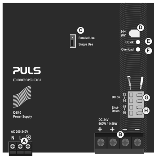
Fig. 14-1 Front side
