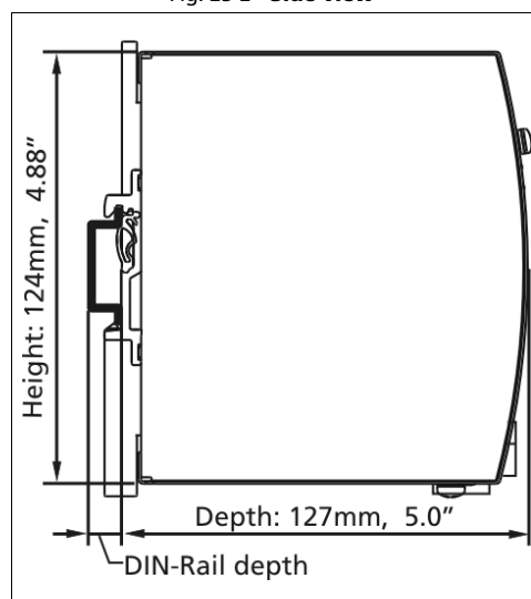
Fig. 23-2 Side view
