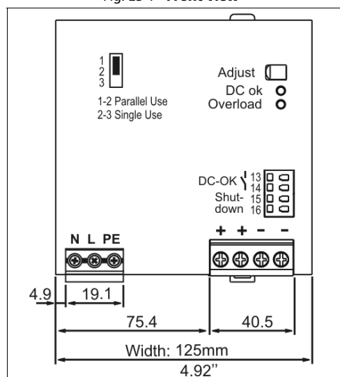
Fig. 23-1 Front view
