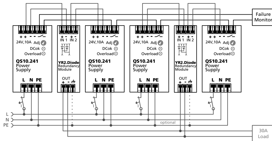
Fig. 19-2 Wiring diagram, n+1 Redundancy, 30A output current
