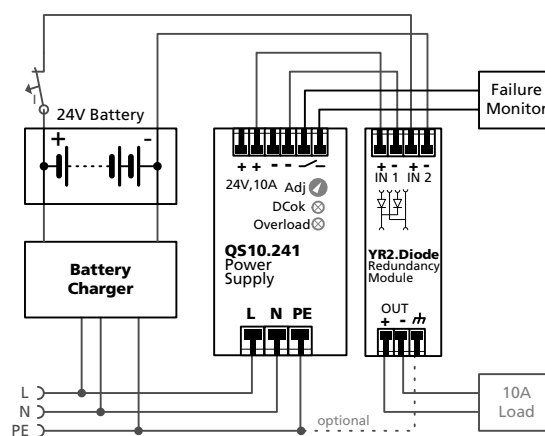
Fig. 19-3 Wiring diagram, 10A Battery back-up
