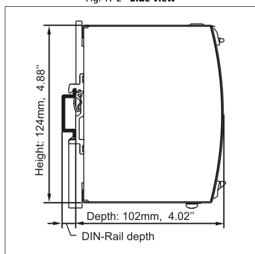
Fig. 17-2 Side view
