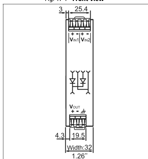
Fig. 17-1 Front view
