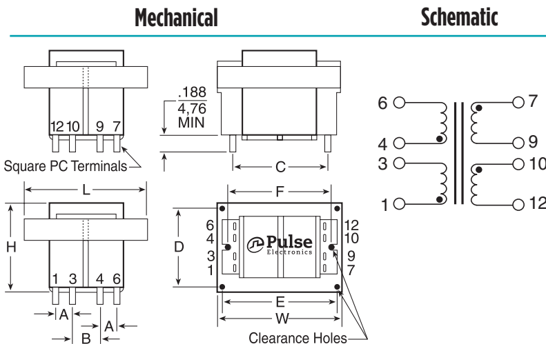
Dimensions (inches)
