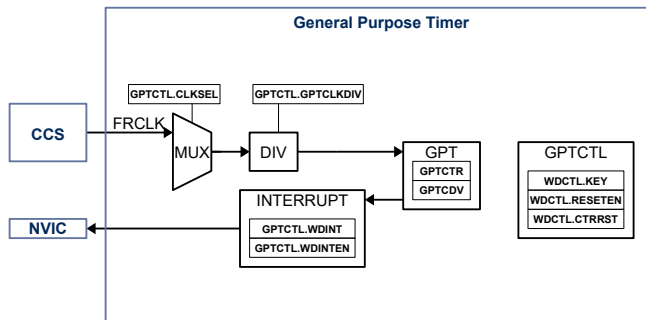
Figure 6-1. GPT
