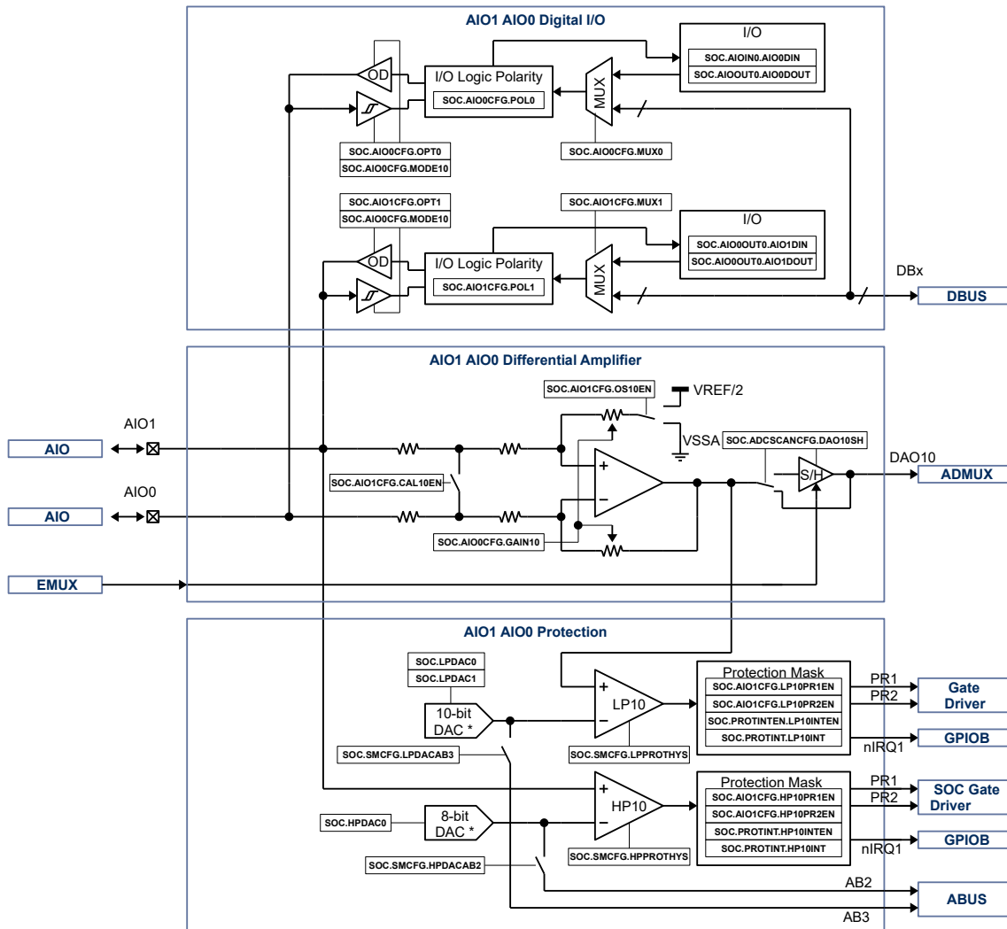
Figure 23-2. AIO1, AIO0
