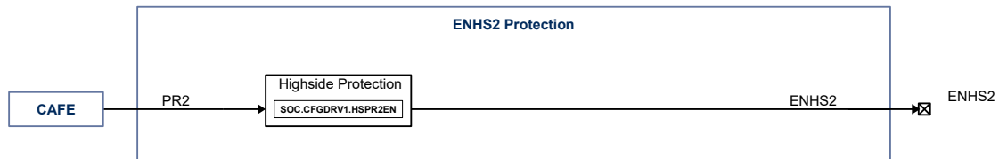
Figure 25-6. ENHS2 Protection
