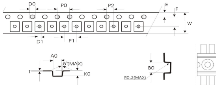
Tape Dimension
