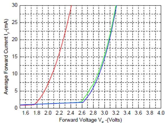
Figure2. Forward Current VS. Forward Voltage
