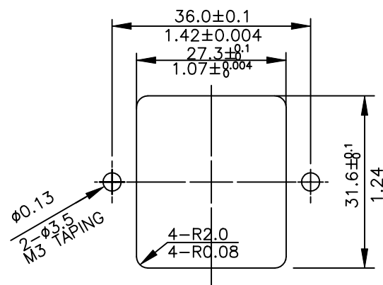
Panel Cutout
