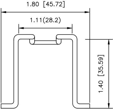
CLIP .072” Dia. Stainless Steel Wire
