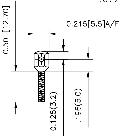
SCREW 6 BA Brass, Nickel Plated
