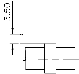
PCB Mounting
