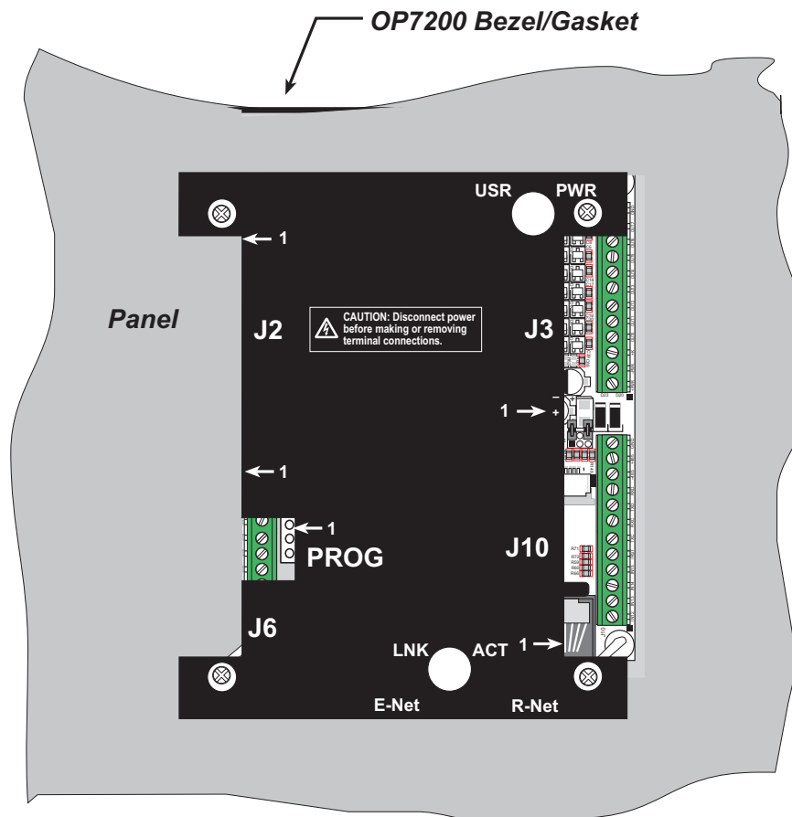
Figure 23. OP7200 Mounted in Panel (rear view)
