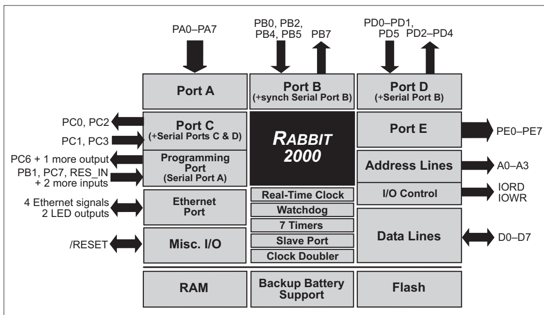
Figure A-5. OP7200 Rabbit-Based Subsystems
