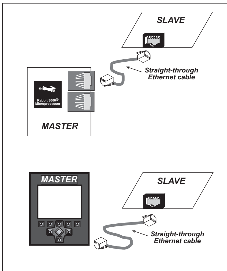
Figure D-1. Connecting Peripheral Boards to a Master
