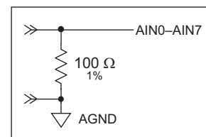
Figure 13. Resistor for 4–20 mA Current Sources
