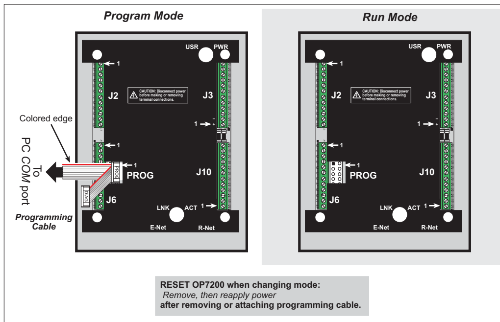
Figure 20. OP7200 Program Mode and Run Mode Set-Up
