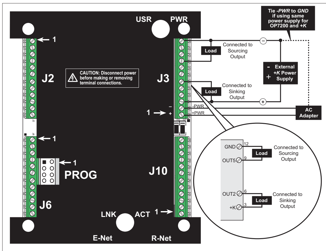
Figure 10. +K, Power Supply, and Sample Load Connections
