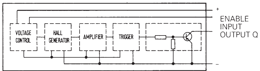
Static with Enable Input
