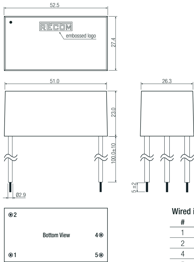
Dimension Drawing Single Wired (mm)
