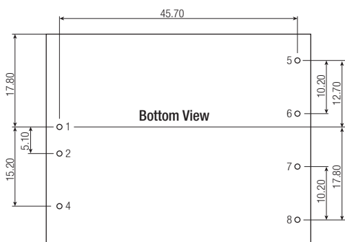
Dimension Drawing (mm) with Heat-sink
