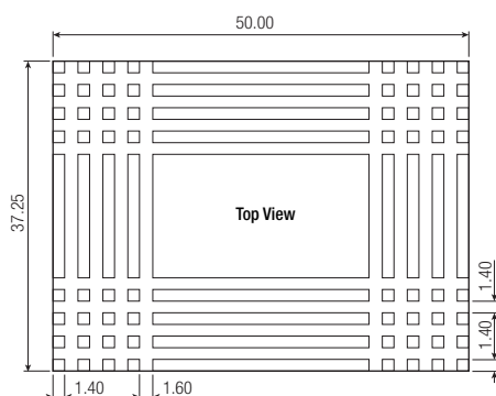
Dimension Drawing (mm) with Heat-sink
