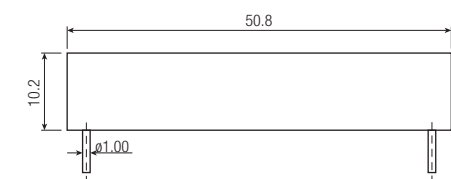
Dimension Drawing (mm)
