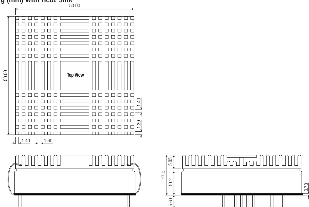
Dimension Drawing (mm) with Heat-sink
