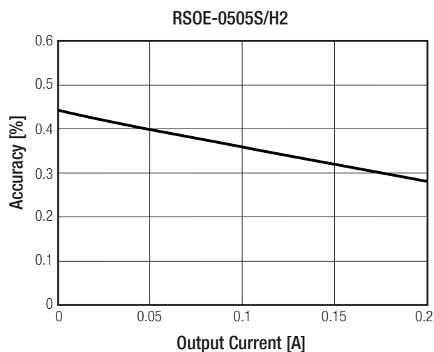
Accuracy vs. Load
