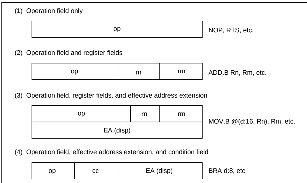
Figure 1.12 Instruction Formats
