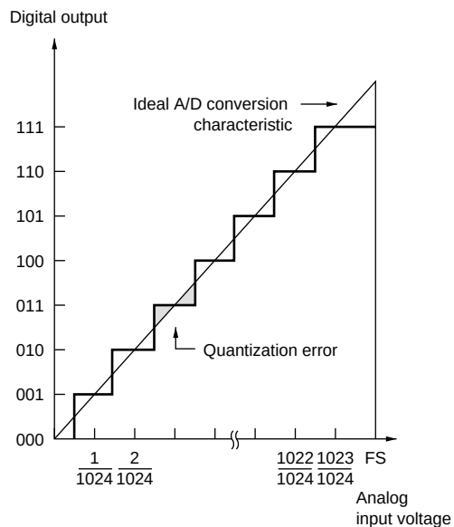
Figure 15.7 A/D Conversion Accuracy Definitions (1)
