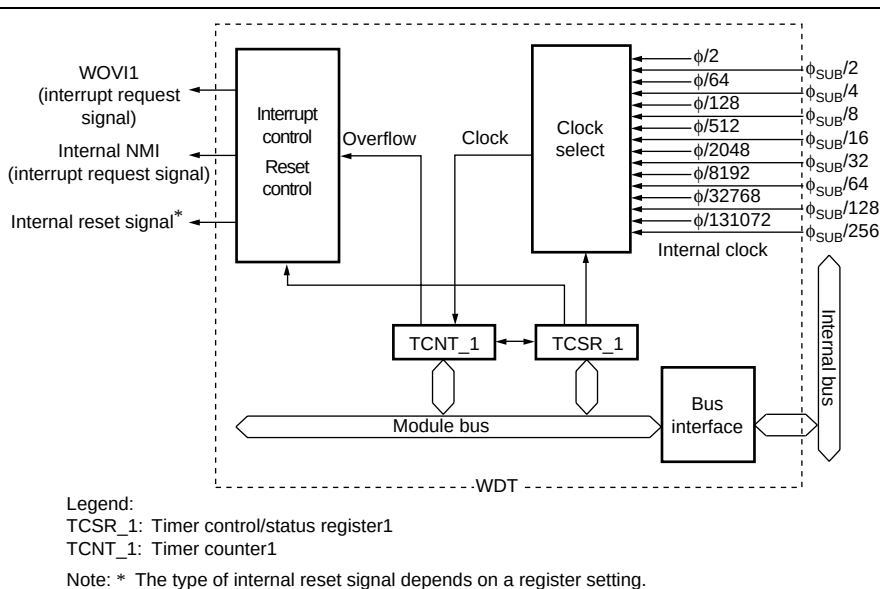
Figure 12.2 Block Diagram of WDT_1
