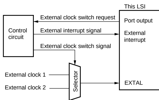
Figure 21.6 External Clock Switching Circuit (Examples)
