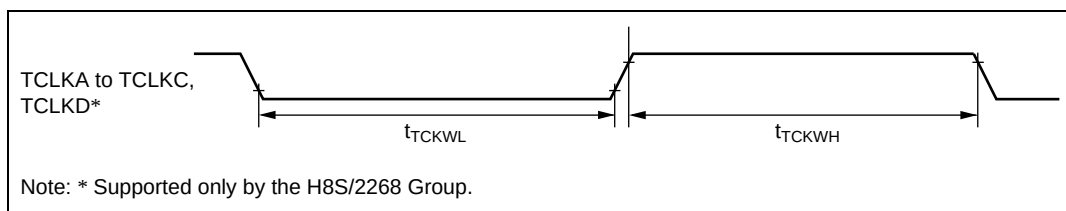
Figure 25.7 TPU Clock Input Timing
