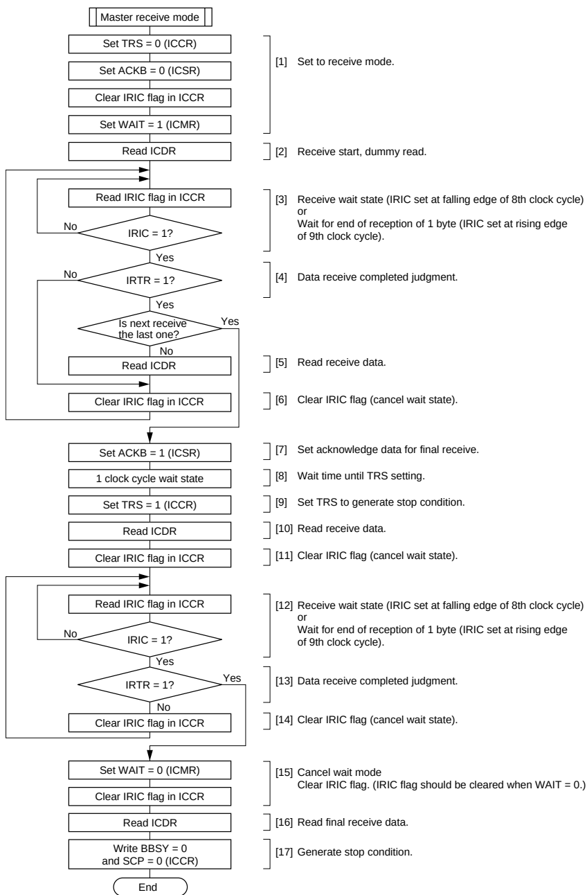
Figure 14.10 Flowchart for Master Receive Mode (Receiving Multiple Bytes) (WAIT = 1) (Example)
