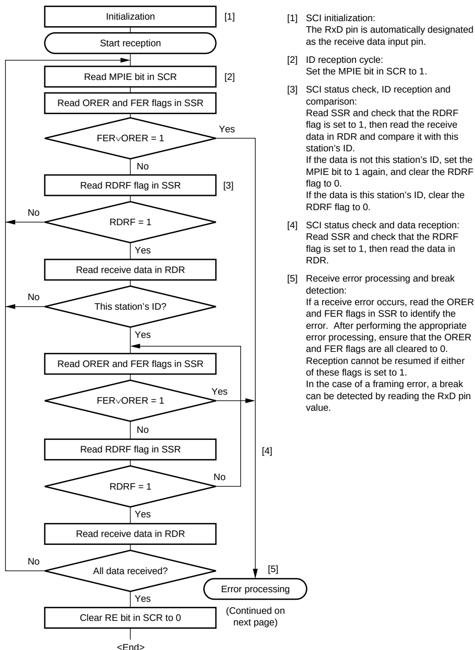
Figure 13.16 Sample Multiprocessor Serial Reception Flowchart (1)
