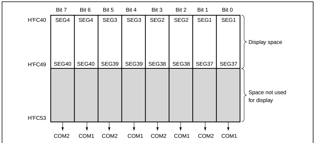
Figure 17.6 LCD RAM Map (1/2 Duty)
