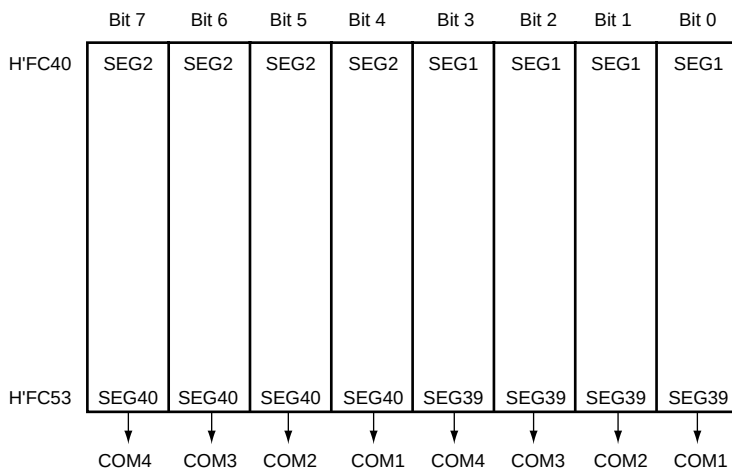
Figure 17.4 LCD RAM Map (1/4 Duty)
