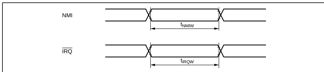
Figure 25.6 Interrupt Input Timing
