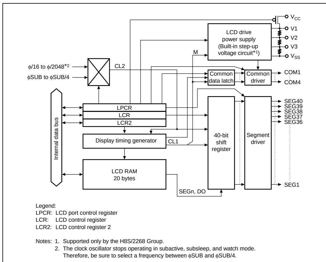
Figure 17.1 Block Diagram of LCD Controller/Driver
