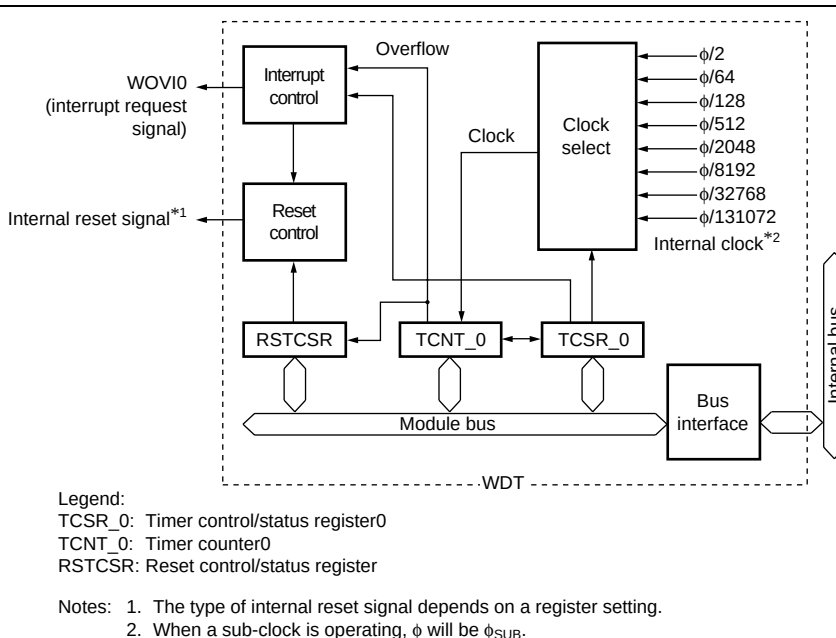
Figure 12.1 Block Diagram of WDT_0
