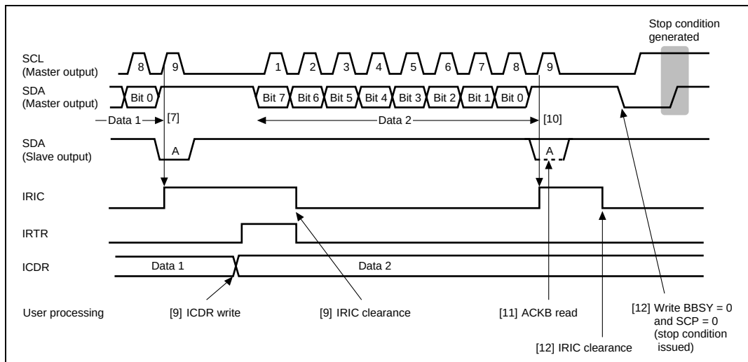
Figure 14.9 Example of Master Transmit Mode Stop Condition Generation Timing (MLS = WAIT = 0)
