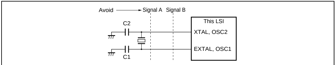
Figure 21.11 Note on Board Design of Oscillator Circuit
