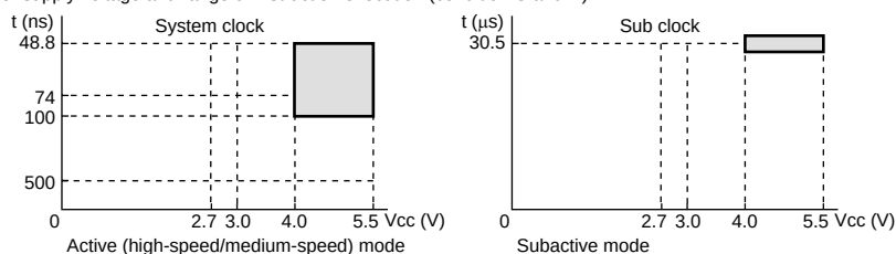
Figure 25.1 Power Supply Voltage and Operating Ranges (2)
