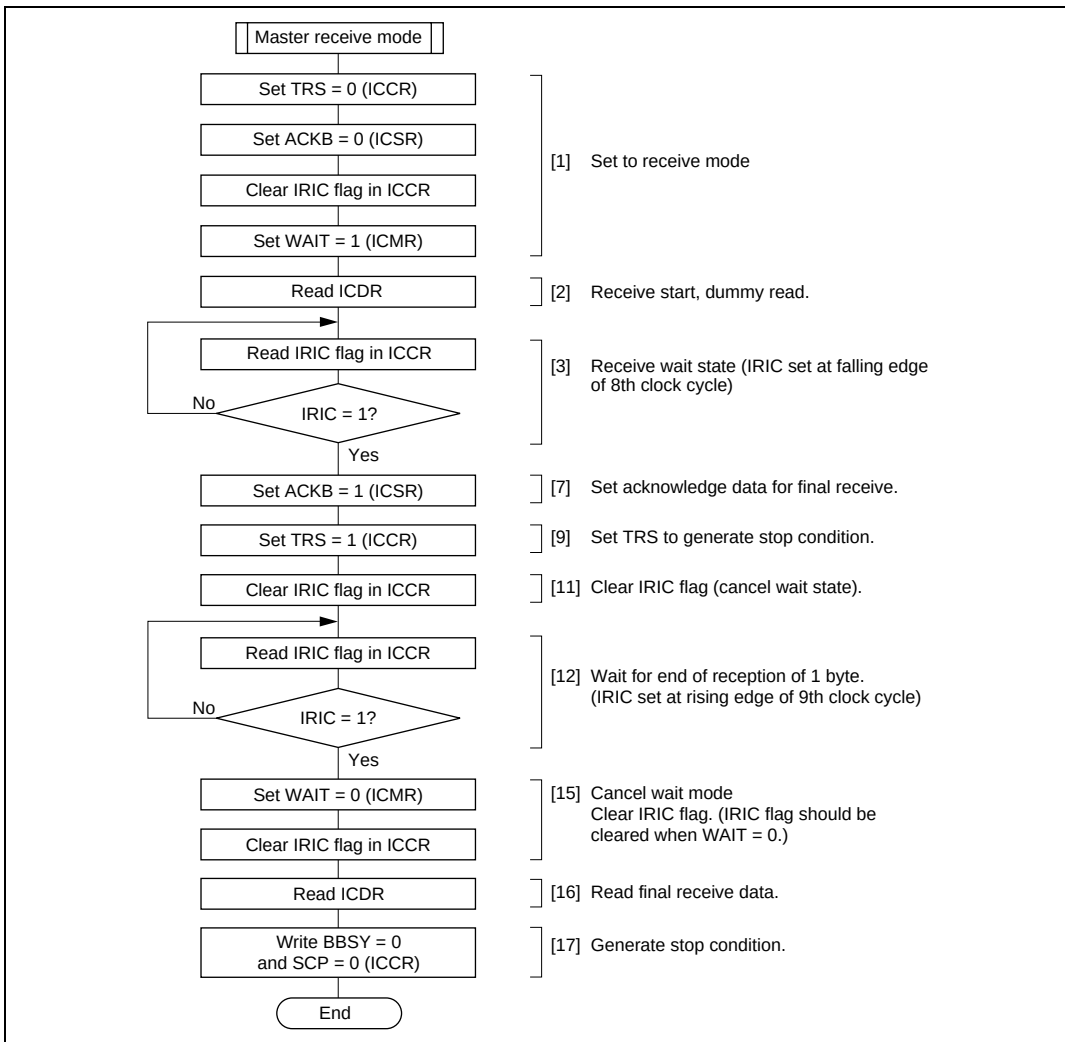
Figure 14.11 Flowchart for Master Receive Mode (Receiving 1 Byte) (WAIT = 1) (Example)
