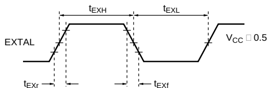
Figure 21.5 External Clock Input Timing
