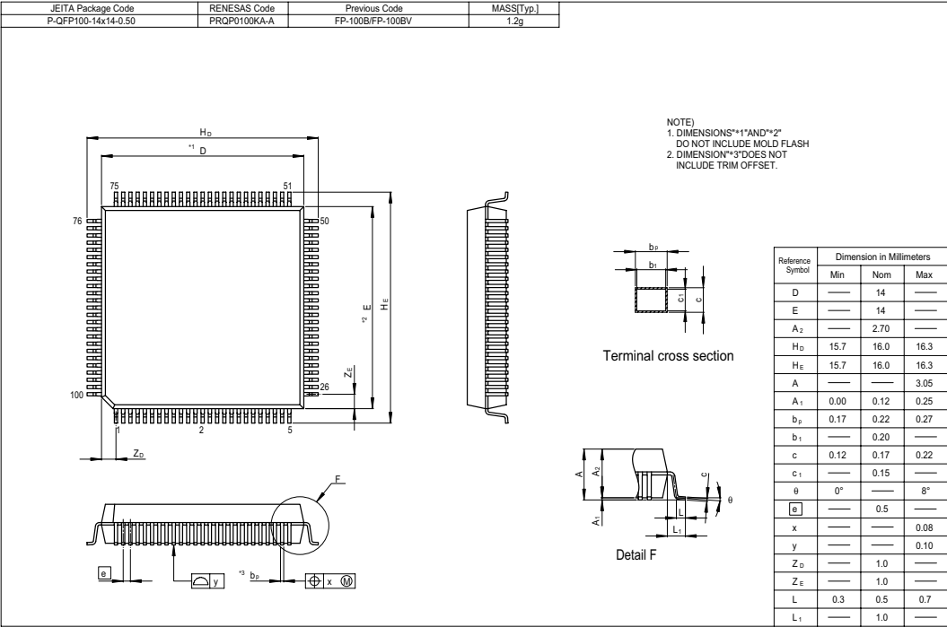
Figure C.3 FP-100B Package Dimensions
