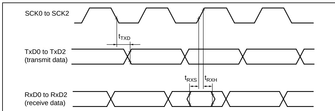
Figure 25.10 SCI Input/Output Timing (Clock Synchronous Mode)
