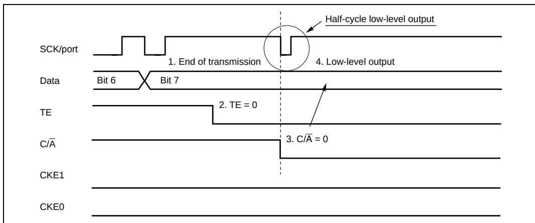
Figure 13.41 Operation when Switching from SCK Pin Function to Port Pin Function
