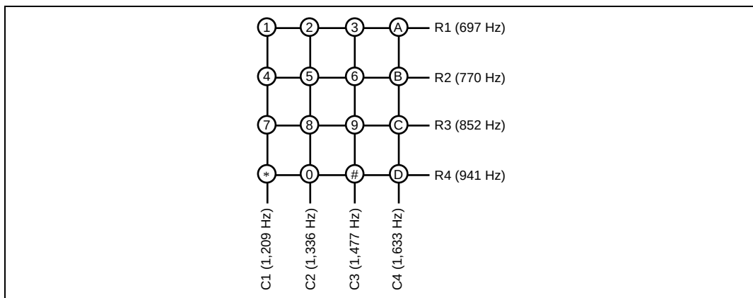
Figure 18.1 DTMF Frequencies
