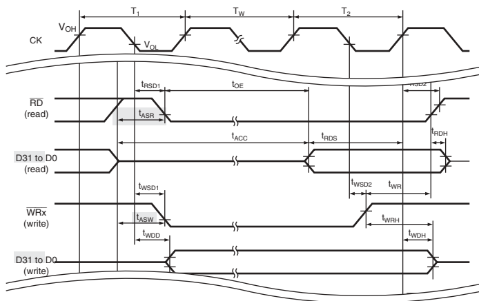
Figure 26.10 Basic Cycle (One Software Wait) 763
