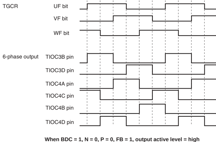
Figure 11.52 Example of Output Phase Switching by Means of UF, VF, WF Bit Settings (1)
