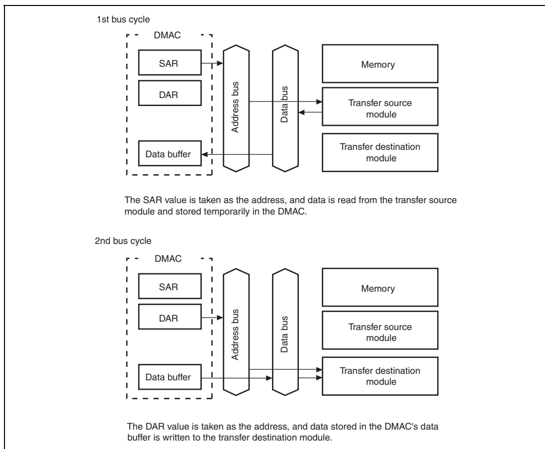
Figure 10.6 Direct Address Operation during Dual Address Mode
