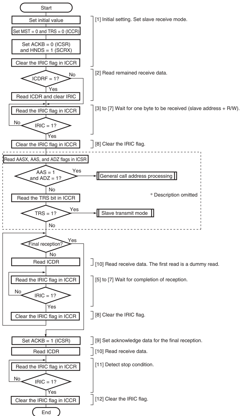
Figure 14.17 Example: Flowchart of Operations in the Slave Receive Mode (HNDS = 1)
