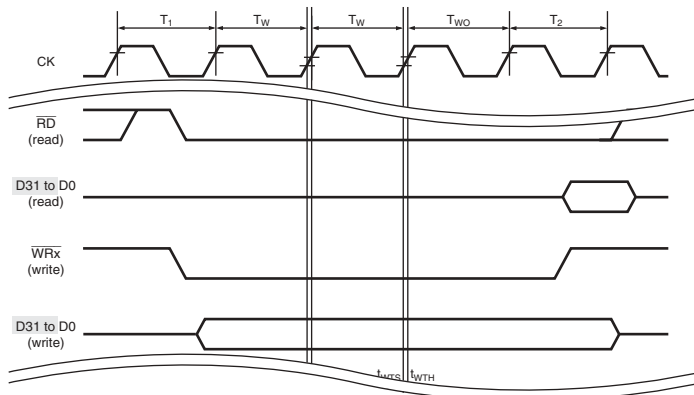
Figure 26.11 Basic Cycle (Two Software Waits + Waits by WAIT Signal) 764
