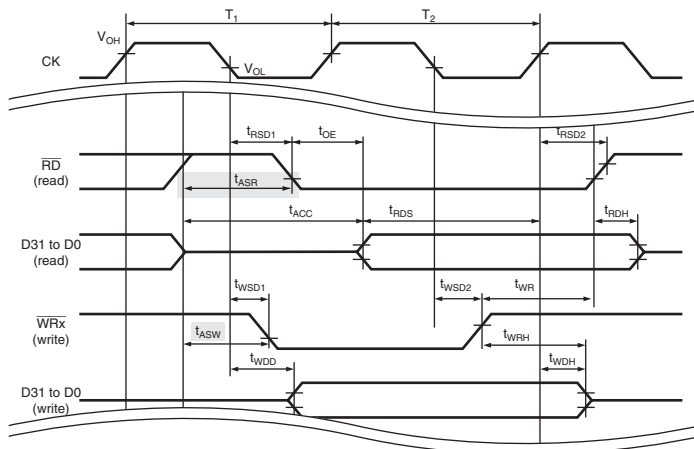
Figure 26.9 Basic Cycle 762 (No Waits)
