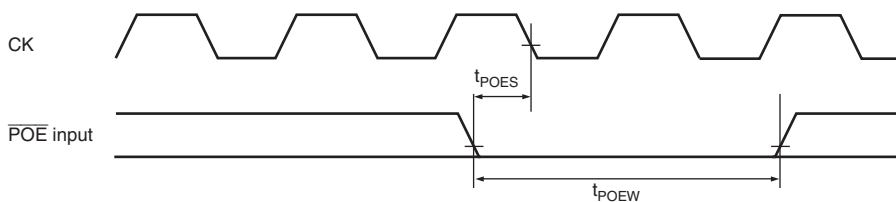
Figure 26.22 \overline{\text{POE}} Input/Output Timing
