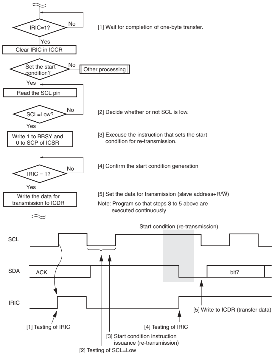
Figure 14.30 Flowchart and Timing of the Execution of the Instruction that Sets the Start Condition for Re-Transmission
