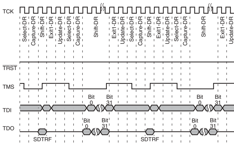
Figure 22.4 Data Input/Output Timing Chart (3)
