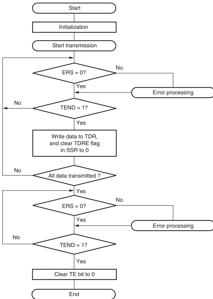
Figure 13.28 Example of Transmit Processing Flow
