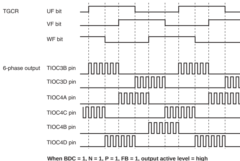
Figure 11.53 Example of Output Phase Switching by Means of UF, VF, WF Bit Settings (2)
