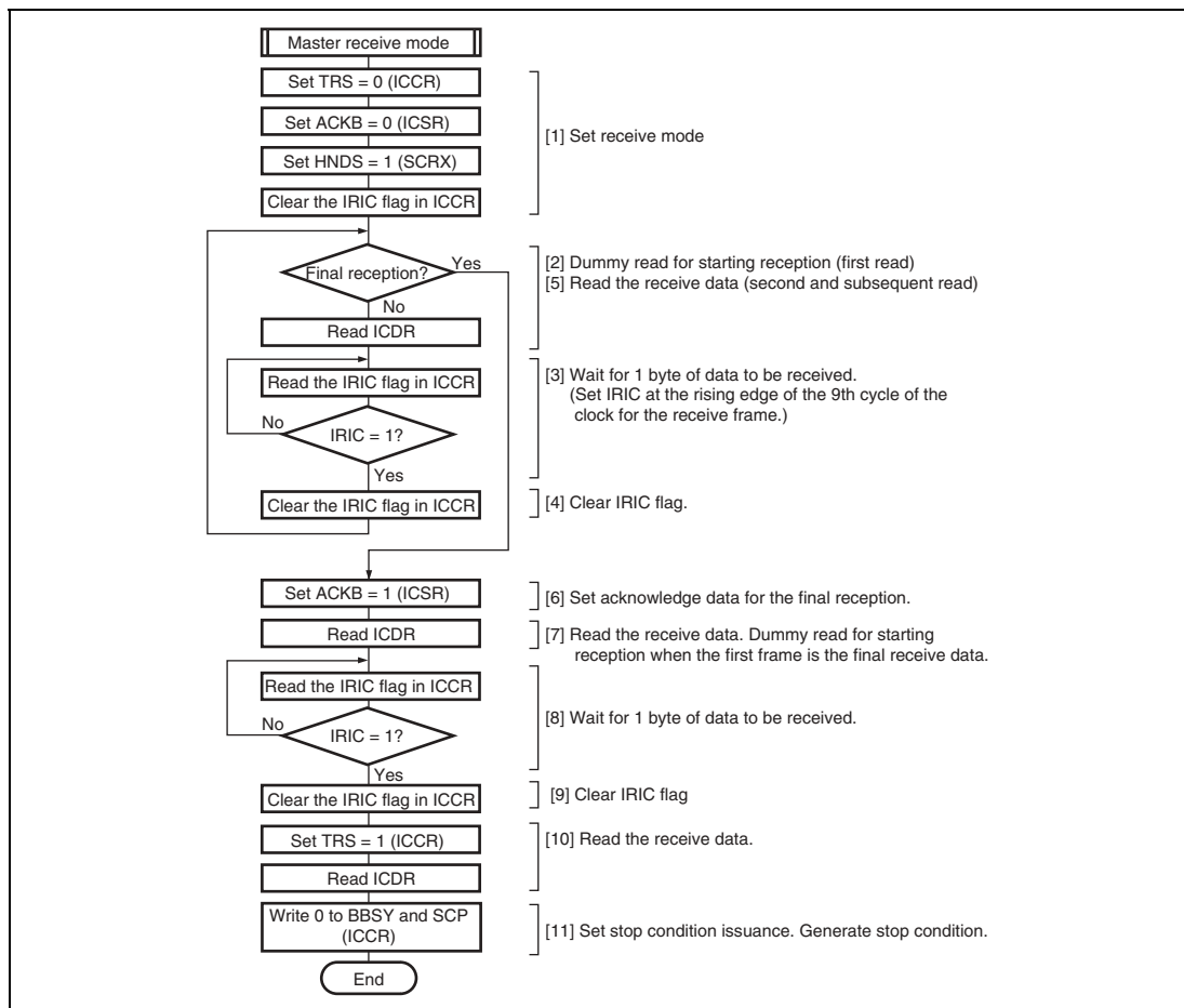
Figure 14.10 Example: Flowchart of Operations in the Master Receive Mode (HNDS = 1)
