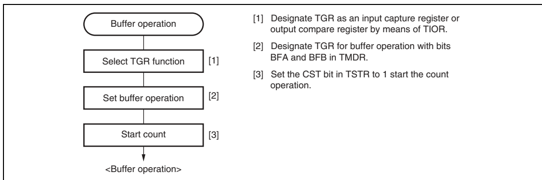
Figure 11.15 Example of Buffer Operation Setting Procedure
