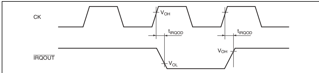
Figure 26.7 Interrupt Signal Output Timing
