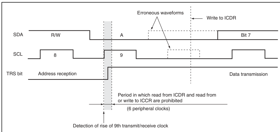
Figure 14.33 Timing for Reading ICDR and Accessing ICCR in Slave Transmit Mode
