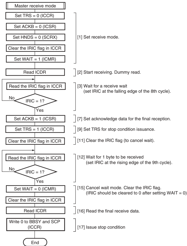
Figure 14.14 Example: Flowchart of Operations in Master Receive Mode (One Byte Reception) (WAIT = 1)
