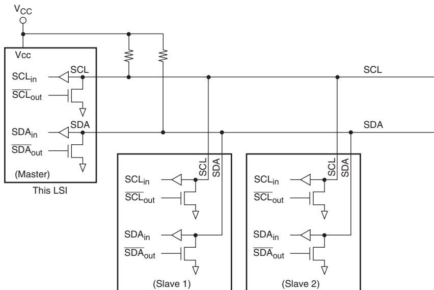
Figure 14.2 Example of the Connection of I 2 C Bus Interfaces (This LSI is the Master Device)
