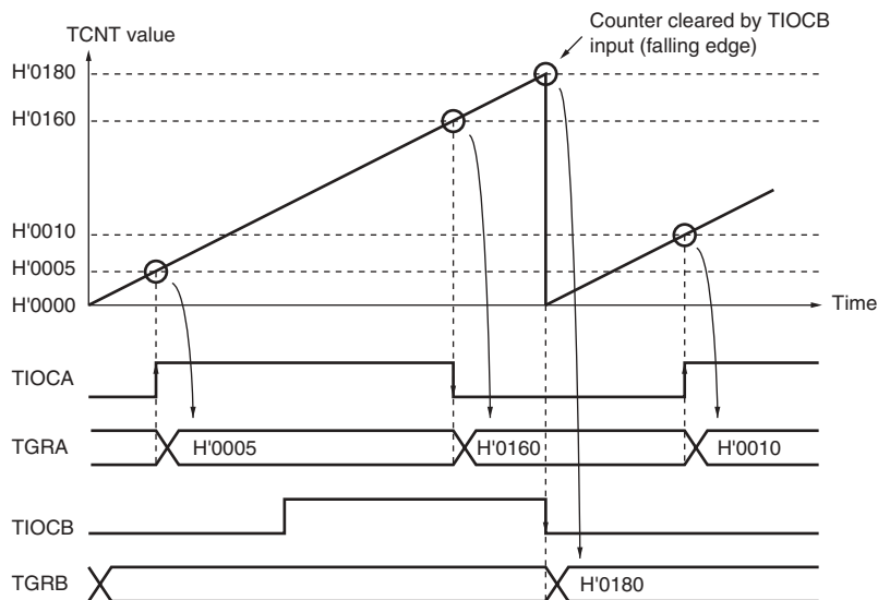
Figure 11.10 Example of Input Capture Operation
