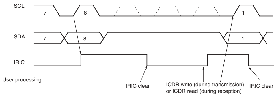
Figure 14.27 IRIC Flag Set Timing and the Control of SCL (3)
