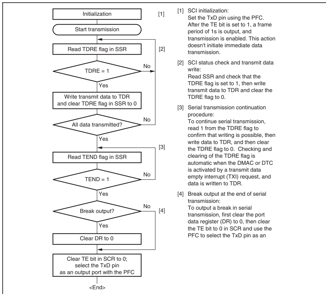
Figure 13.7 Sample Serial Transmission Flowchart
