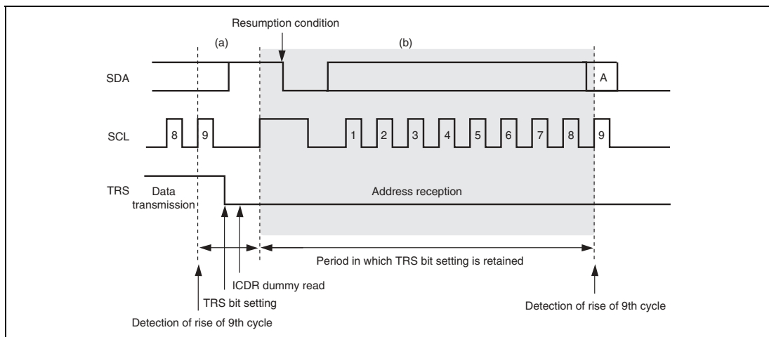
Figure 14.34 Timing for Setting TRS Bit in Slave Mode
