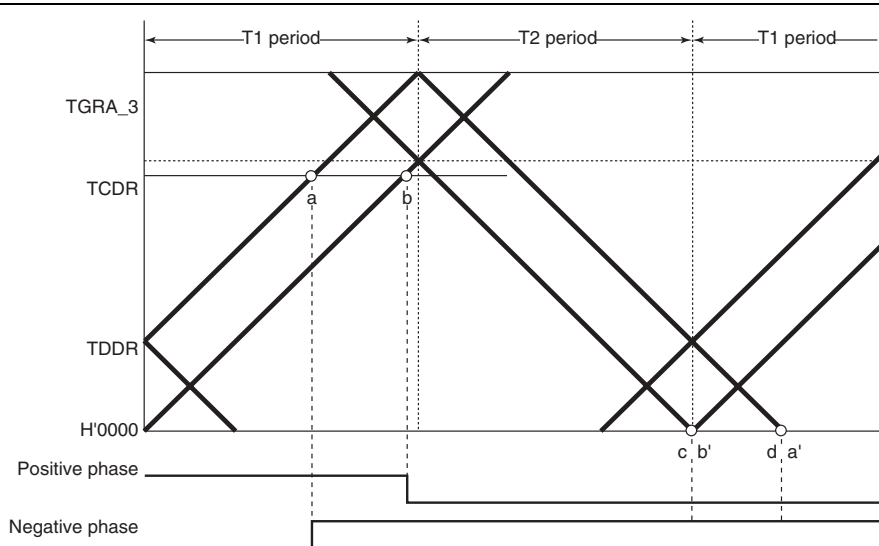
Figure 11.46 Example of Complementary PWM Mode 0% and 100% Waveform Output (4)
