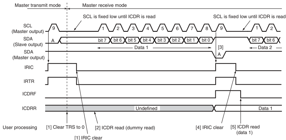
Figure 14.11 An Example of the Timing of Operations in Master Receive Mode (MLS = WAIT = 0, HNDS = 1)
