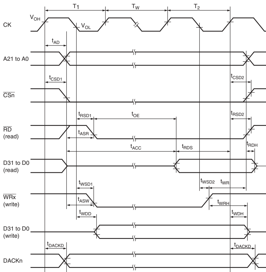
Figure 26.10 Basic Cycle (One Software Wait)
