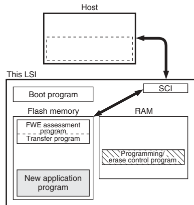
Figure 19.4 User Program Mode
