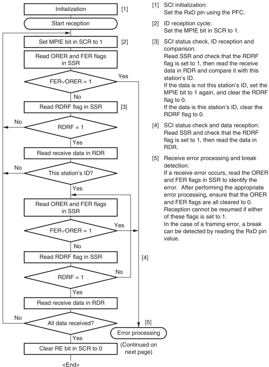
Figure 13.13 Sample Multiprocessor Serial Reception Flowchart (1)
