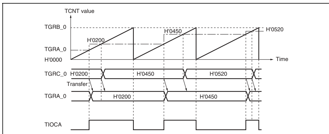
Figure 11.16 Example of Buffer Operation (1)
