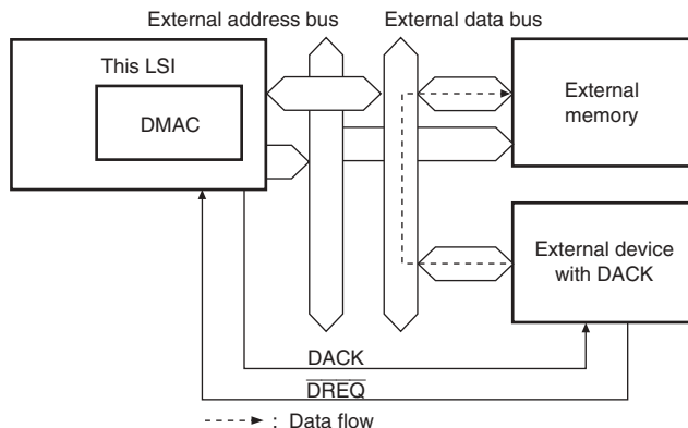
Figure 10.4 Data Flow in Single Address Mode
