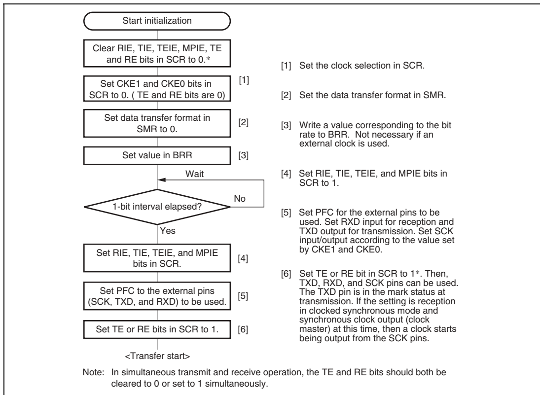
Figure 13.15 Sample SCI Initialization Flowchart
