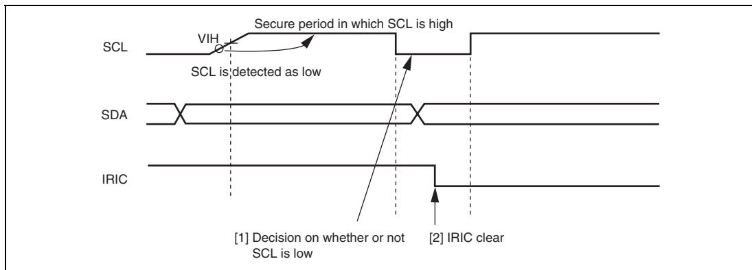
Figure 14.32 Timing for Clearing IRIC Flag When WAIT = 1
