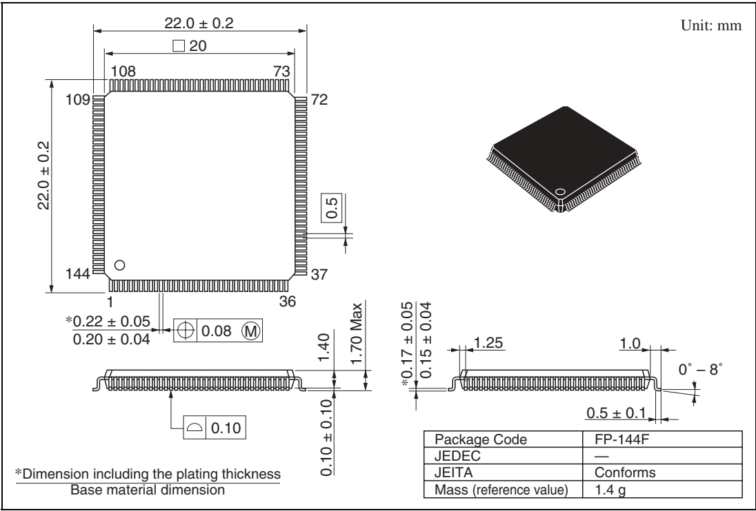
Figure E.2 FP-144F
