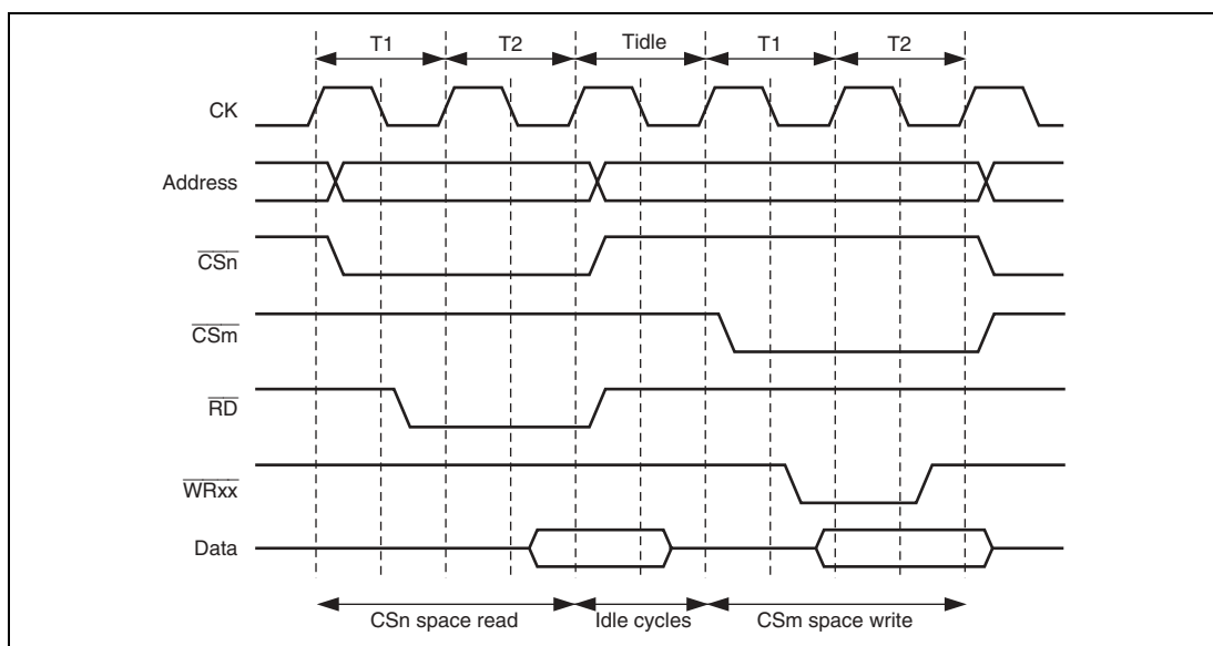
Figure 9.7 Example of Idle Cycle Insertion
