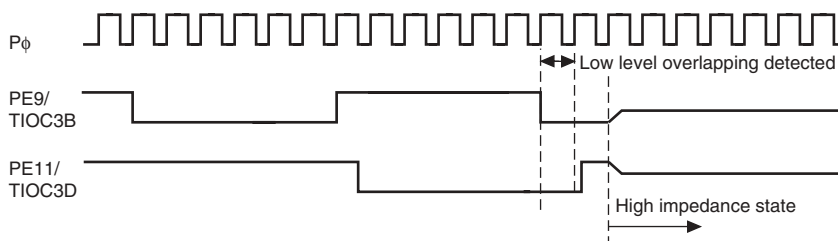
Figure 11.116 Output-Level Detection Operation
