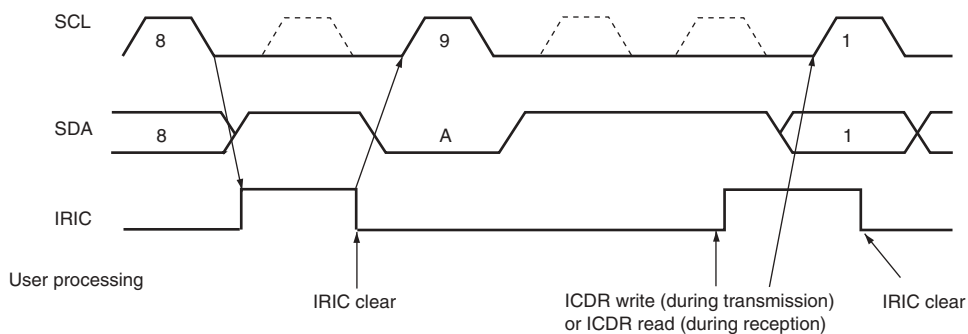
Figure 14.26 IRIC Flag Set Timing and the Control of SCL (2)
