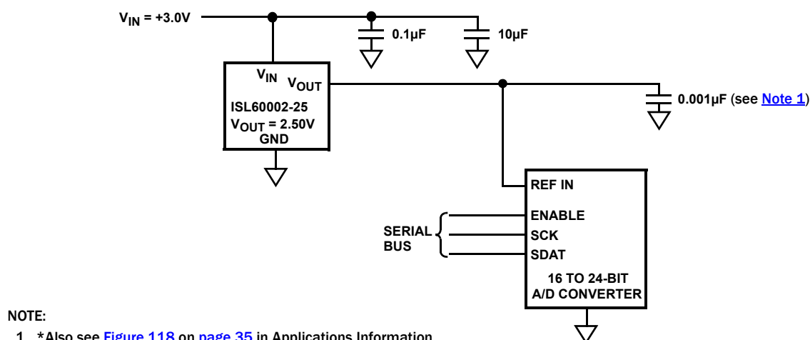
FIGURE 1. TYPICAL APPLICATION
