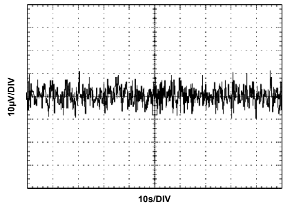
FIGURE 41. V_{OUT} NOISE
