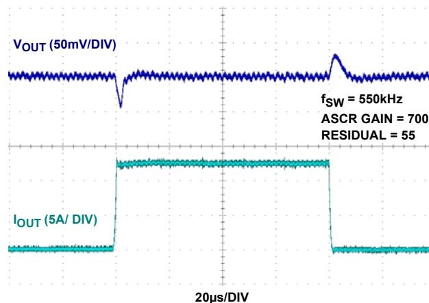
FIGURE 11. 1V TRANSIENT RESPONSE
