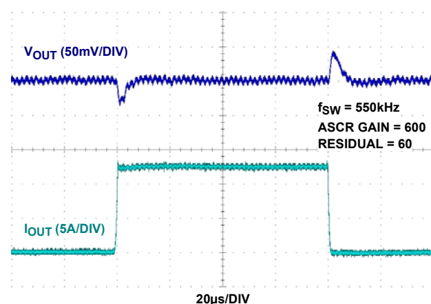
FIGURE 13. 1.8V TRANSIENT RESPONSE
