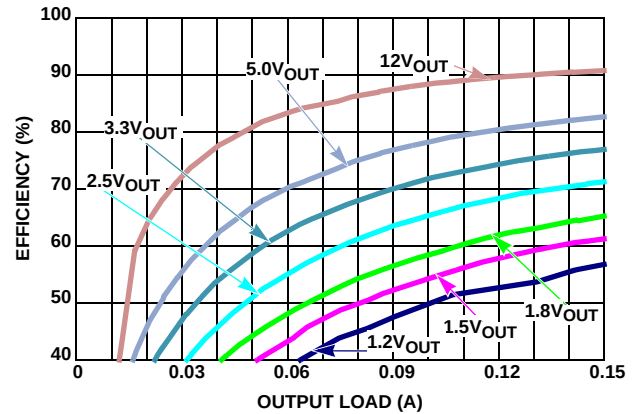
FIGURE 10. EFFICIENCY vs LOAD, PWM, V_{IN} = 36\text{V}
