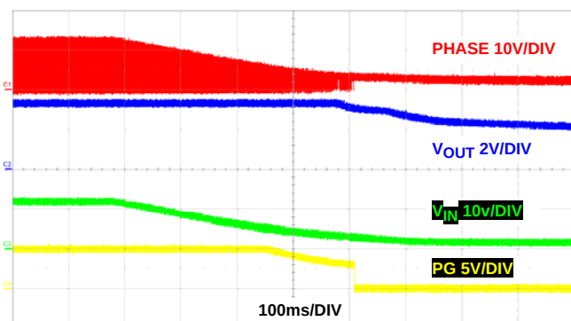
FIGURE 34. SHUTDOWN V_{IN} AT NO LOAD, PWM
