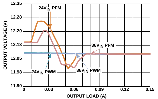
FIGURE 18. V_{OUT} REGULATION vs LOAD, V_{OUT} = 12\text{V}
