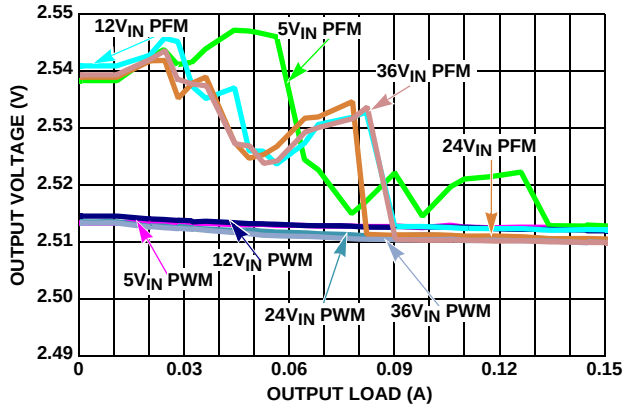
FIGURE 15. V_{OUT} REGULATION vs LOAD, V_{OUT} = 2.5\text{V}
