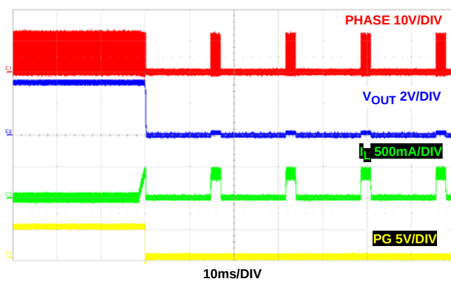
FIGURE 44. OVERCURRENT PROTECTION
