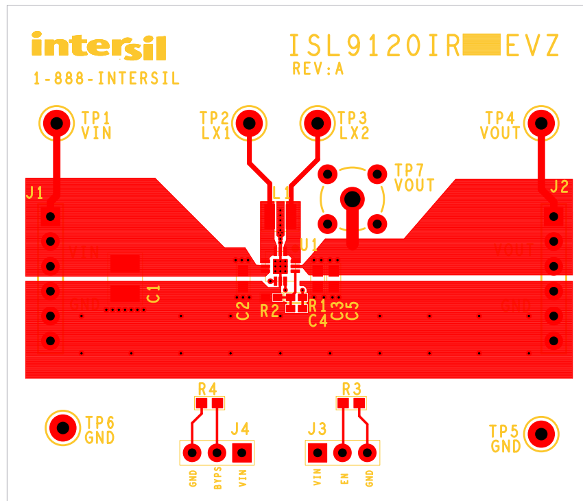
FIGURE 8. TOP LAYER
