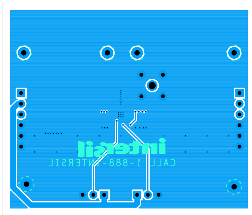
FIGURE 9. BOTTOM LAYER
