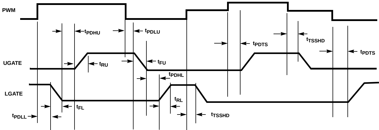
FIGURE 2. TIMING DIAGRAM
