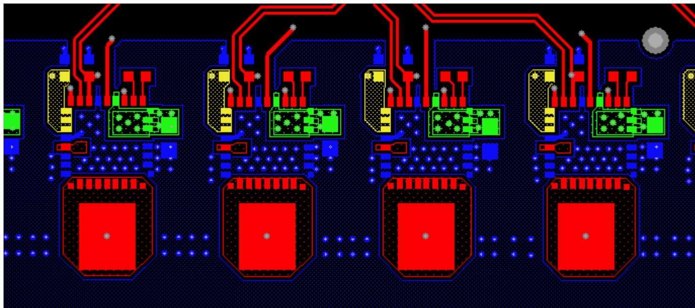
FIGURE 16. MULTIPHASE PCB LAYOUT EXAMPLE TOP LAYER
