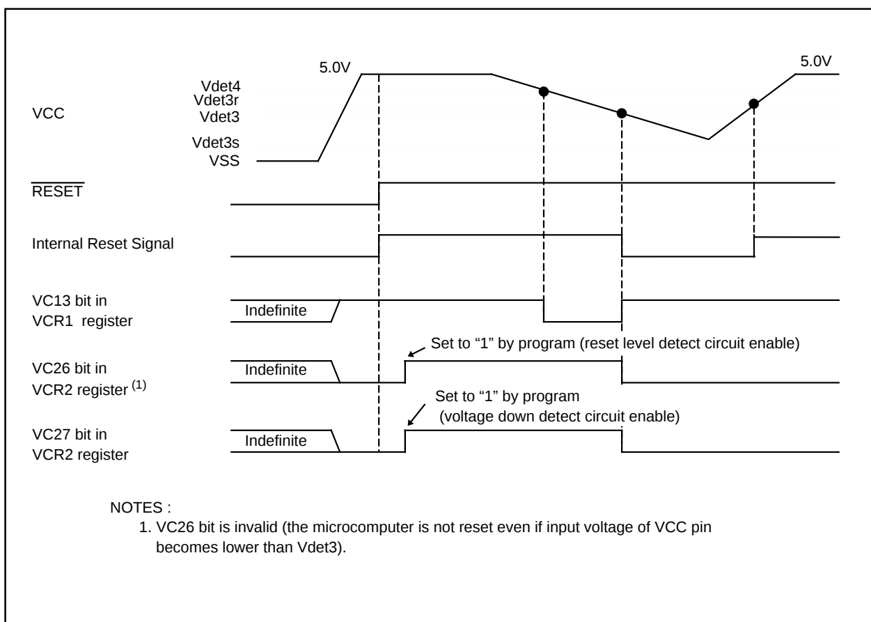
Figure 5.5.3. Typical Operation of Hardware Reset 2
