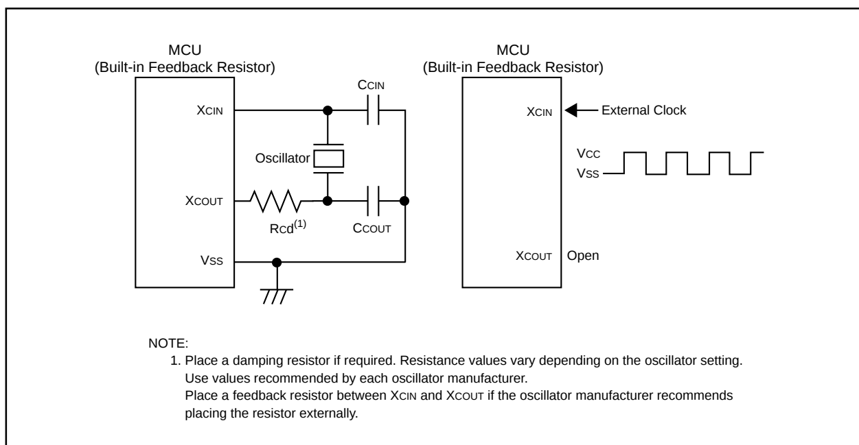
Figure 7.2.1. Examples of Sub Clock Connection Circuit
