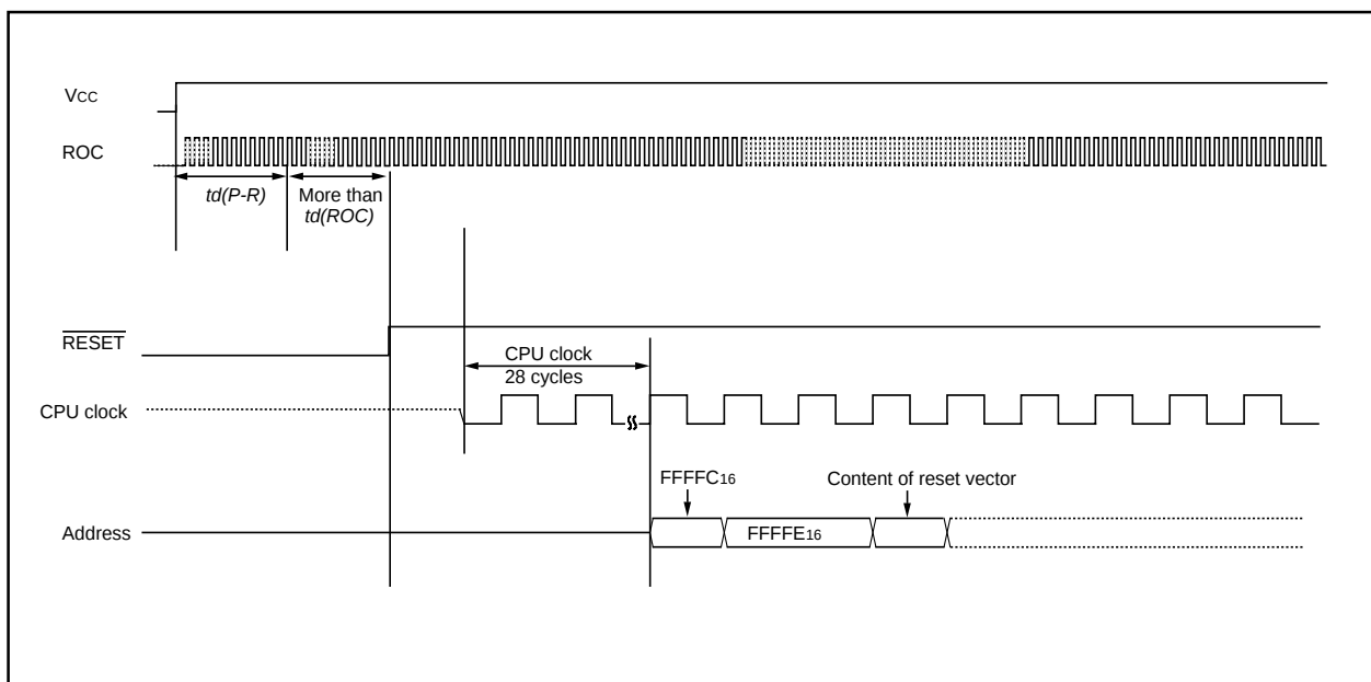
Figure 5.1.1.2. Reset Sequence
