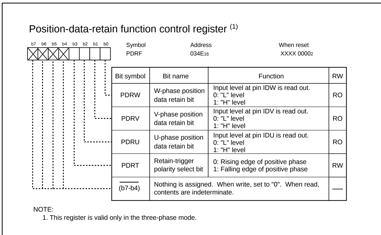
Figure 12.3.1.2.1. PDRF Register
