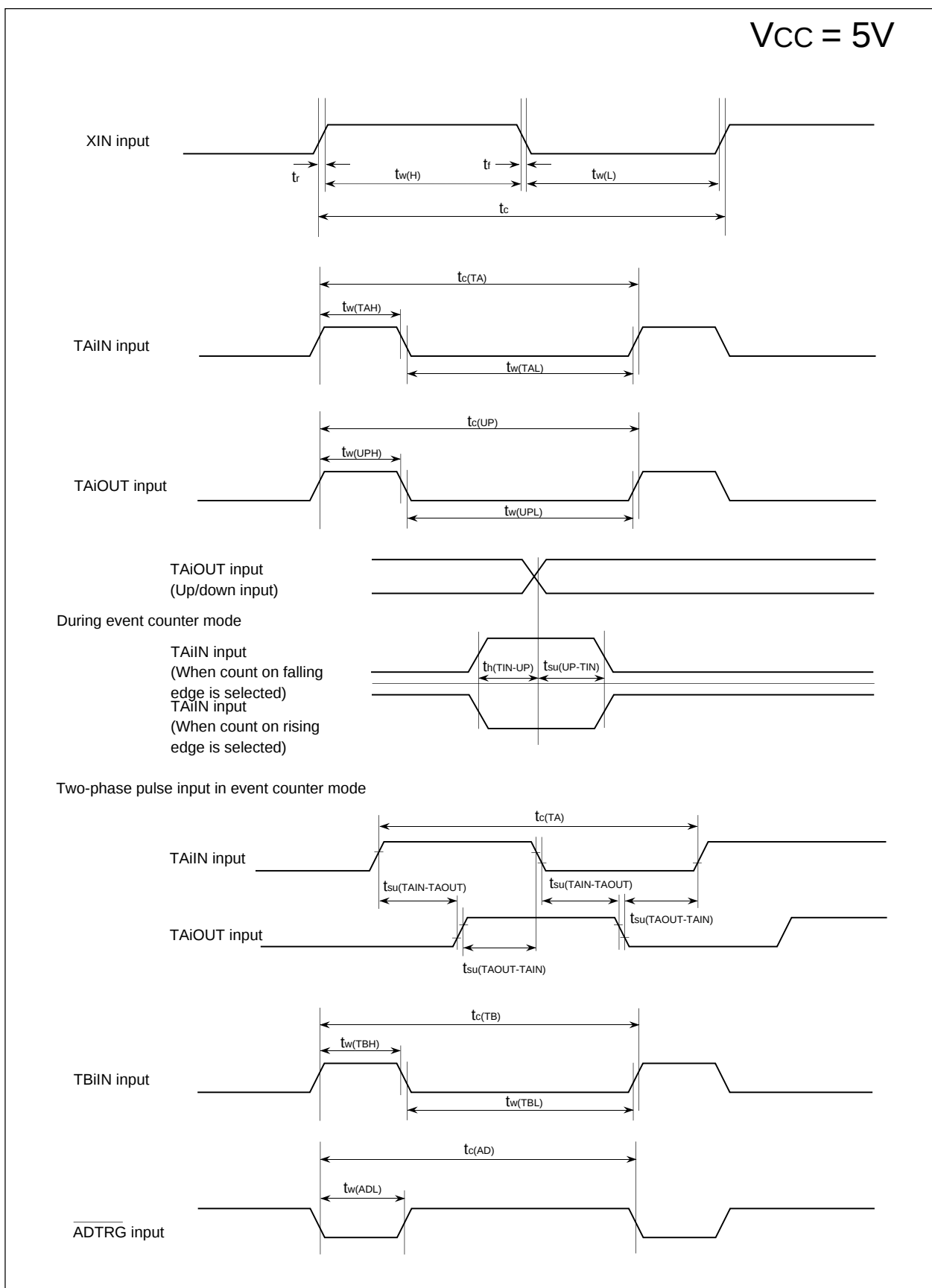
Figure 18.5. Timing Diagram (1)
