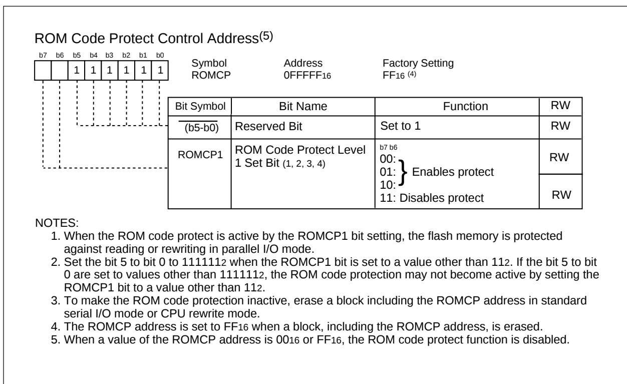
Figure 17.3.1.1. ROMCP Address
