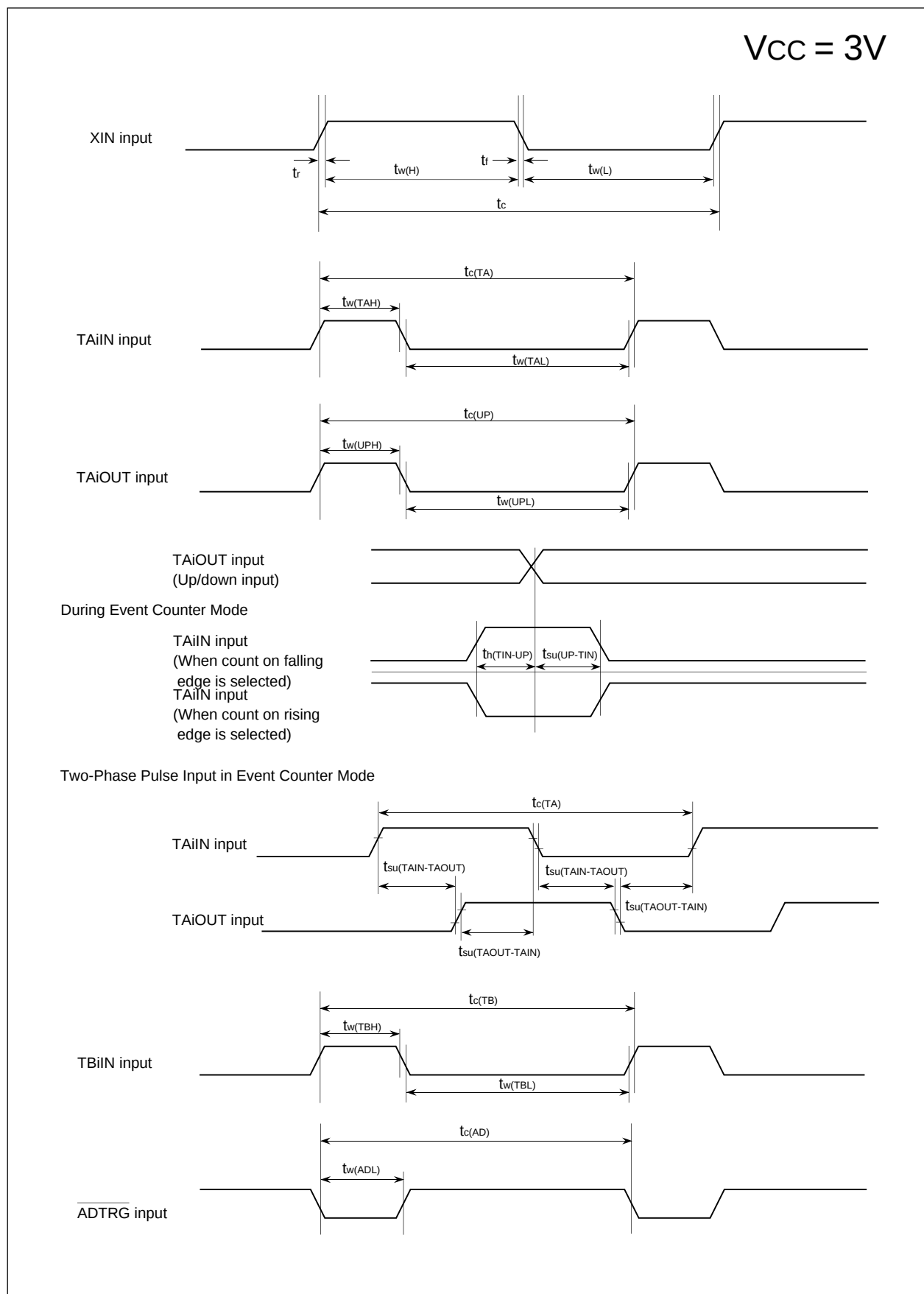
Figure 18.7. Timing Diagram (1)
