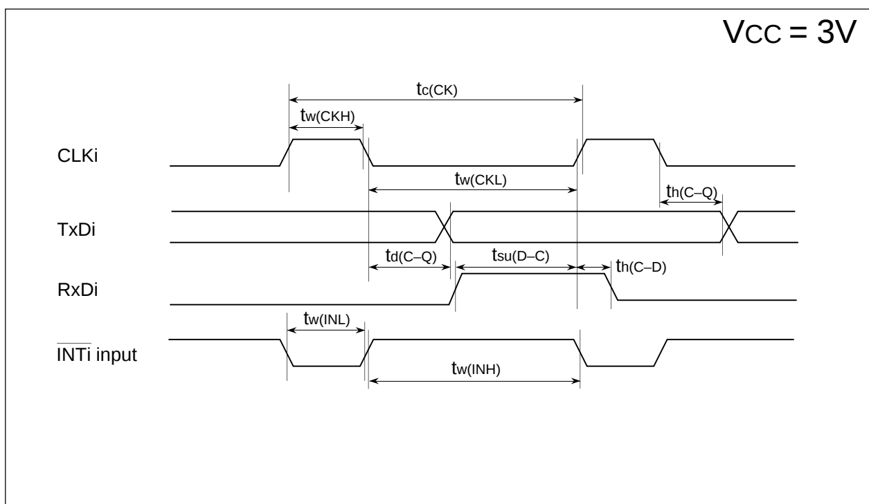
Figure 18.8. Timing Diagram (2)
