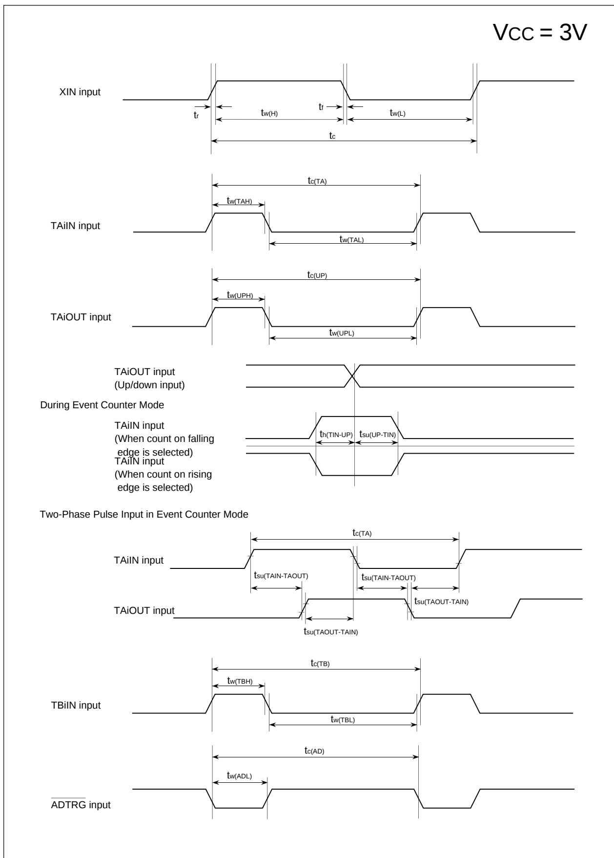
Figure 18.3. Timing Diagram (1)
