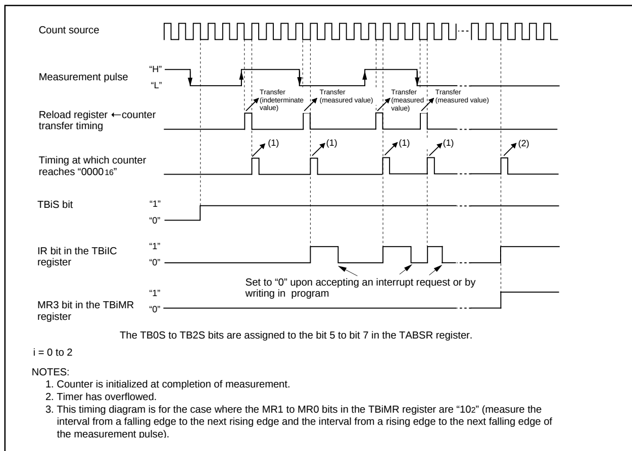
Figure 12.2.3.3 Operation timing when measuring a pulse width
