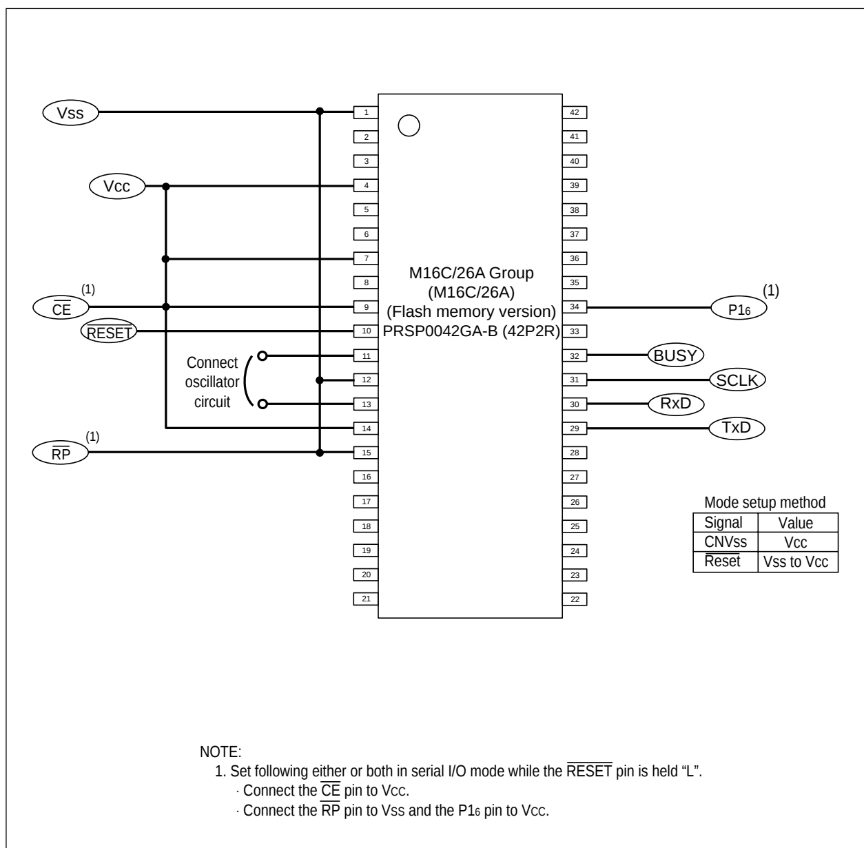
Figure 17.9.1. Pin Connections for Serial I/O Mode (1)
