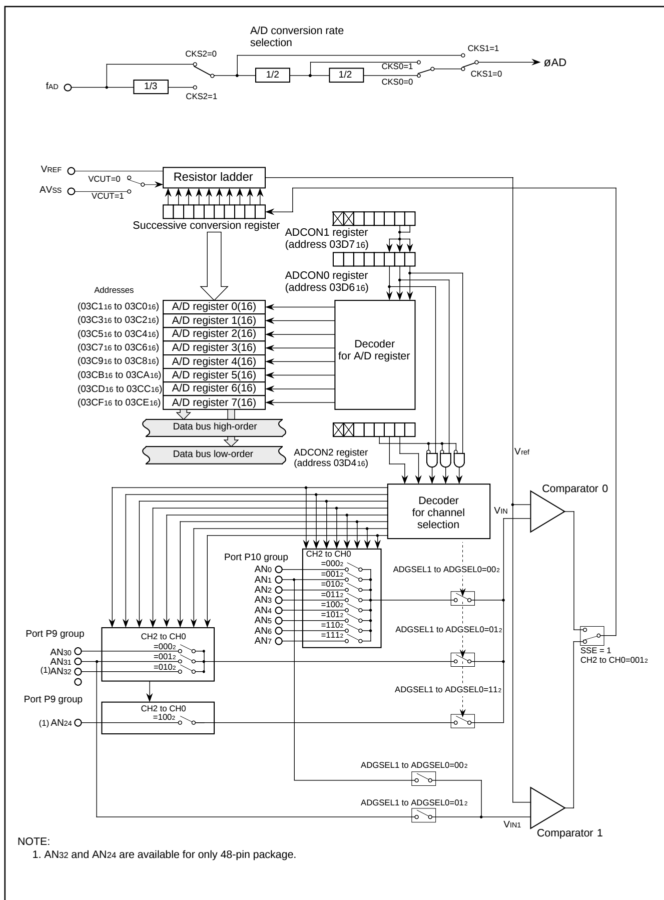
Figure 14.1 A/D Converter Block Diagram
