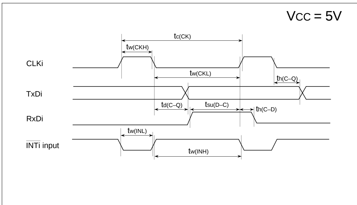
Figure 18.6. Timing Diagram (2)
