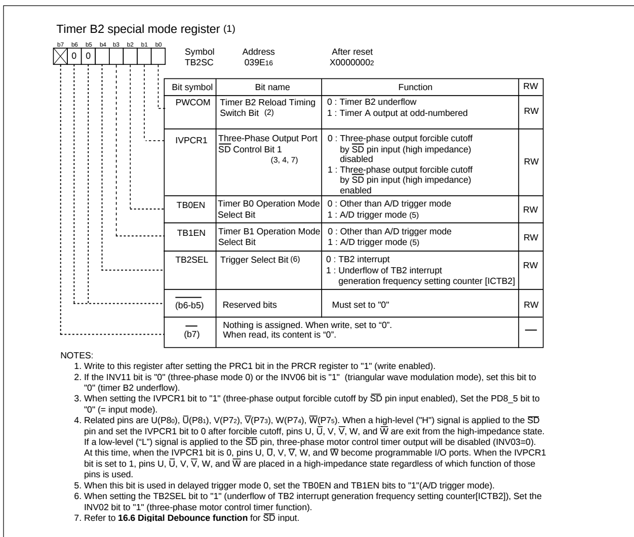
Figure 12.2.4.2 TB2SC Register
