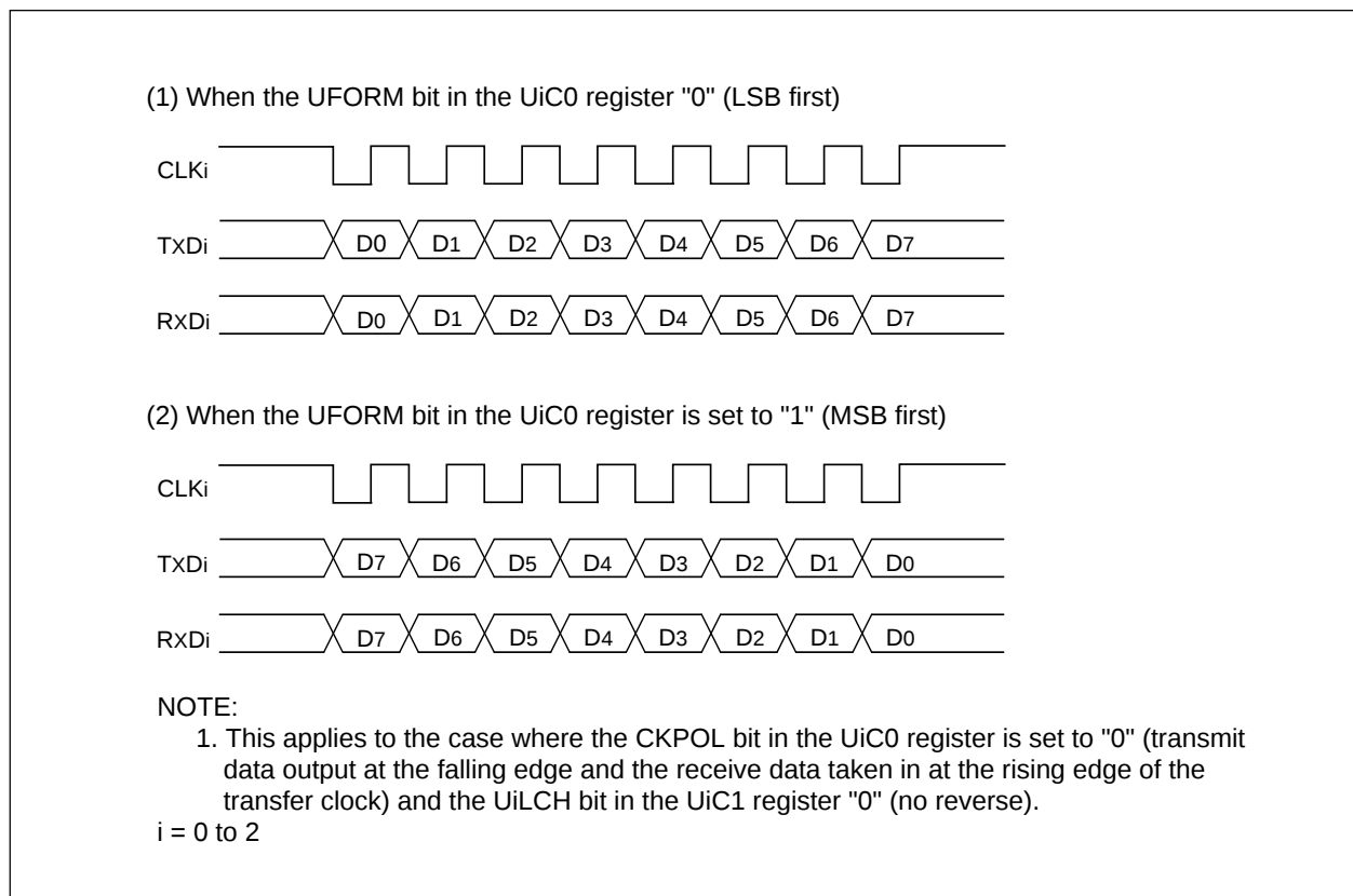
Figure 13.1.1.3.1 Transfer format
