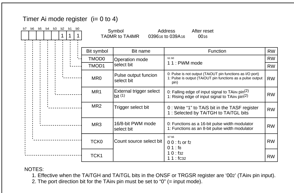
Figure 12.1.4.1. TAIiMR Register in Pulse Width Modulation Mode
