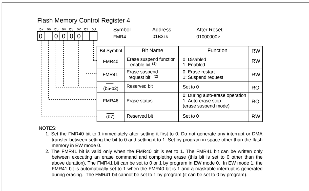
Figure 17.5.2. FMR4 register
