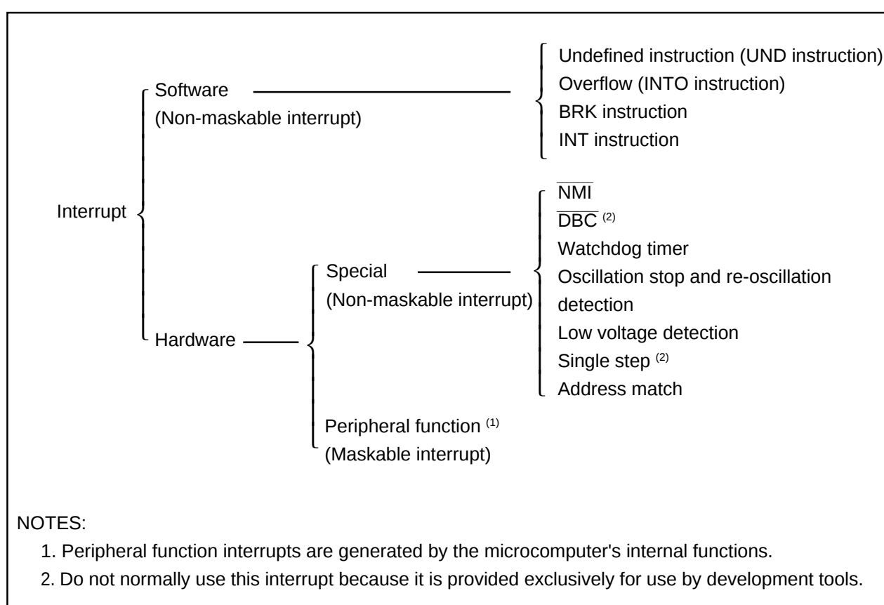
Figure 9.1.1. Interrupts
