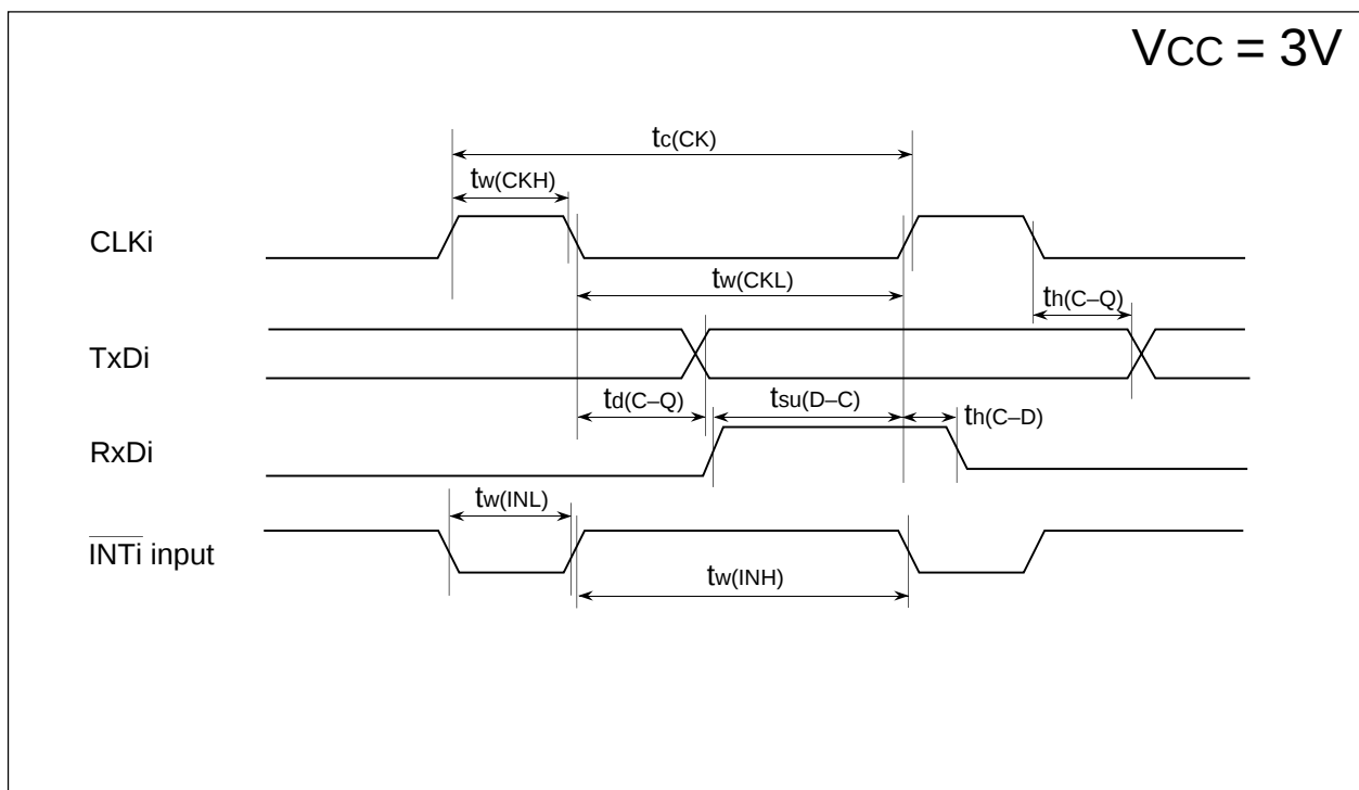
Figure 18.4. Timing Diagram (2)
