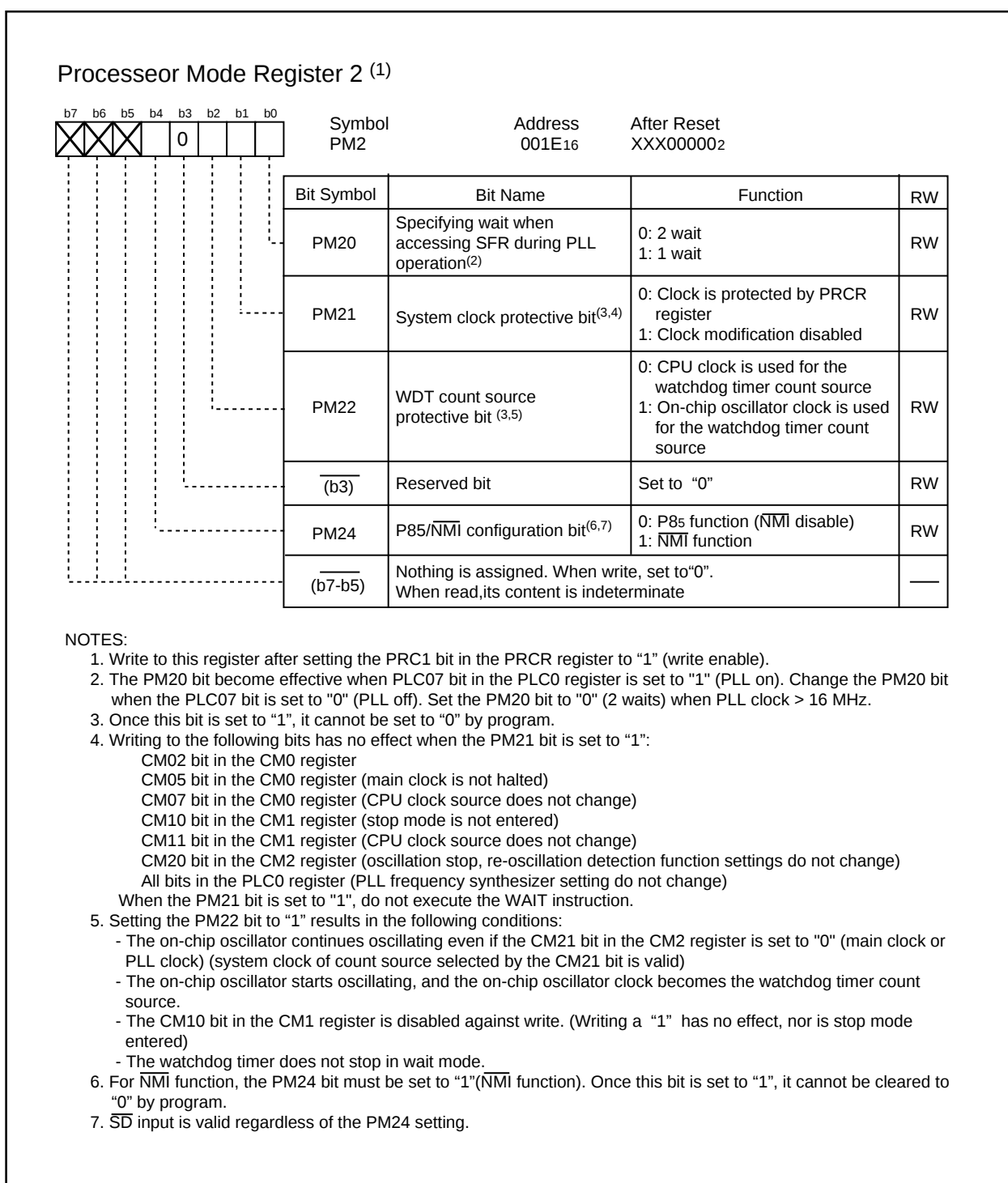
Figure 6.2 PM2 Register
