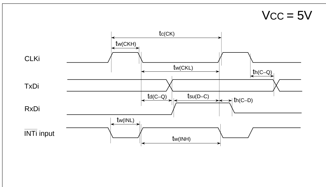
Figure 18.2. Timing Diagram (2)
