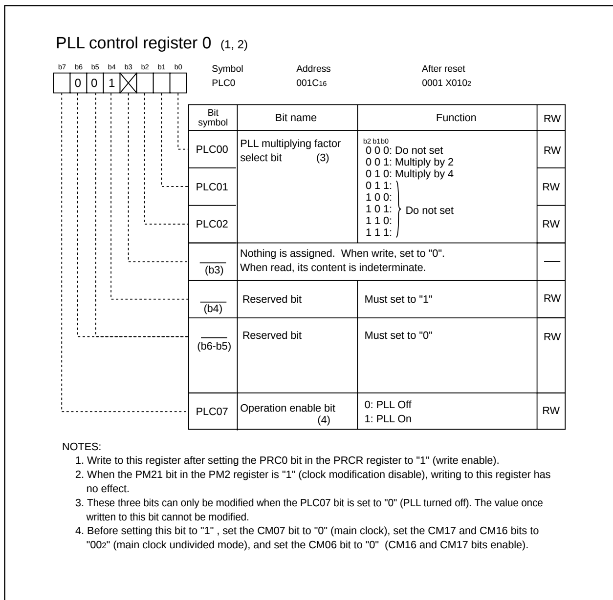
Figure 7.7. PLC0 Register
