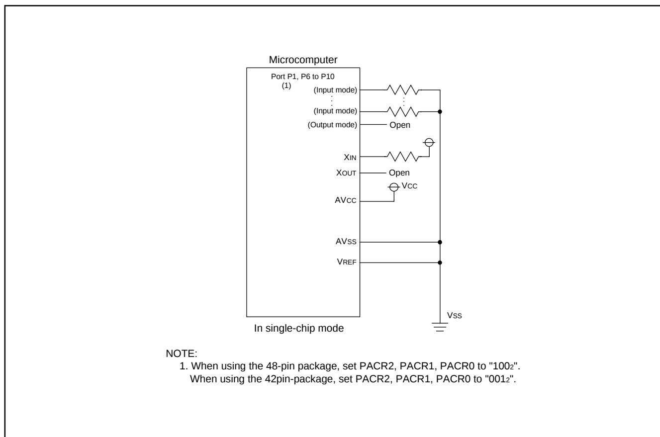
Figure 16.7. Unassigned Pins Handling
