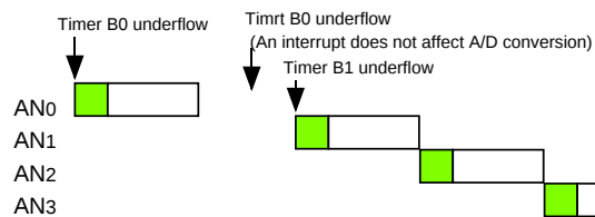
Figure 14.1.7.1 Operation Example in Delayed Trigger Mode 0
