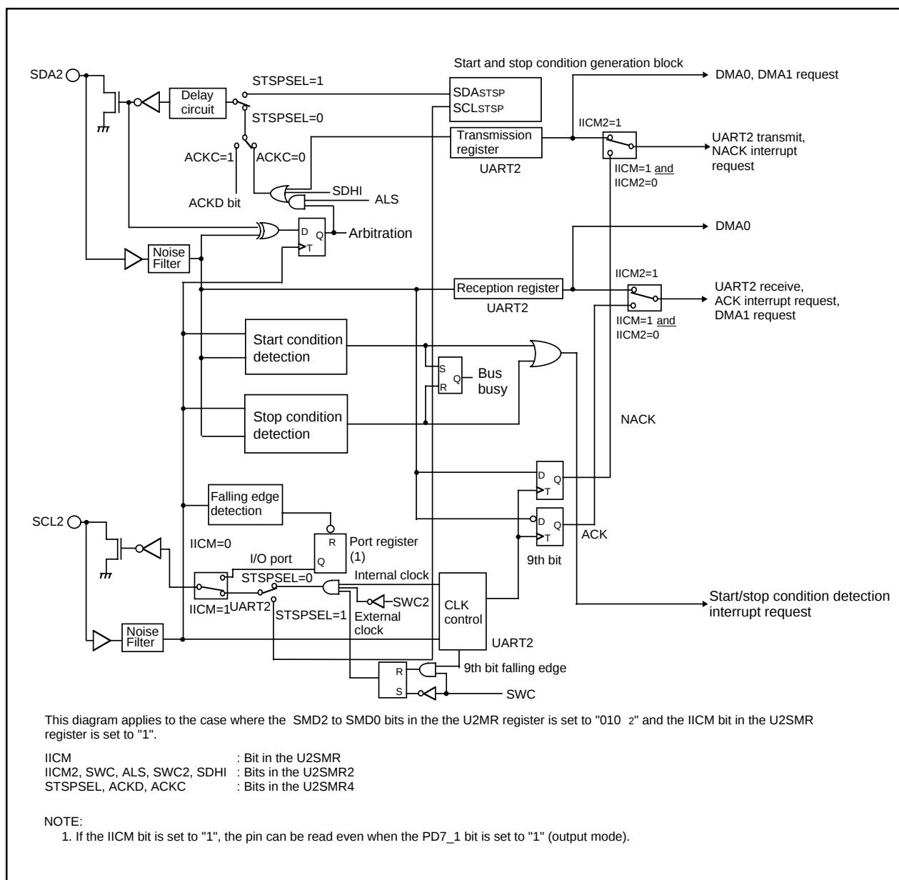
Figure 13.1.3.1. I²C bus Mode Block Diagram
