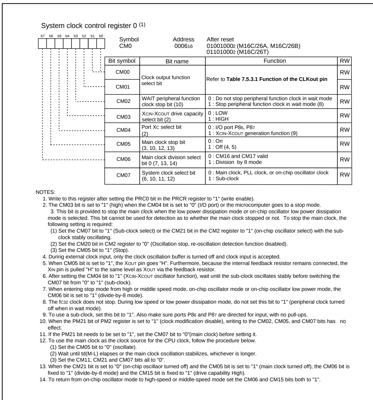
Figure 7.2. CM0 Register
