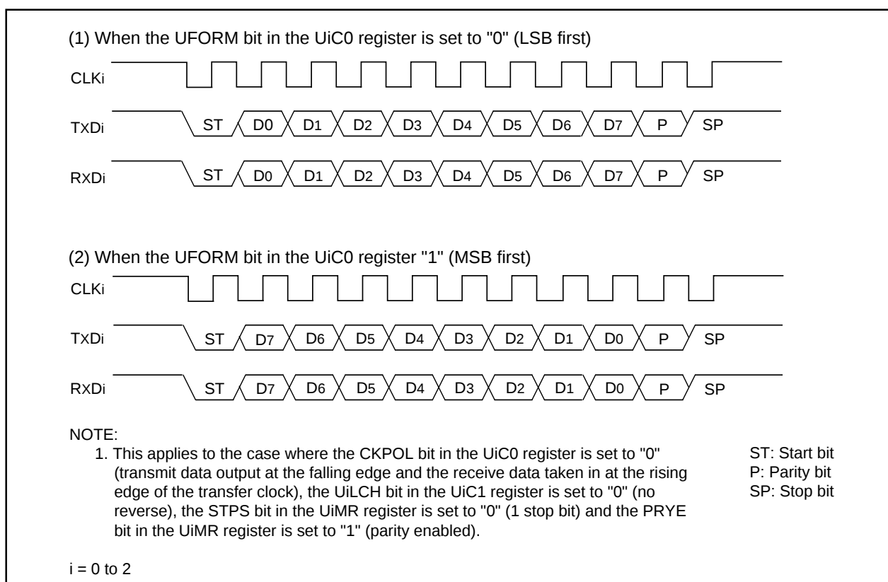
Figure 13.1.2.3.1. Transfer Format
