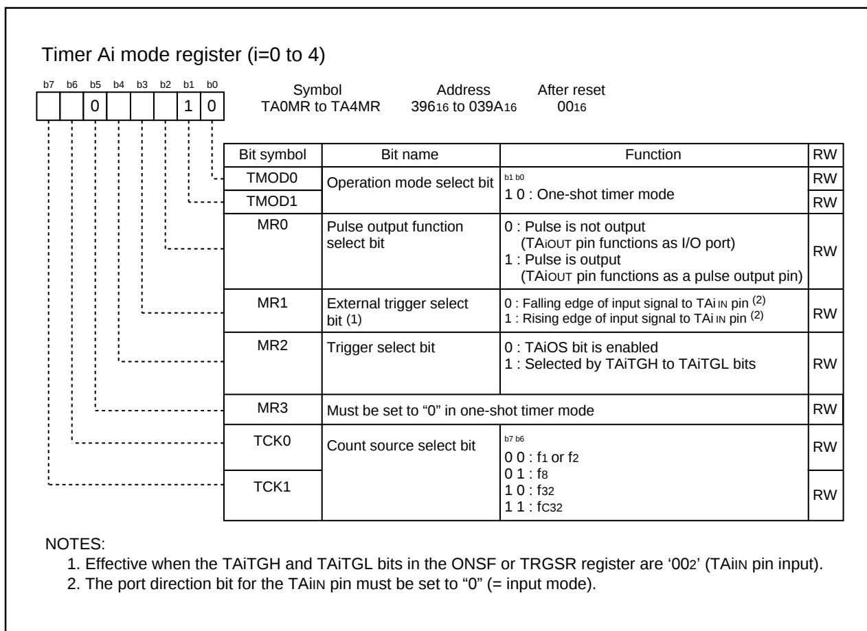
Figure 12.1.3.1. TAI i MR Register in One-shot Timer Mode
