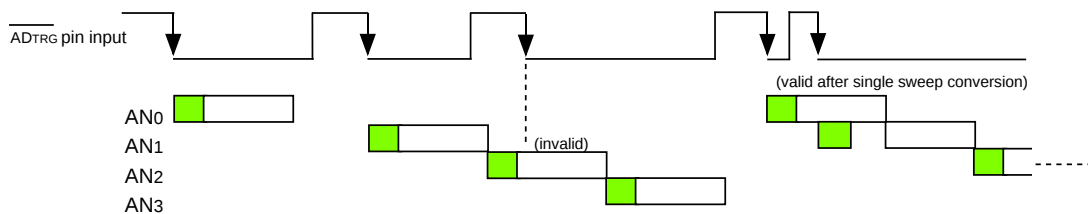
Figure 14.1.8.1 Operation Example in Delayed Trigger Mode1
