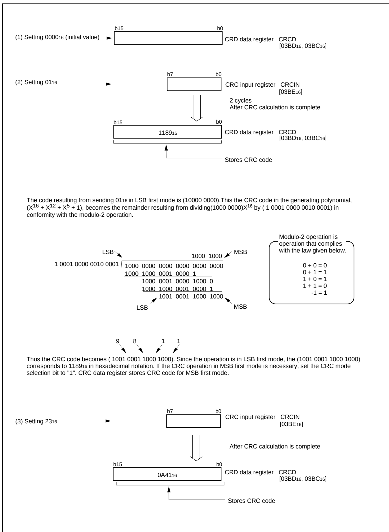
Figure 15.3. CRC Calculation
