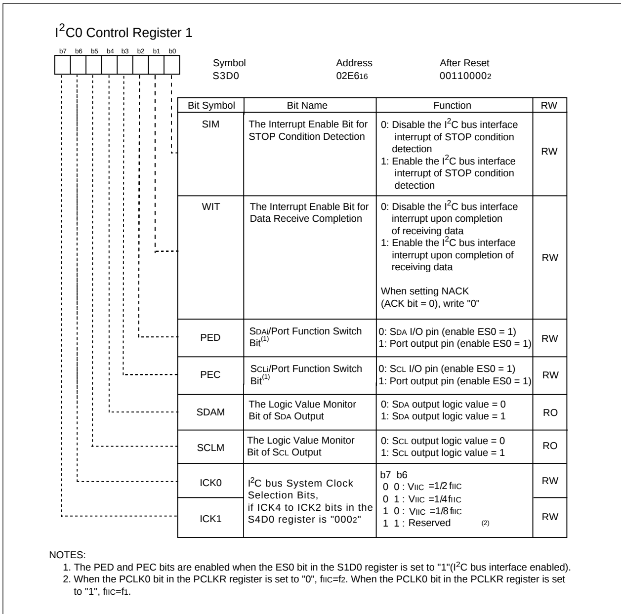
Figure 16.6 S3D0 Register
