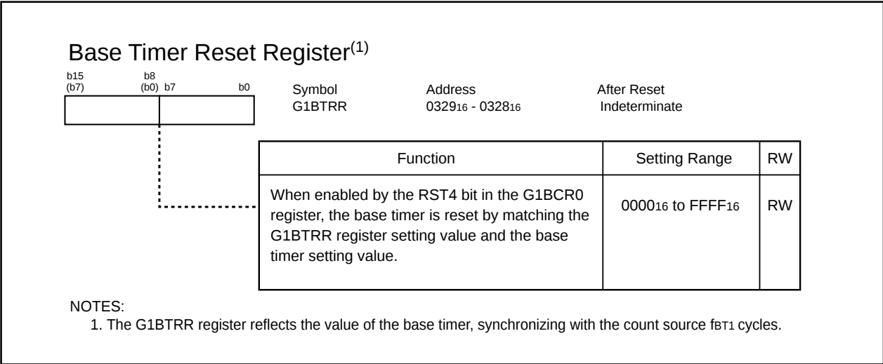
Figure 13.4 G1BTRR Register
