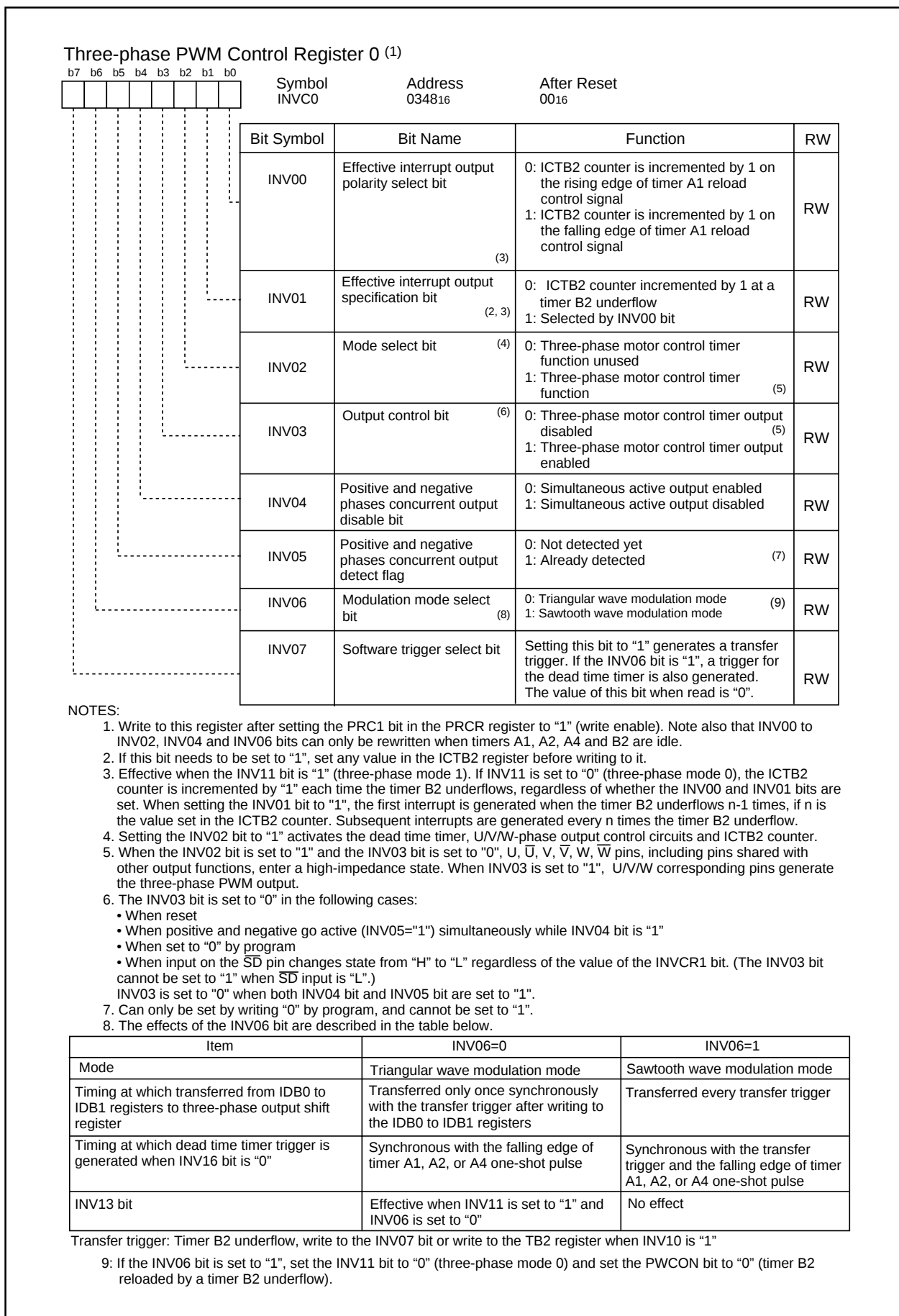
Figure 12.26 INV0 Register
