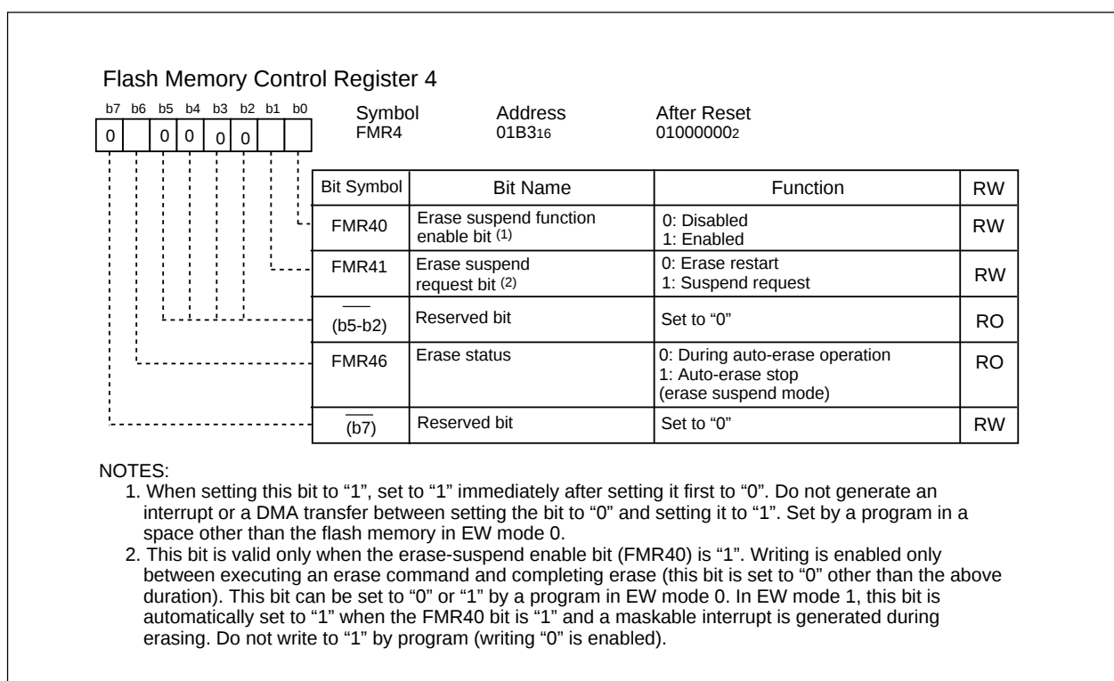
Figure 18.8 FMR4 Register
