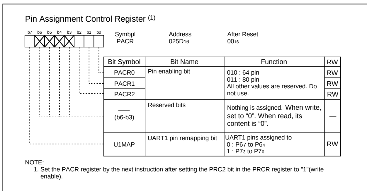
Figure 17.10 PACR Register
