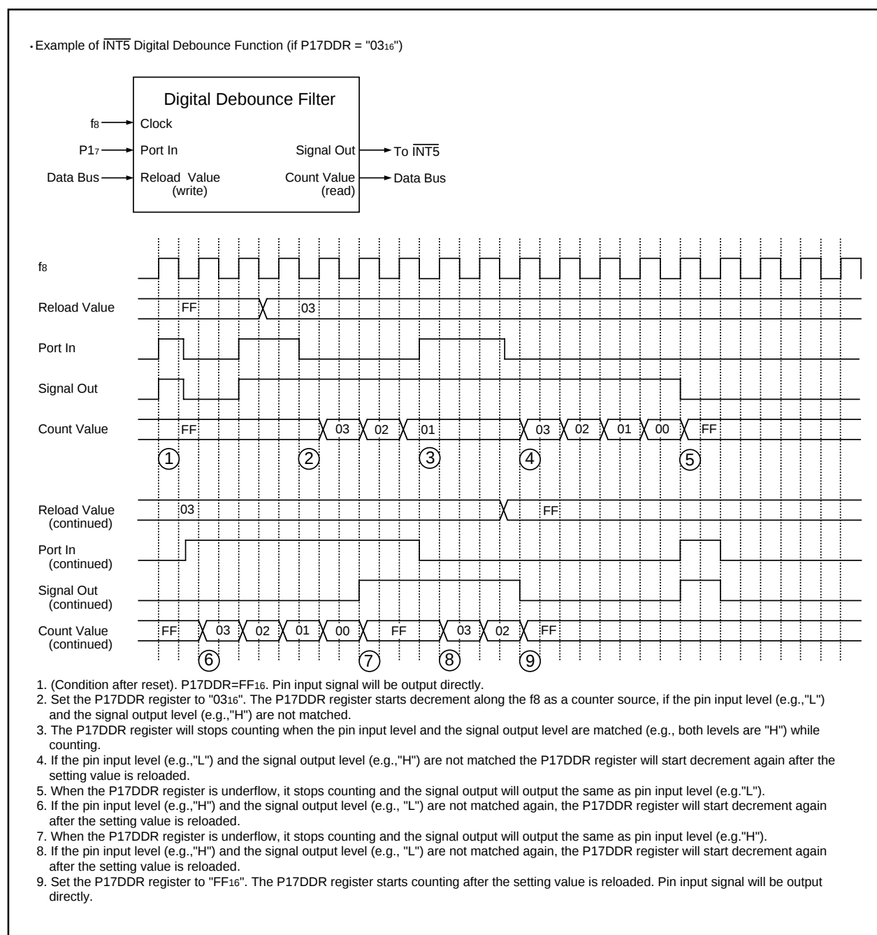
Figure 17.12 Digital Debounce Filter
