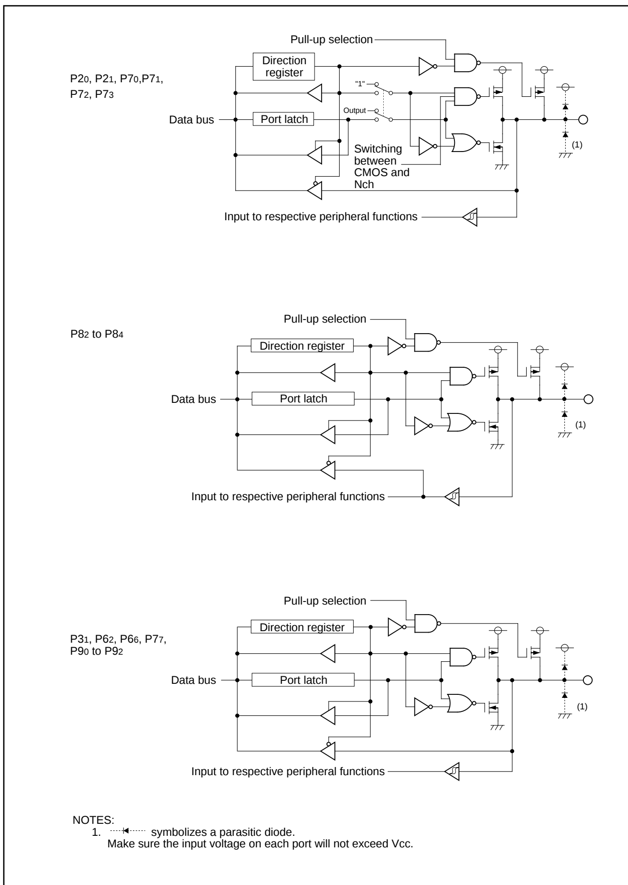
Figure 17.2 I/O Ports (2)
