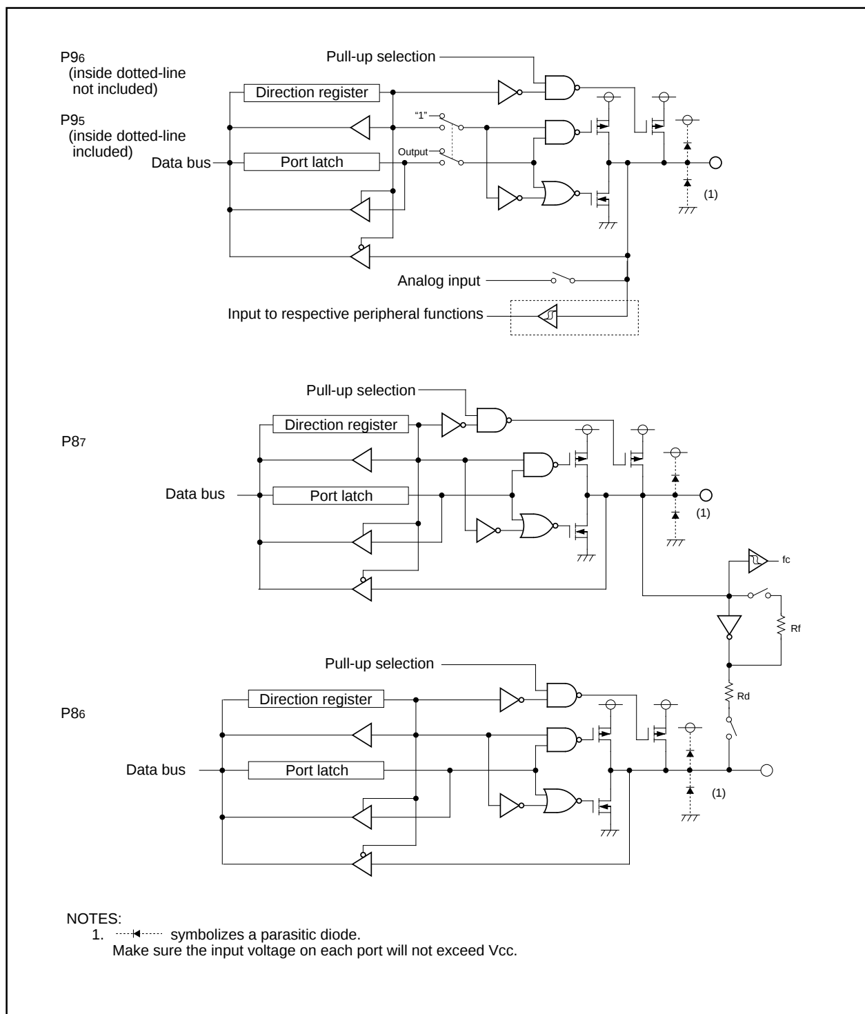
Figure 17.4 I/O Ports (4)
