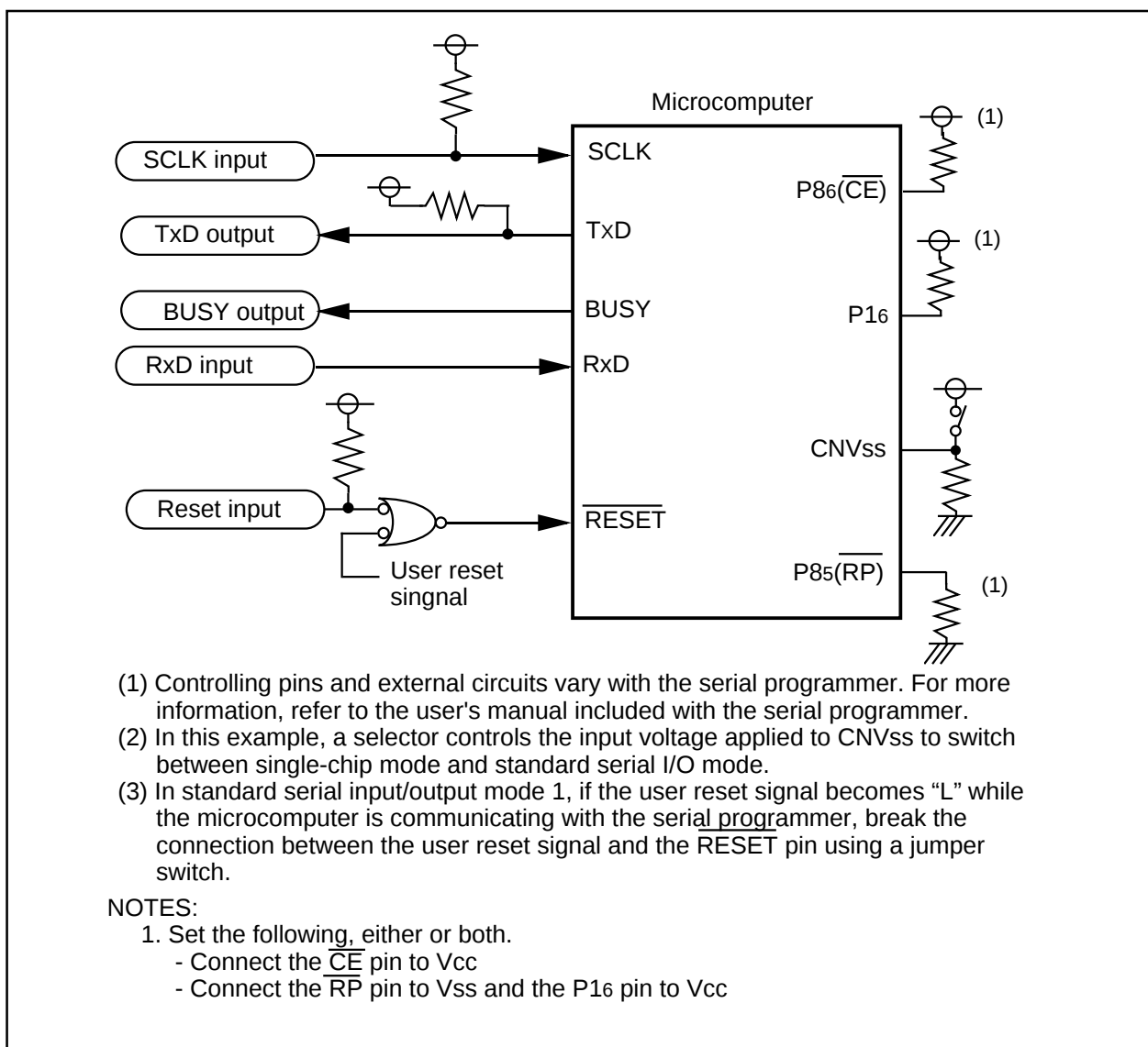
Figure 18.18 Circuit Application in Standard Serial I/O Mode 1
