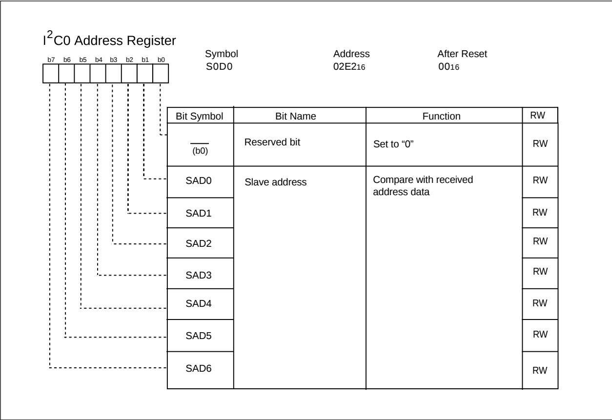
Figure 16.2 S0D0 Register
