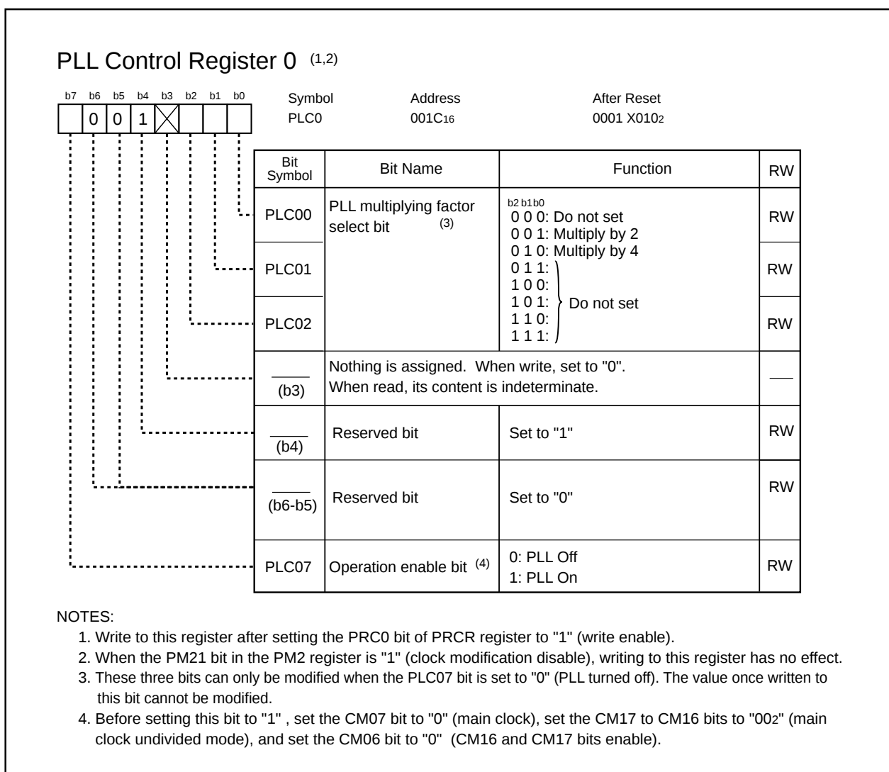
Figure 7.7 PLC0 Register
