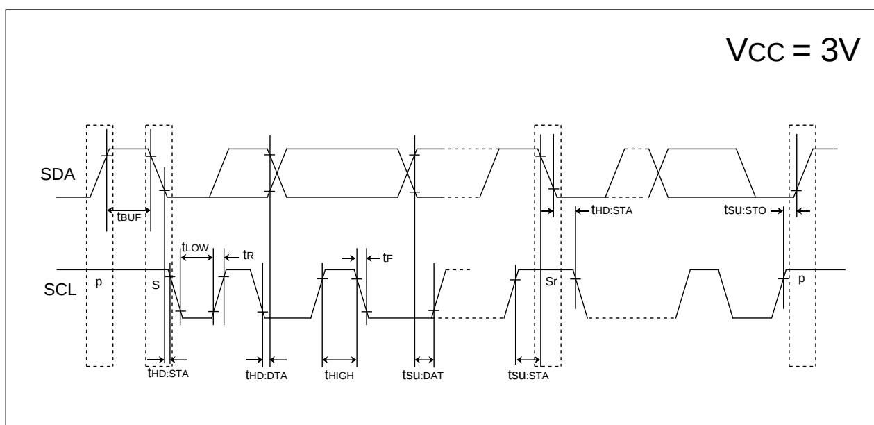
Figure 19.7 Timing Diagram (3)
