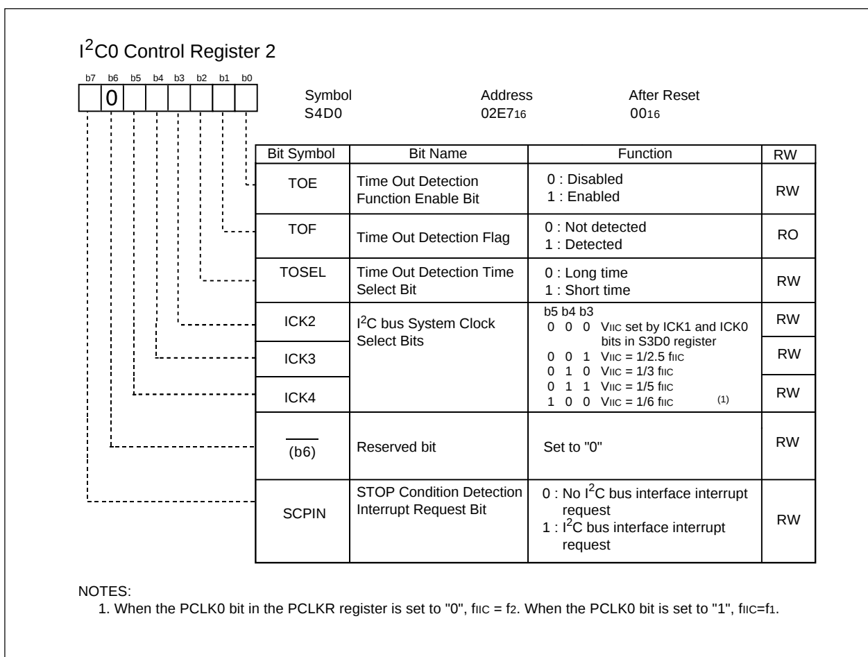
Figure 16.7 S4D0 Register
