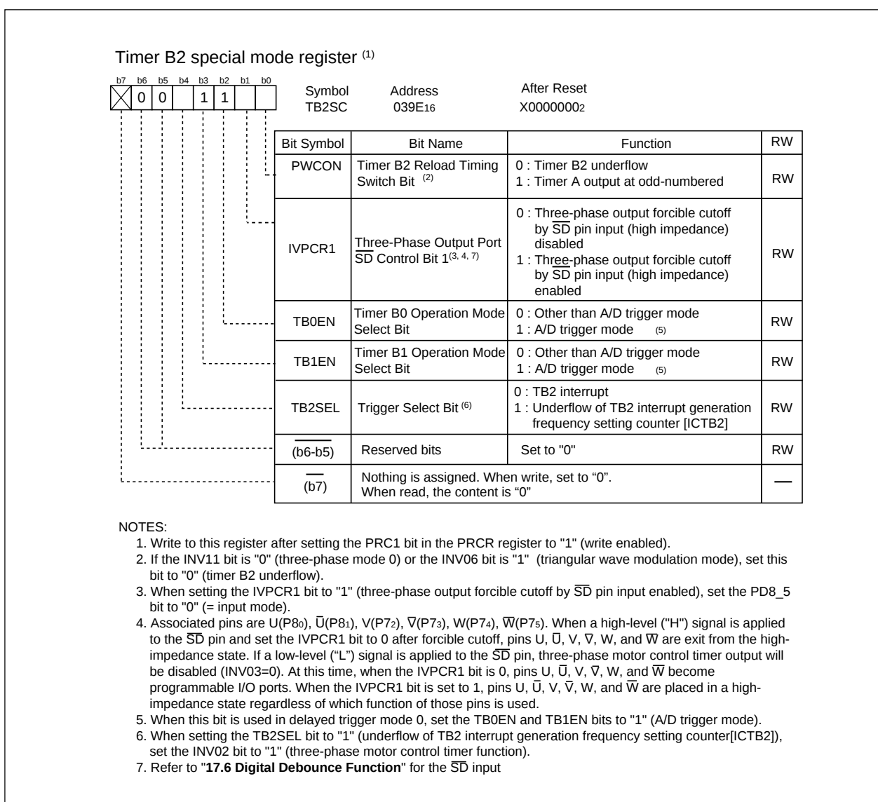
Figure 12.24 TB2SC Register in A/D Trigger Mode
