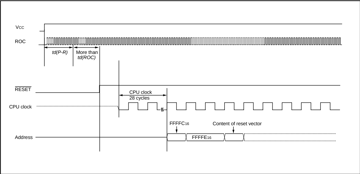
Figure 5.2 Reset Sequence
