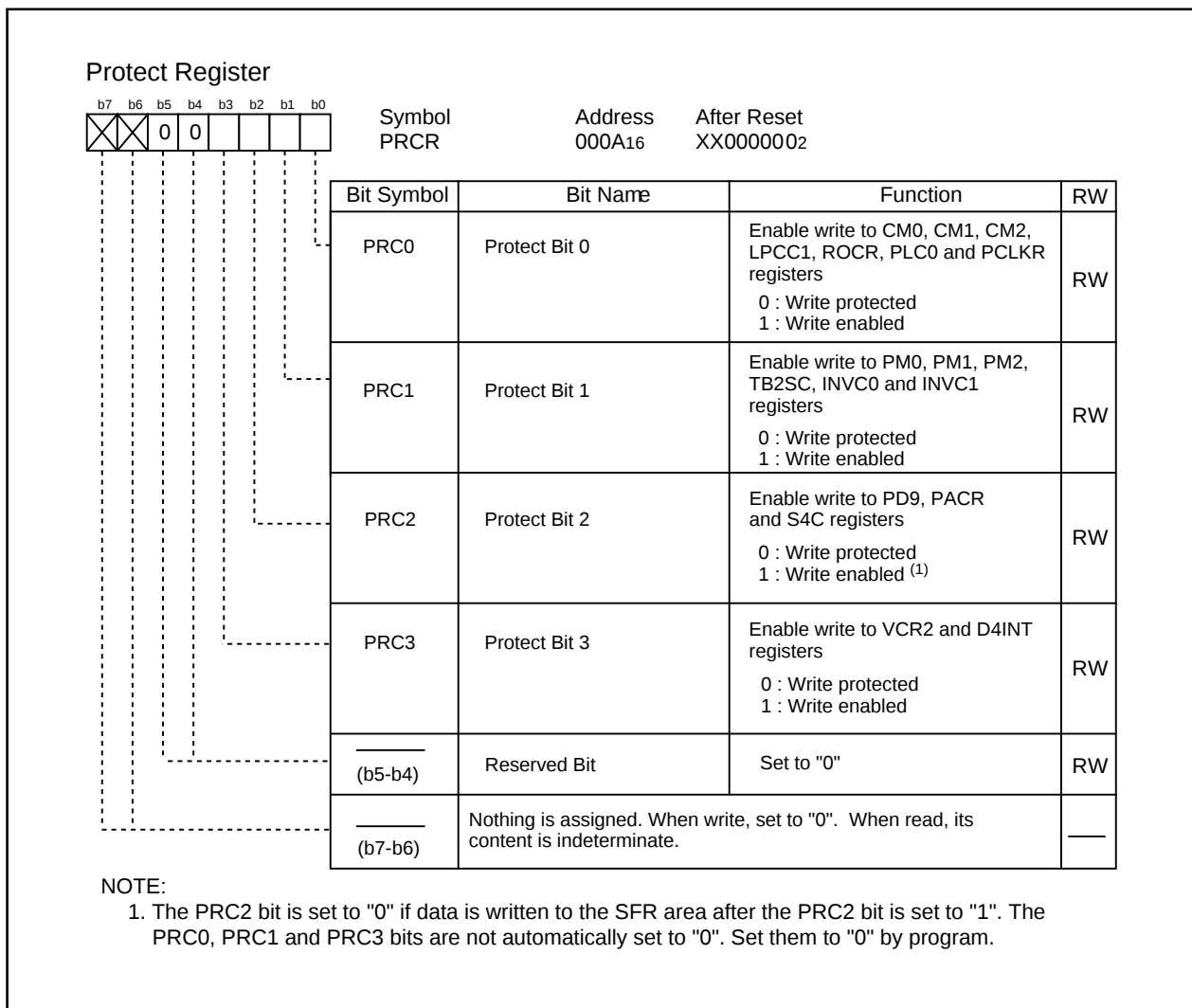
Figure 8.1 PRCR Register
