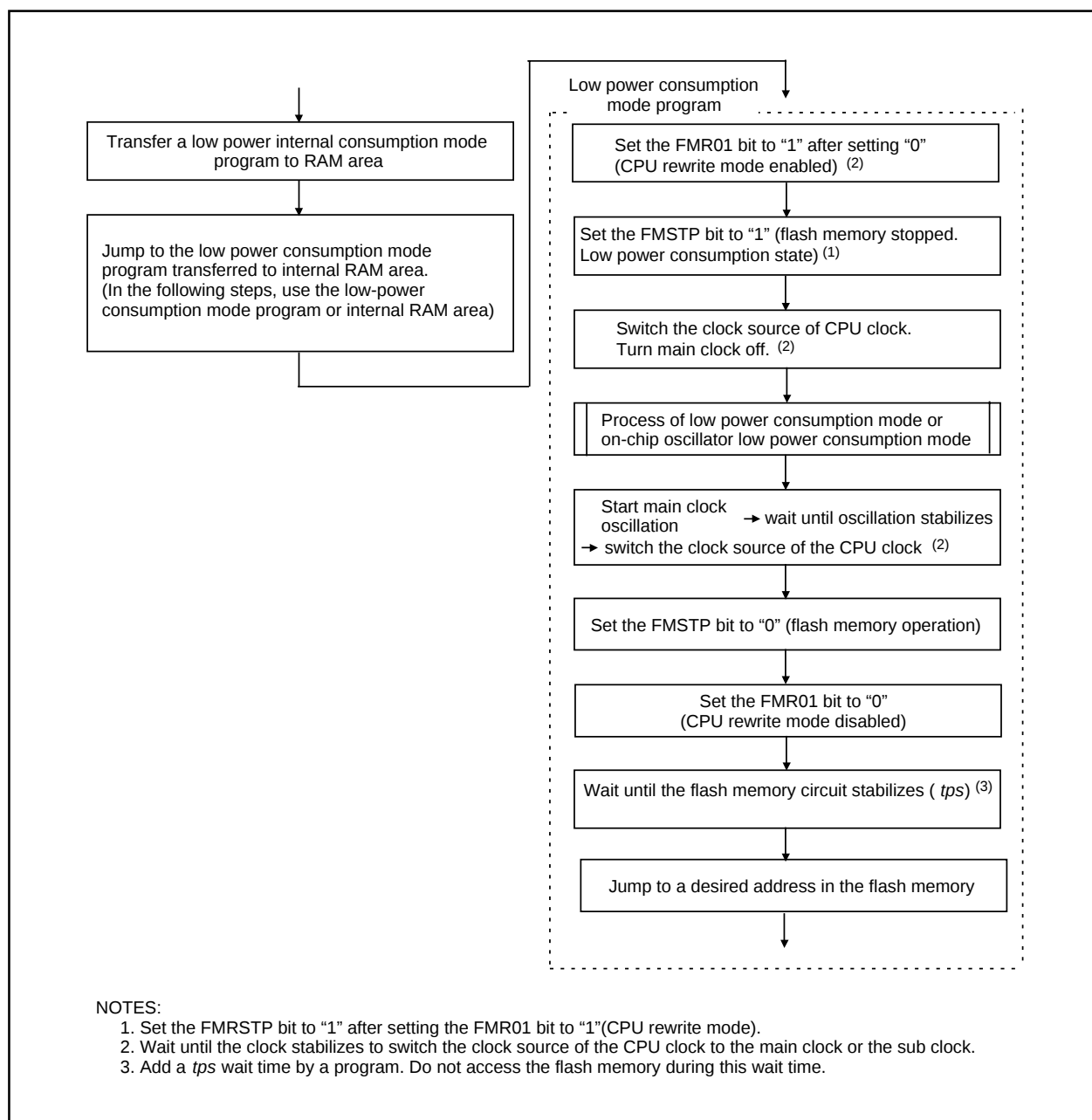
Figure 18.11 Processing Before and After Low Power Dissipation Mode
