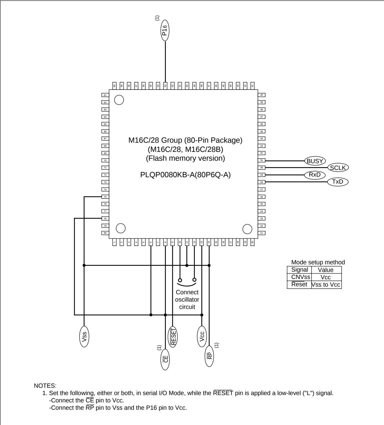
Figure 18.17 Pin Connections for Serial I/O Mode (2)
