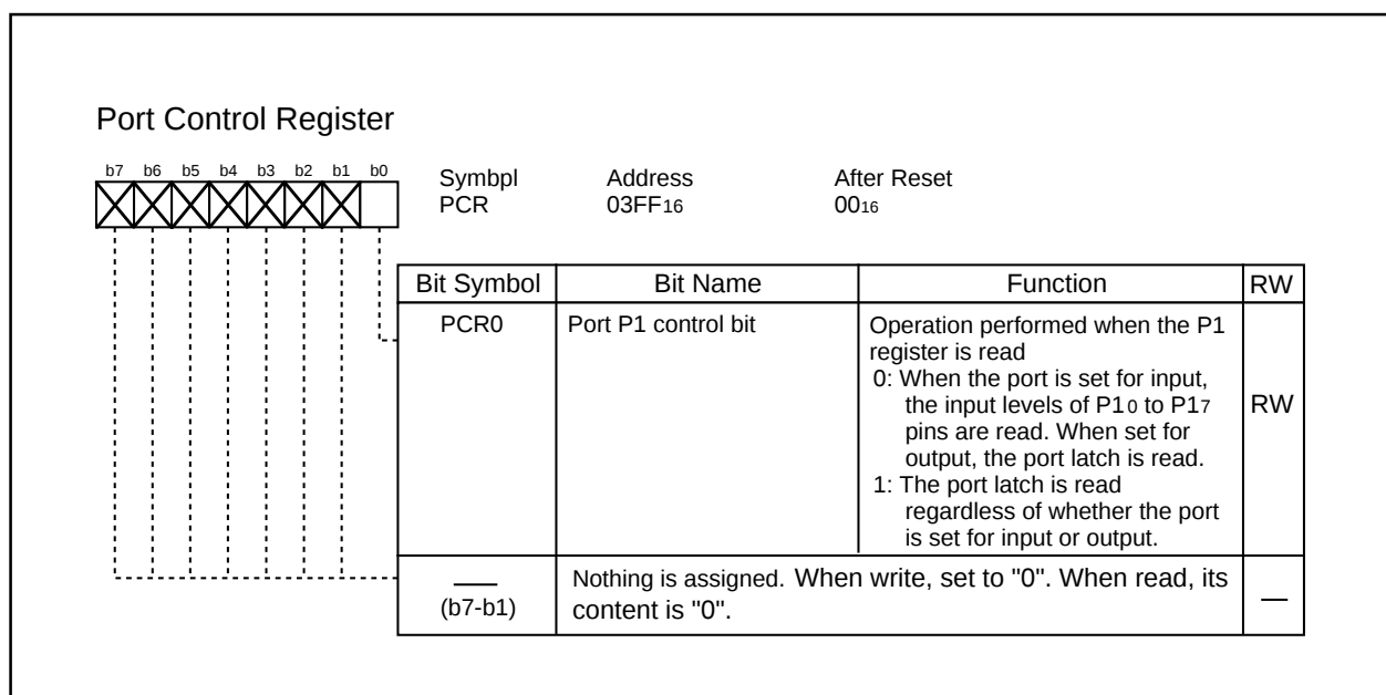
Figure 17.9 PCR Register
