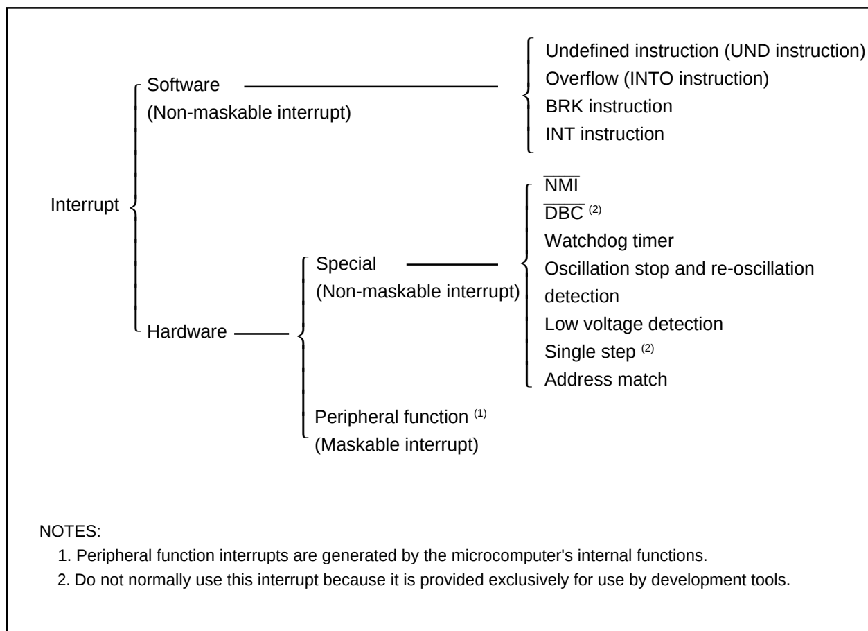
Figure 9.1 Interrupts
