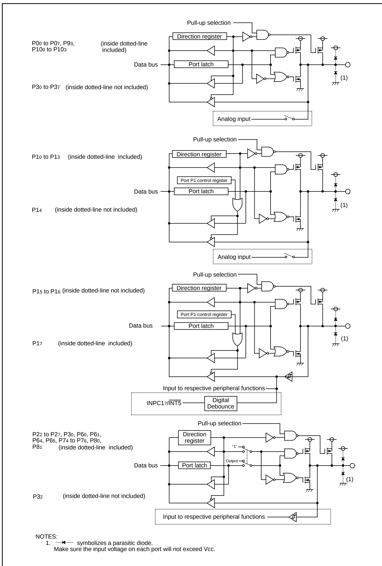
Figure 17.1 I/O Ports (1)
