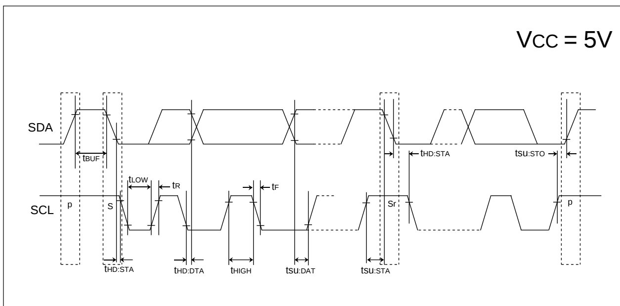
Figure 19.4 Timing Diagram (3)
