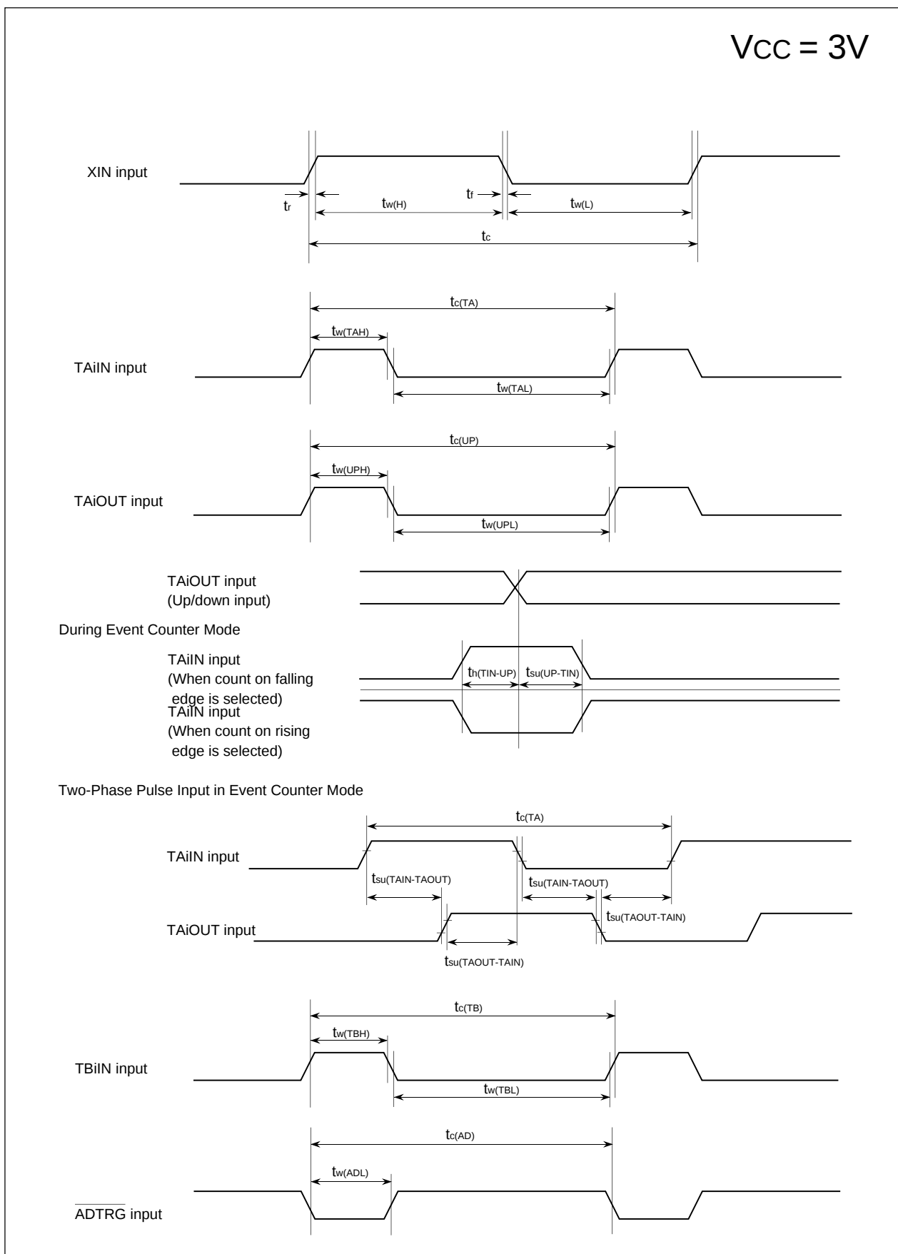
Figure 19.5 Timing Diagram (1)
