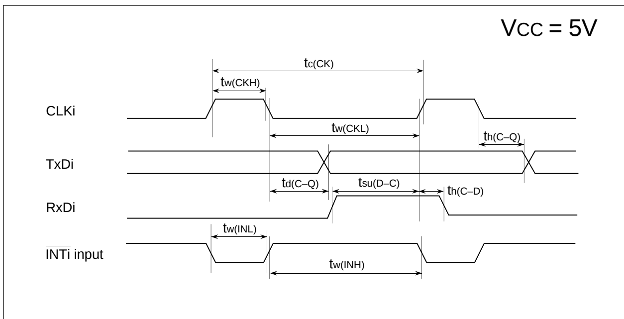
Figure 19.3. Timing Diagram (2)
