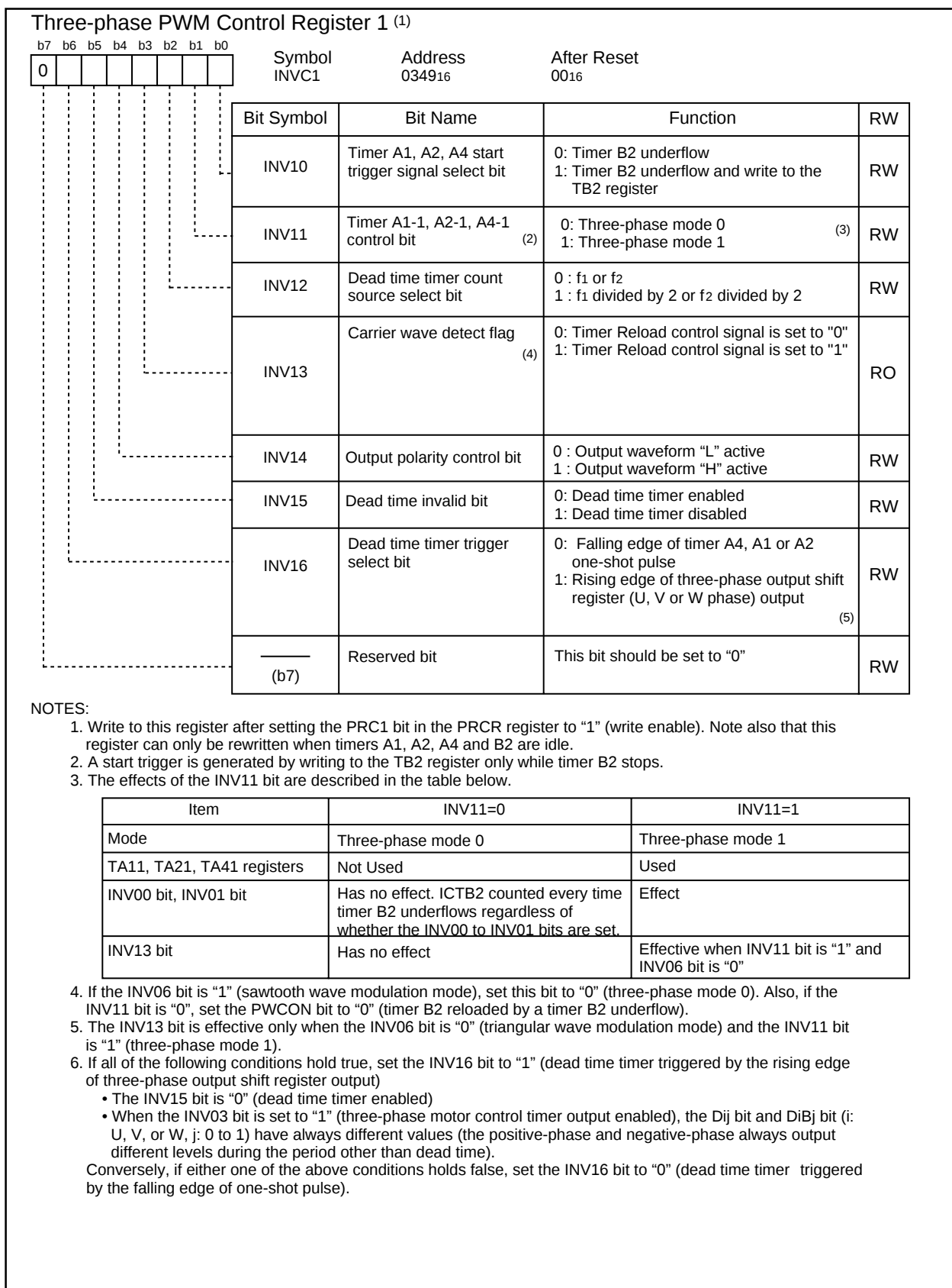
Figure 12.27 INVC1 Register
