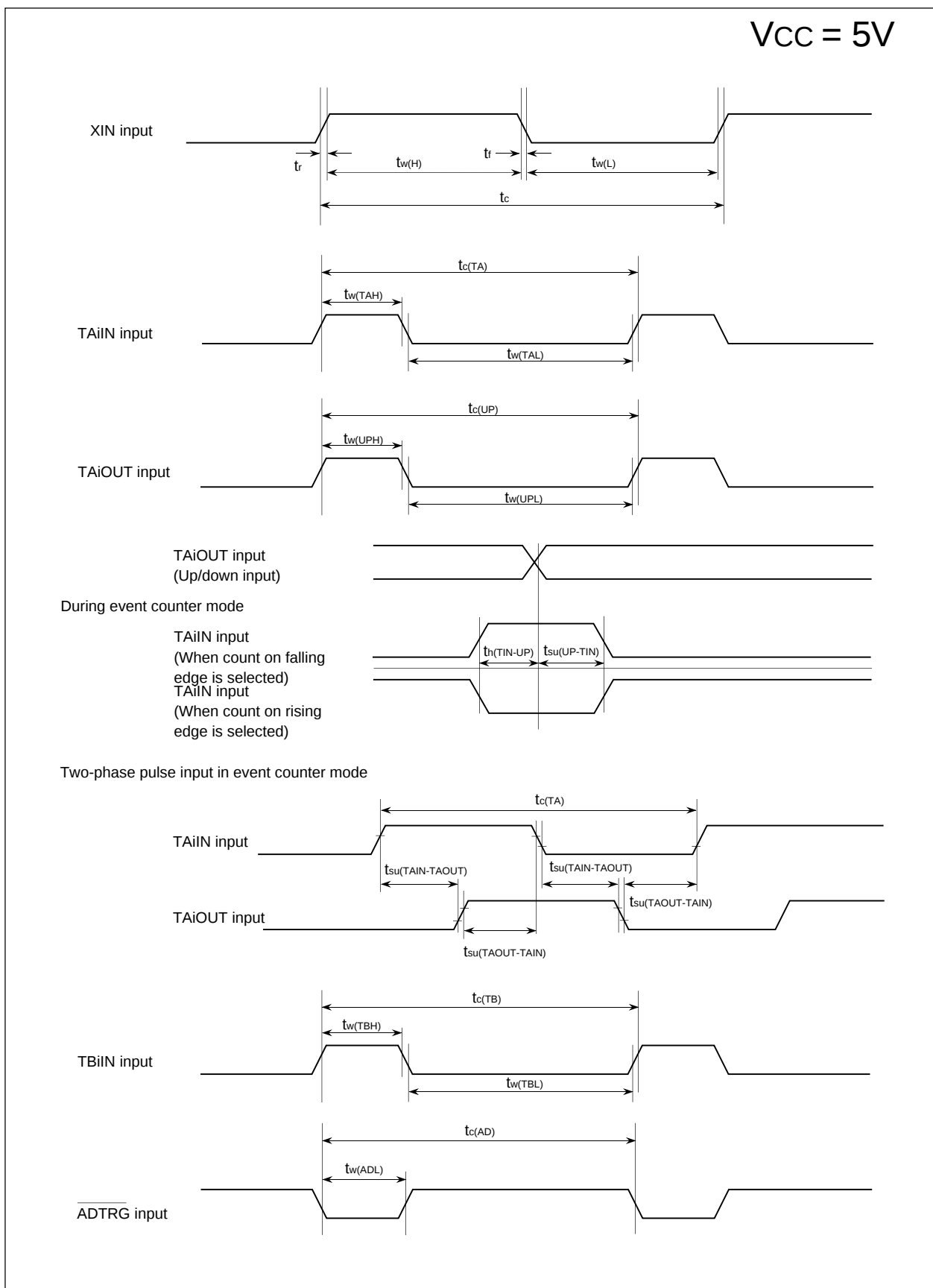
Figure 19.2 Timing Diagram (1)
