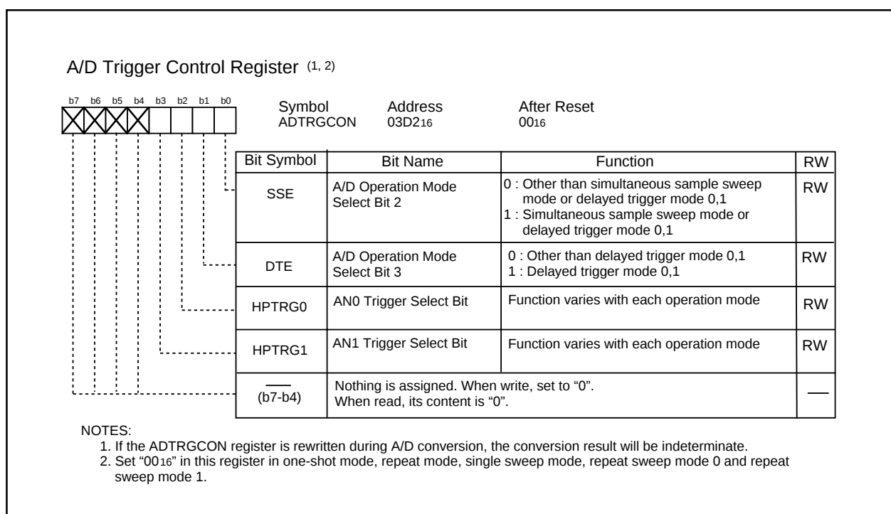
Figure 15.3 ADTRGCON Register
