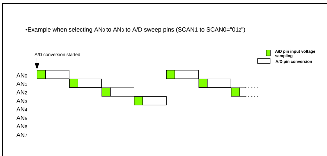
Figure 15.12 Operation Example in Repeat Sweep Mode 0
