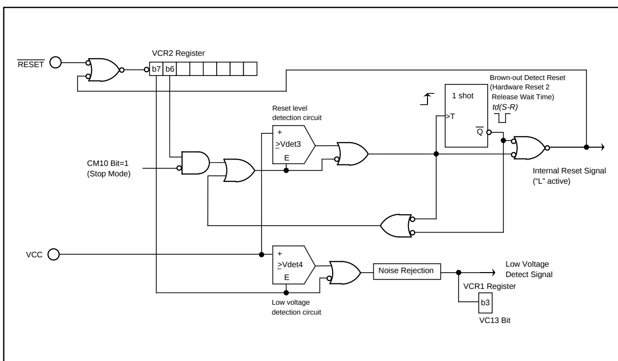
Figure 5.4 Low Voltage Detection Circuit Block
