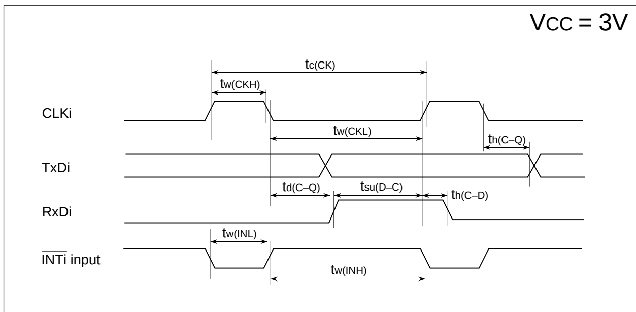
Figure 19.6 Timing Diagram (2)
