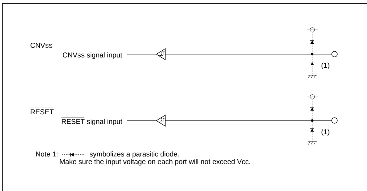
Figure 17.5 I/O Pins
