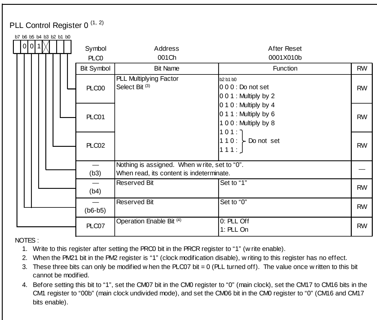
Figure 10.6 PLC0 Register
