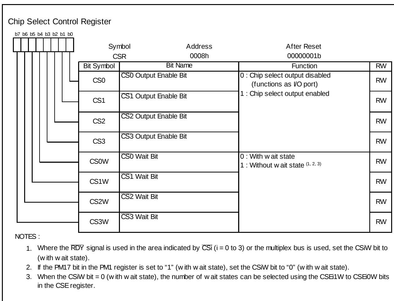
Figure 8.1 CSR Register
