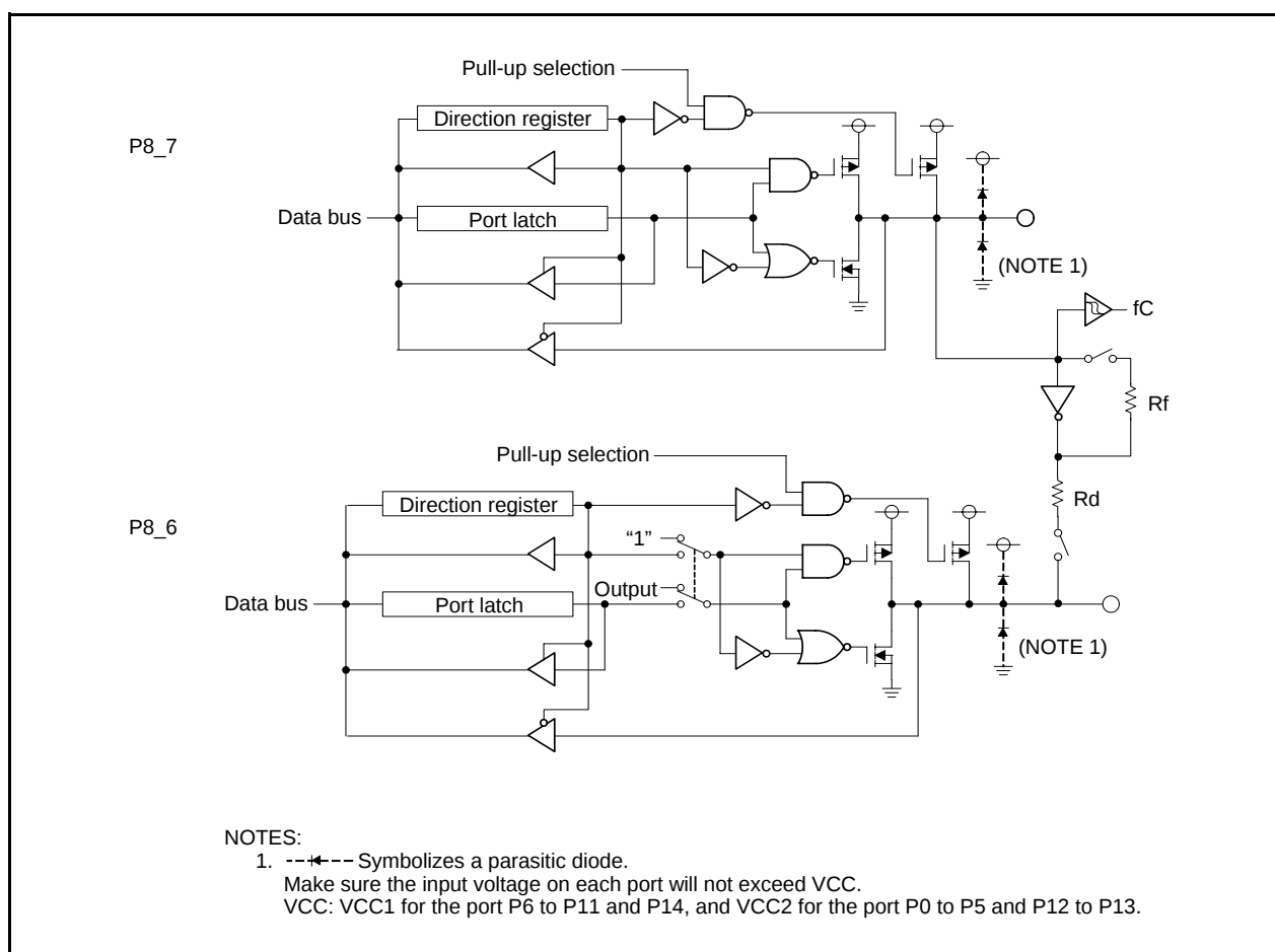
Figure 21.5 I/O Ports (5)
