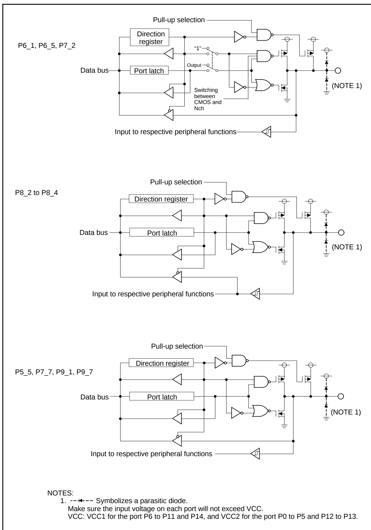
Figure 21.2 I/O Ports (2)
