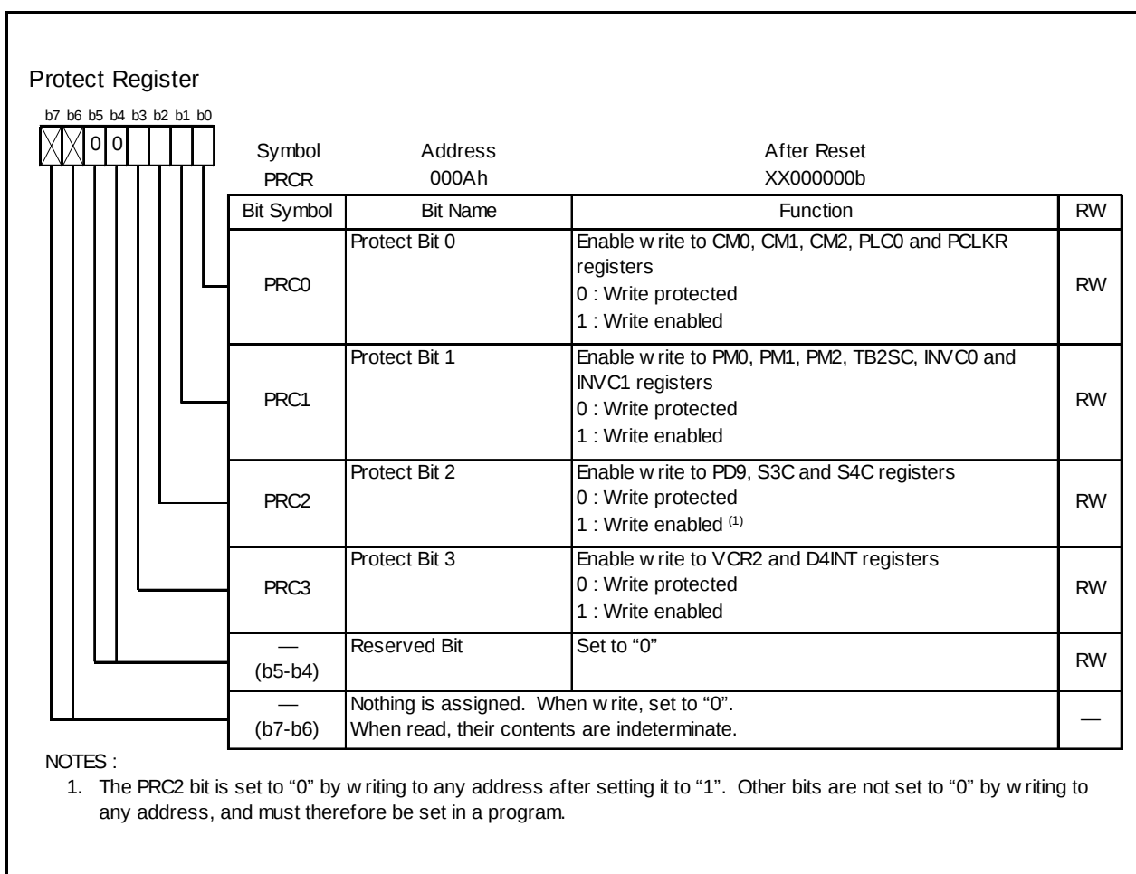
Figure 11.1 PRCR Register
