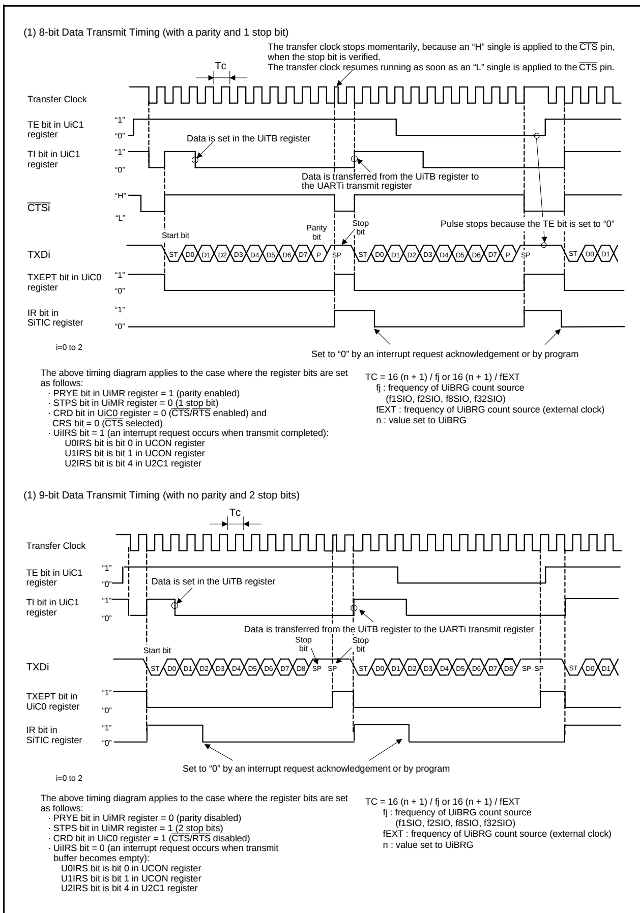
Figure 17.19 Transmit Operation
