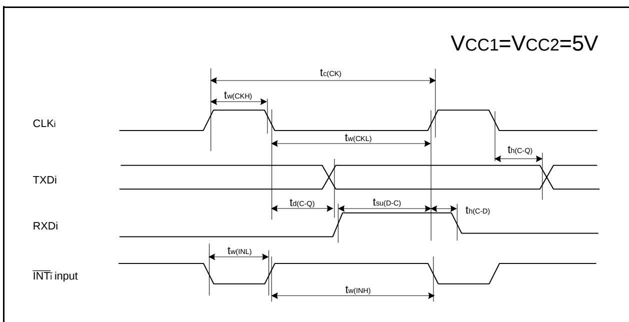
Figure 23.25 Timing Diagram (2)
