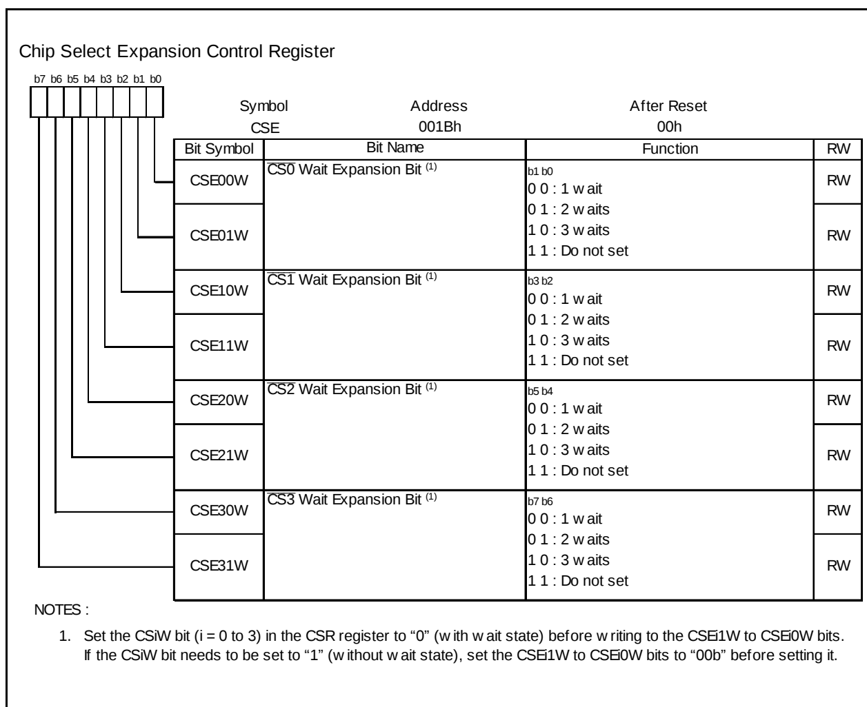
Figure 8.6 CSE Register
