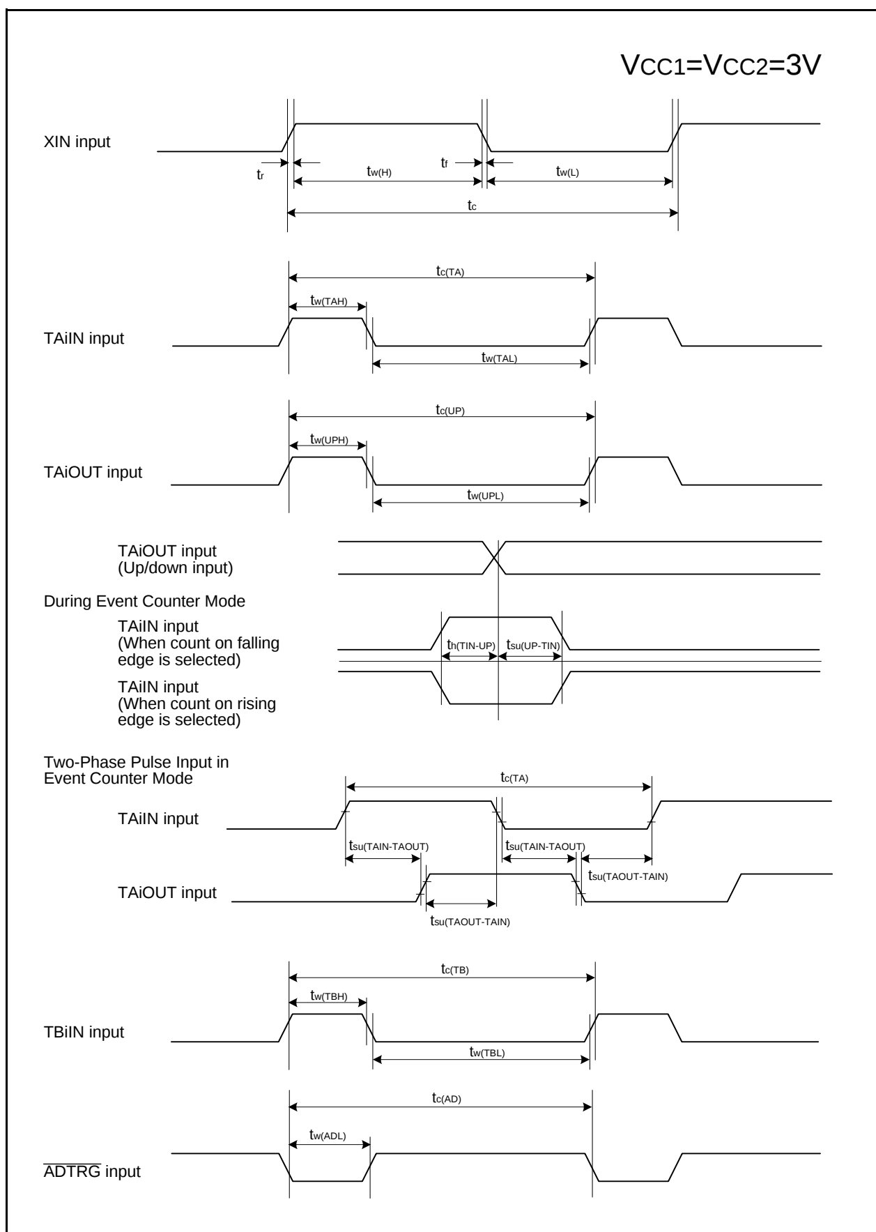
Figure 23.13 Timing Diagram (1)
