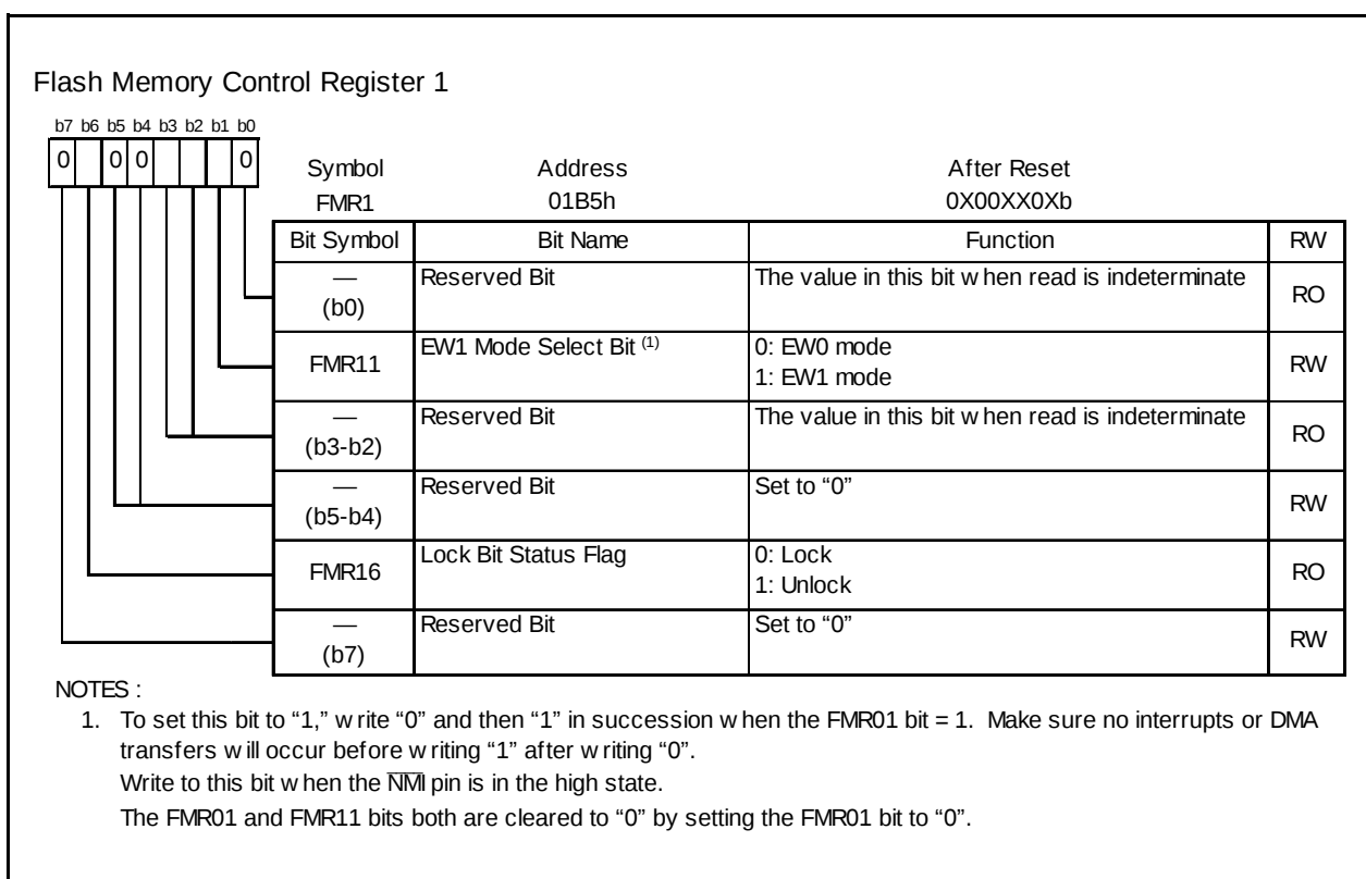
Figure 22.6 FMR1 Register
