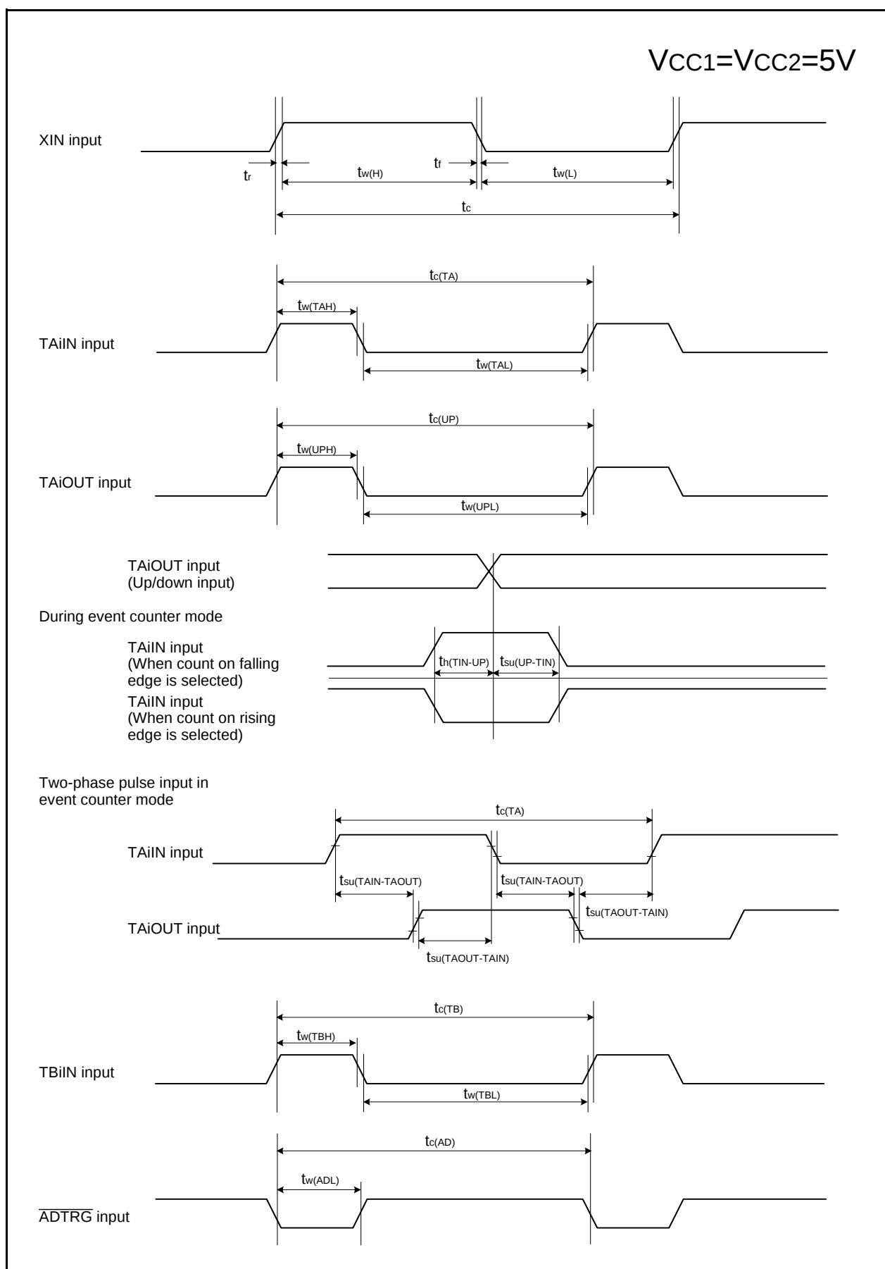
Figure 23.24 Timing Diagram (1)
