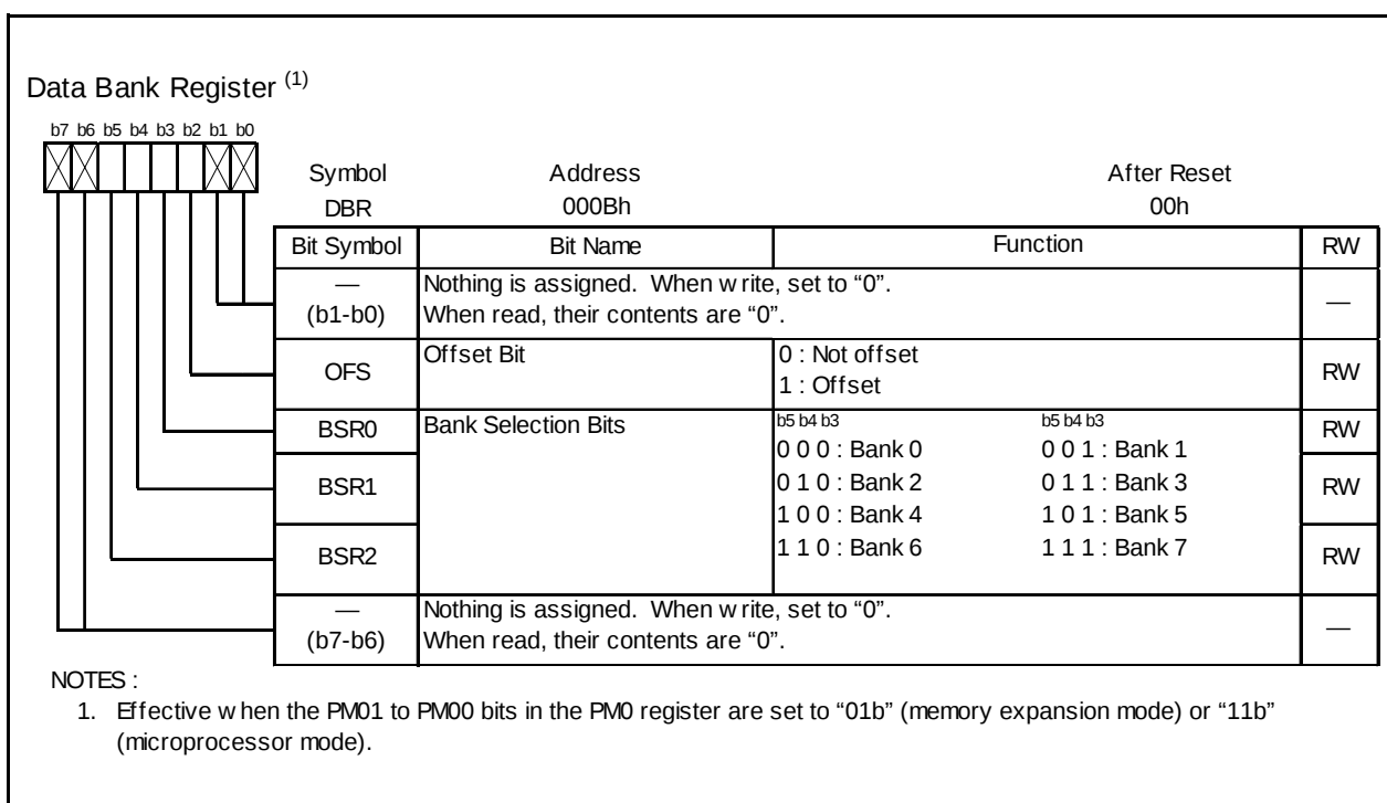
Figure 9.1 DBR Register
