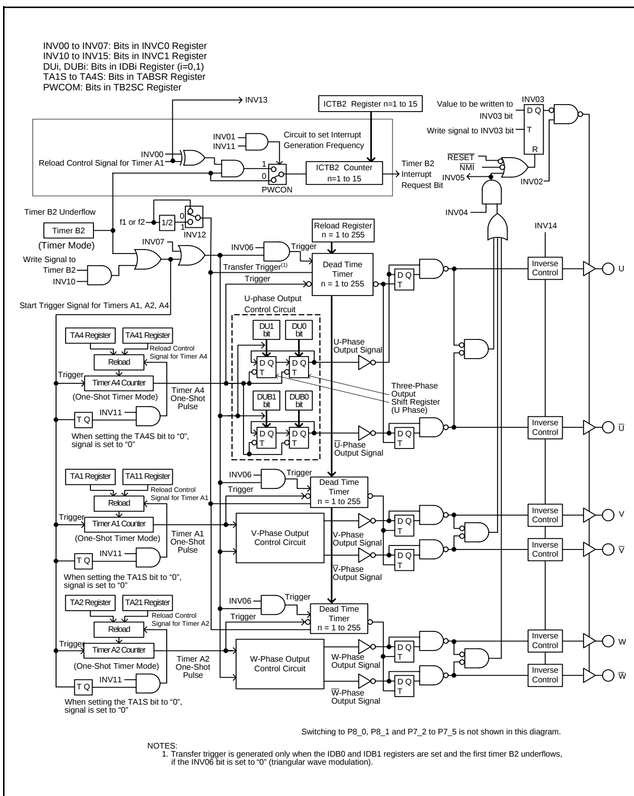
Figure 16.1 Three-phase Motor Control Timer Functions Block Diagram
