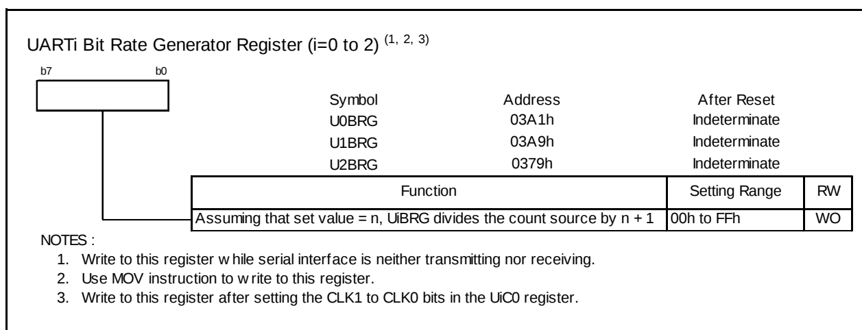
Figure 17.6 UiBRG Register
