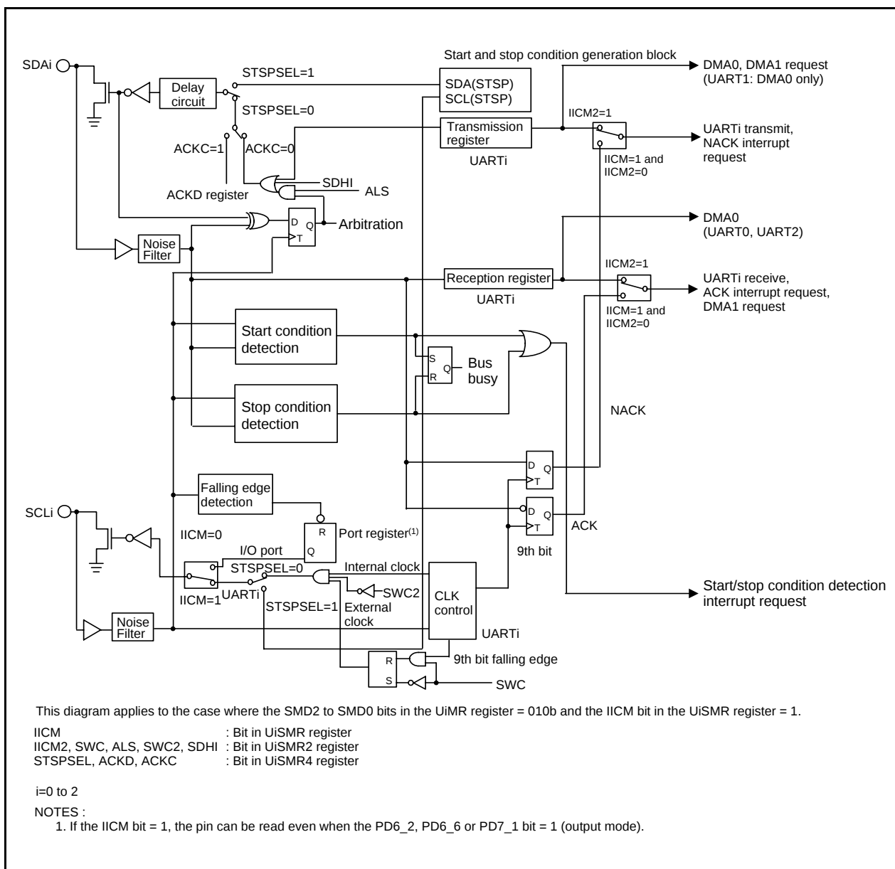
Figure 17.25 I²C Mode Block Diagram
