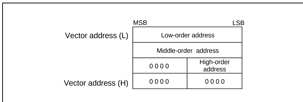
Figure 12.2 Interrupt Vector
