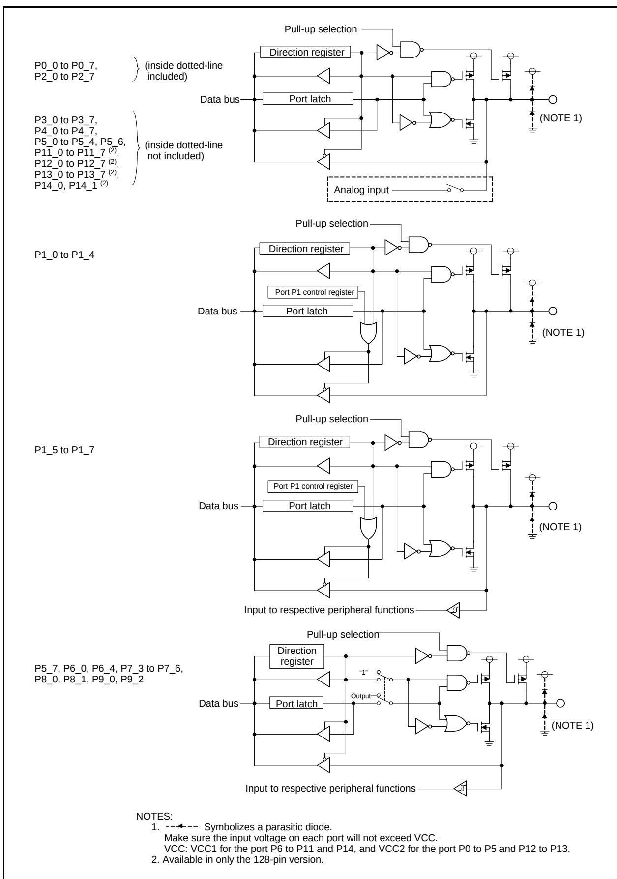
Figure 21.1 I/O Ports (1)
