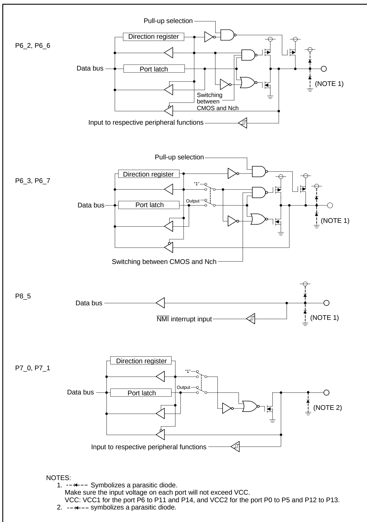
Figure 21.3 I/O Ports (3)
