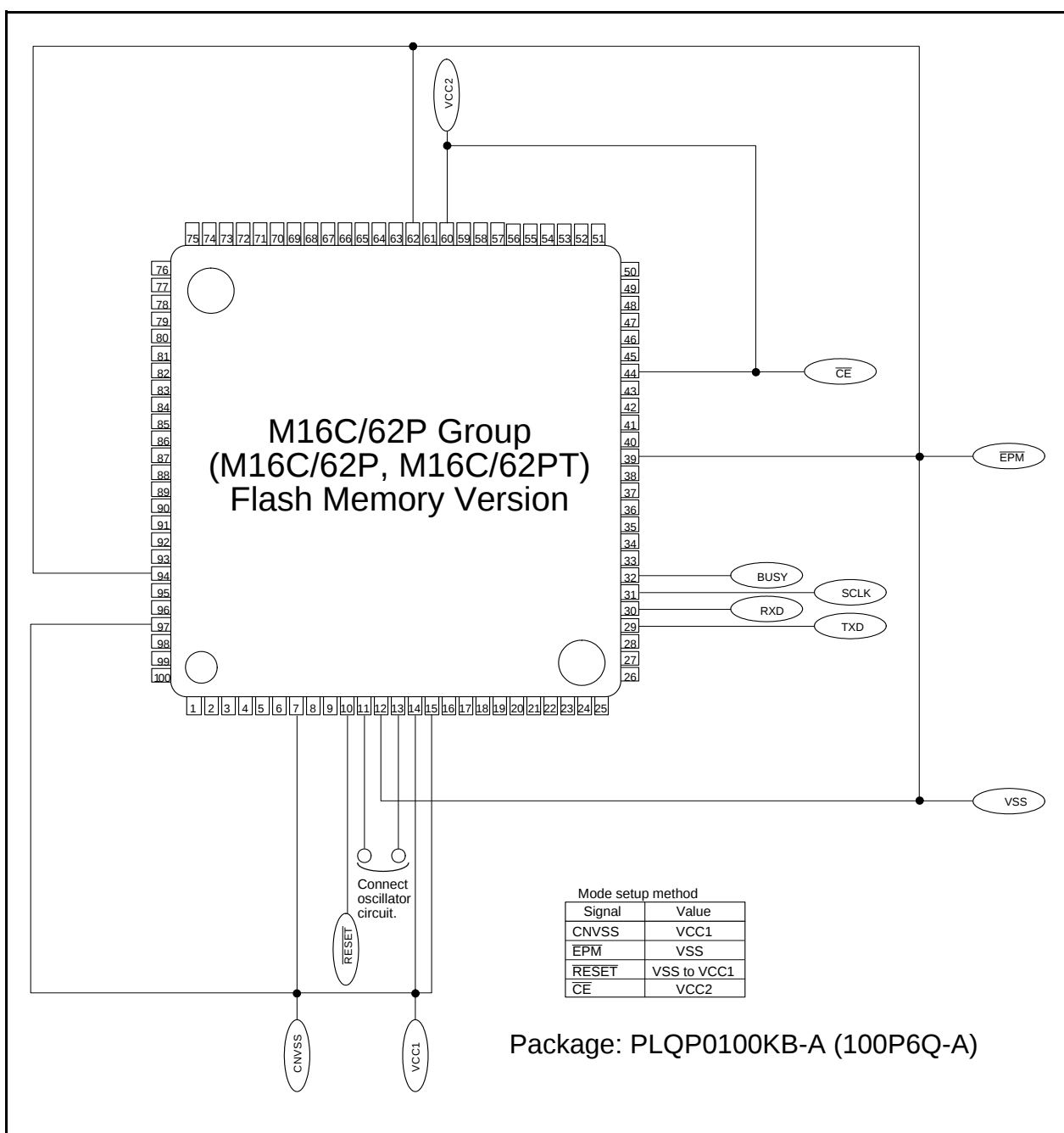
Figure 22.17 Pin Connections for Serial I/O Mode (3)
