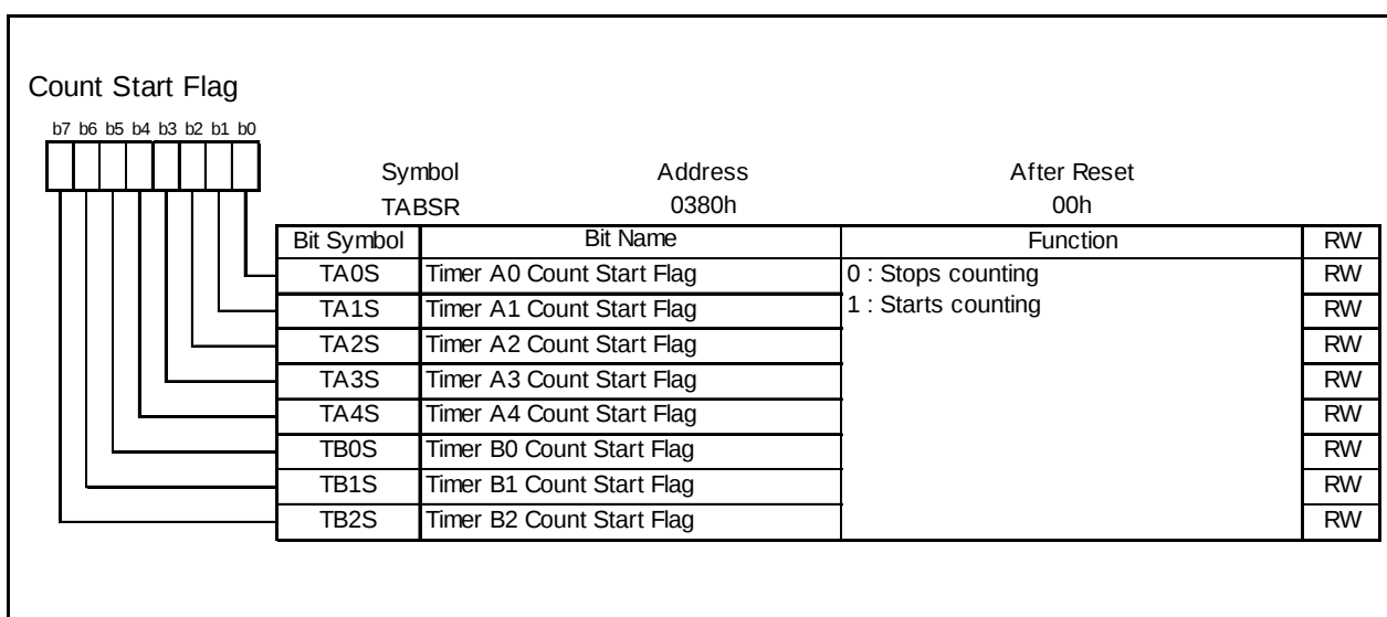
Figure 16.7 TABSR Register
