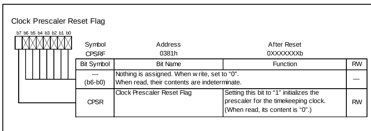
Figure 15.7 CPSRF Register
