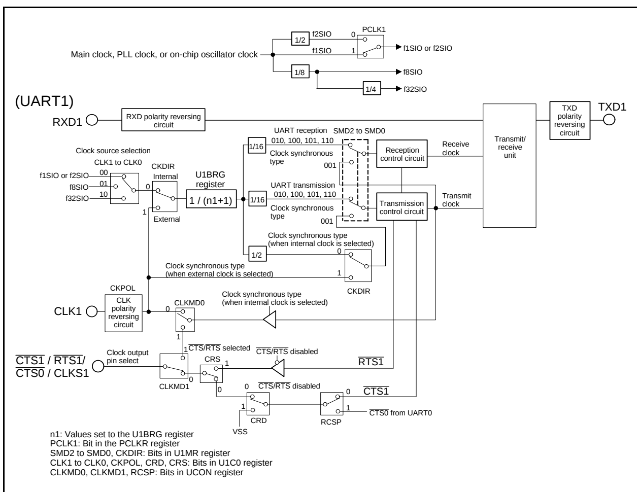
Figure 17.2 UART1 Block Diagram
