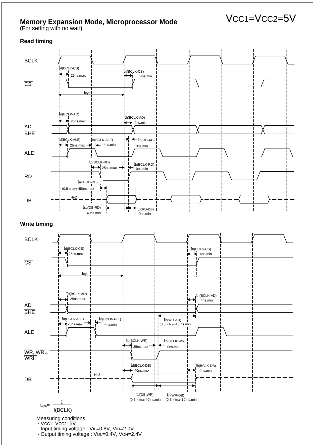
Figure 23.6 Timing Diagram (4)
