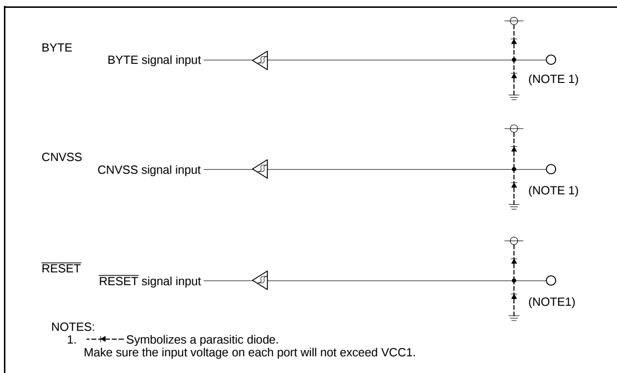
Figure 21.6 I/O Pins
