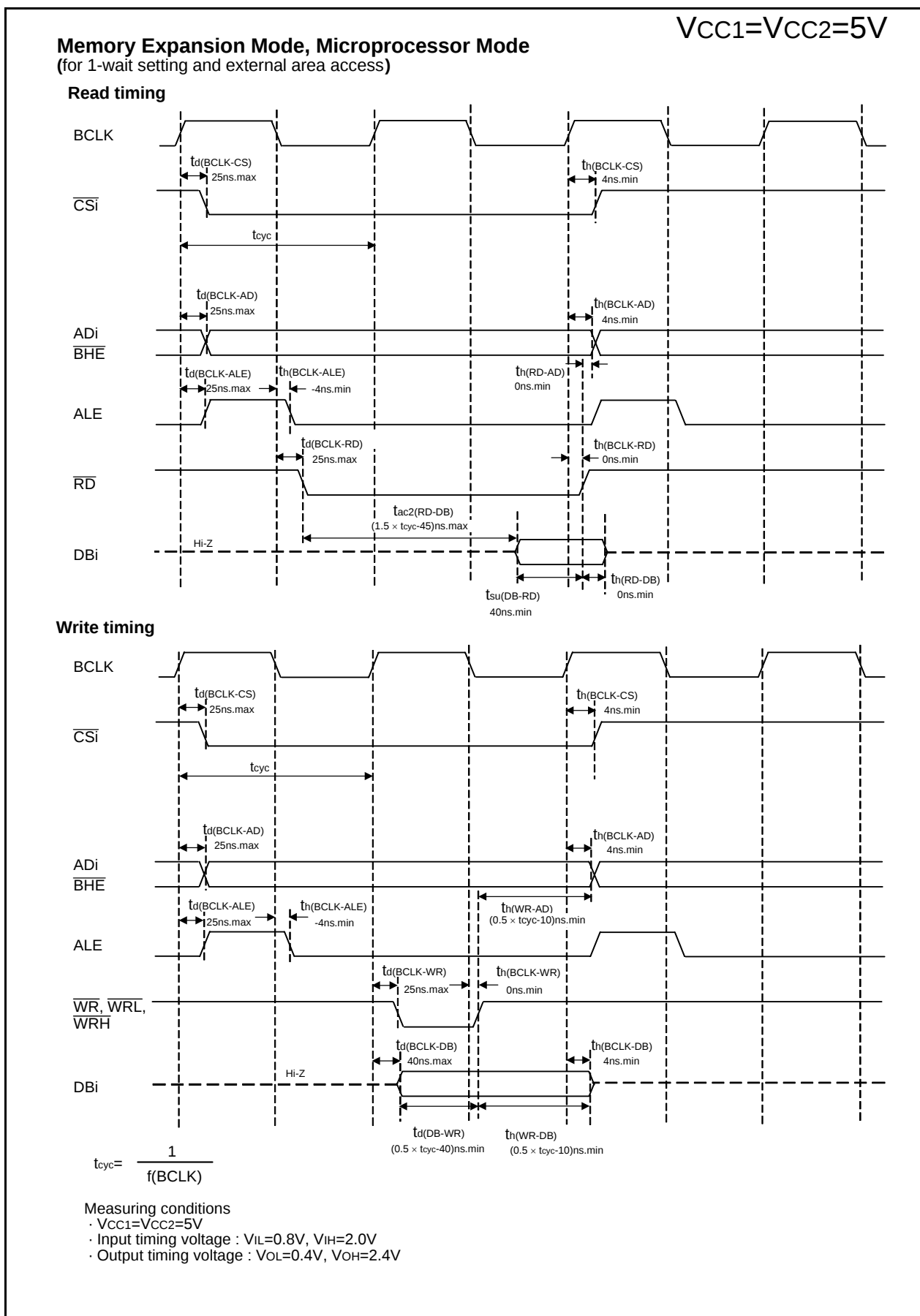
Figure 23.7 Timing Diagram (5)
