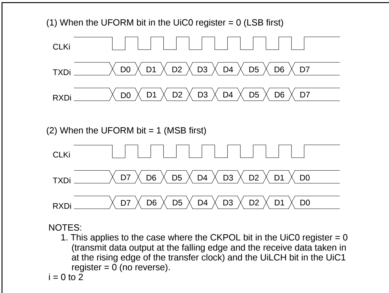
Figure 17.15 Transfer Format
